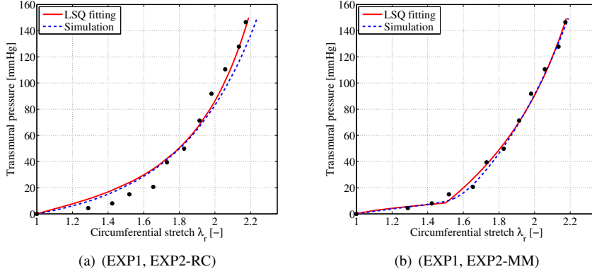
Figure 10: Strain-stress relation \mathcal{T}(\lambda_r) and corresponding relation obtained from the numerical simulations for the anisotropic models of Sec. 2.2.2. The dots represent the experimental data in (Scott et al., 1972).
