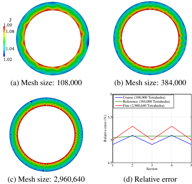
Figure 16: Volume ratio J for different meshes of the computational domain.
