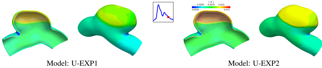
Figure 30: Vessel wall displacement in the aneurysm dome at the time t = 0.6 s. The gray overlay represents the undeformed geometry. The deformations are magnified by a factor 3
