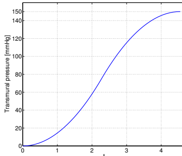
Figure 7: Inflating pseudo-time pressure profile p(t) for problem (3).
