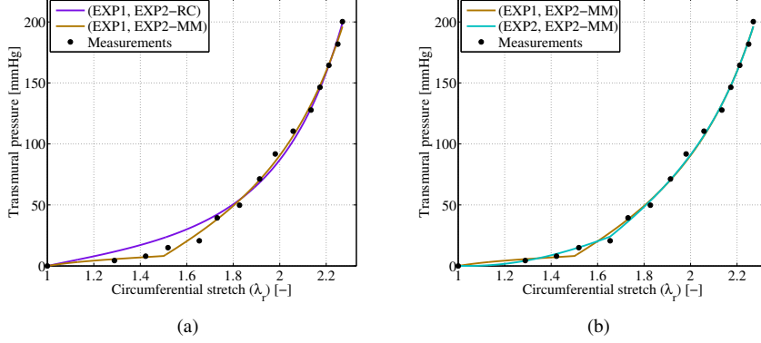
Figure 4: Least-squares approximation of the data in (Scott et al., 1972) using the anisotropic models.
