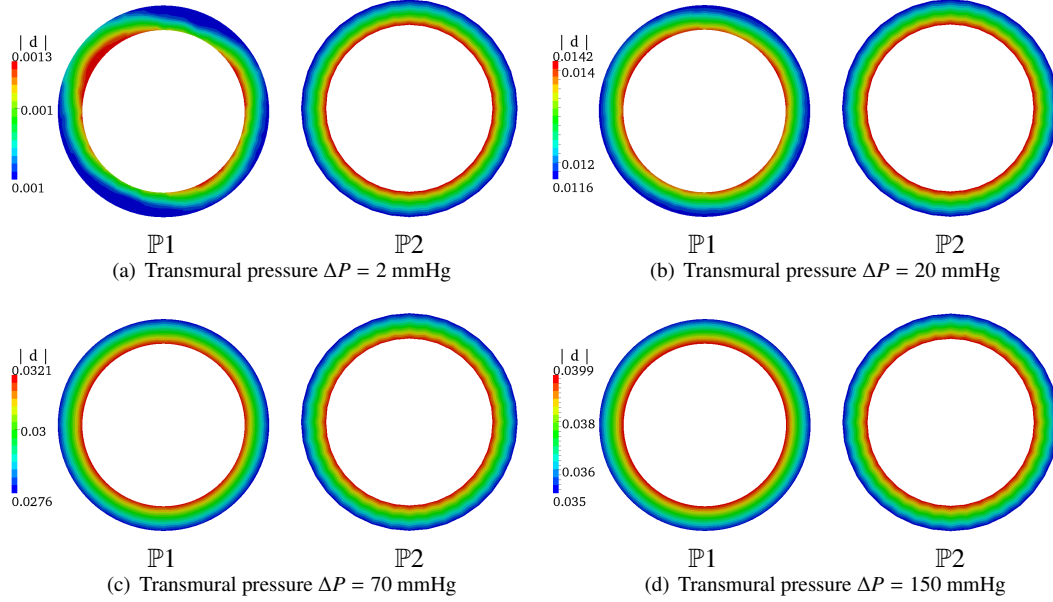
Figure 12: Displacement magnitude [cm] at different inflating pressures using the isotropic EXP1 model: using \mathbb{P}1 elements (#DOFs: 241, 200) (left columns); using \mathbb{P}2 elements (#DOFs: 234, 360) (right columns).
