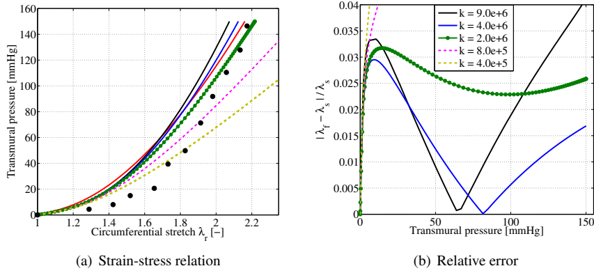
Figure 13: Strain-stress relations for different values of \kappa for the isotropic SVK model with the material parameters of Tab. 1.
