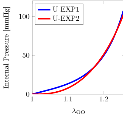
Figure 26: Stress-strain relations for the U-EXP1 and U-EXP2 models
