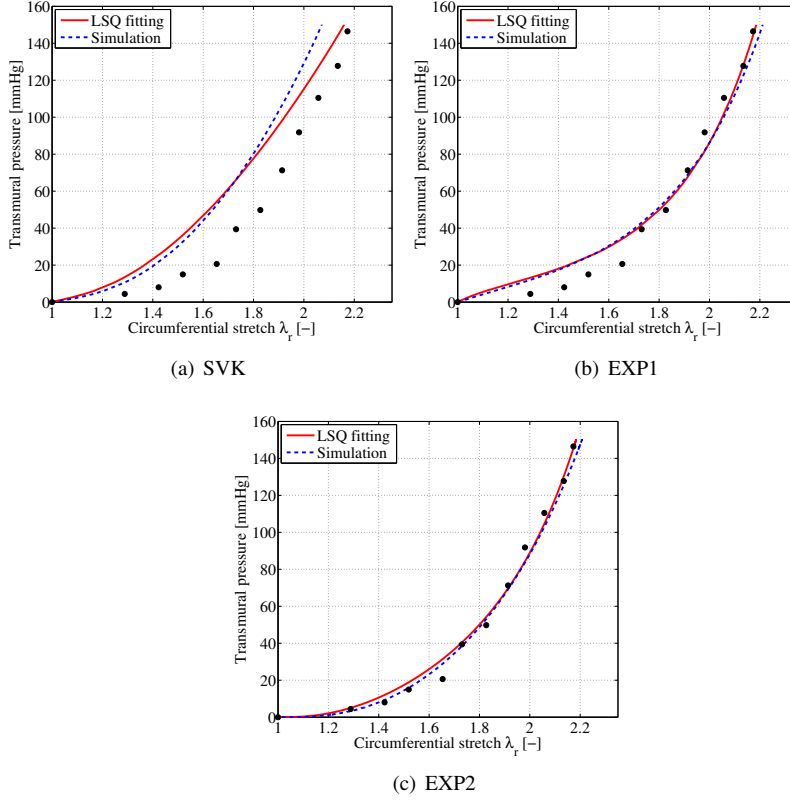
Figure 9: Strain-stress relation \mathcal{T}(\lambda_r) and corresponding relation obtained from the numerical simulations for the isotropic models of Sec. 2.2.2. The dots represent the experimental data in (Scott et al., 1972).
