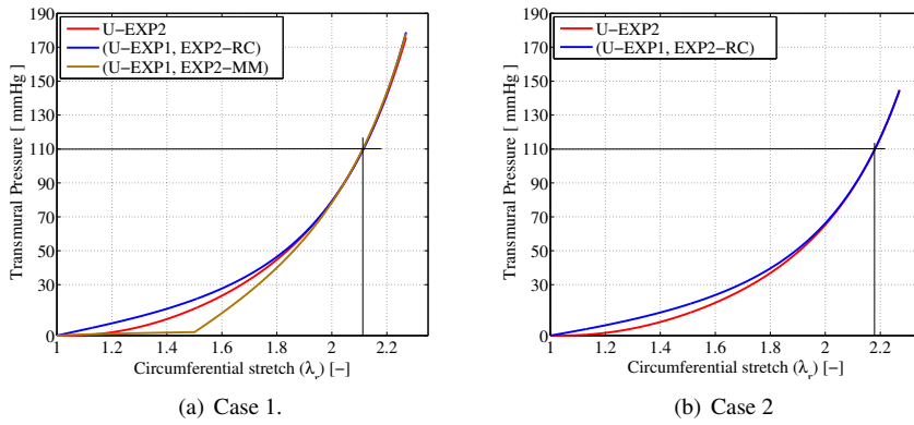
Figure 6: Functions \mathcal{T}(\lambda_r) with the weakening parameters of Tab. 3.
