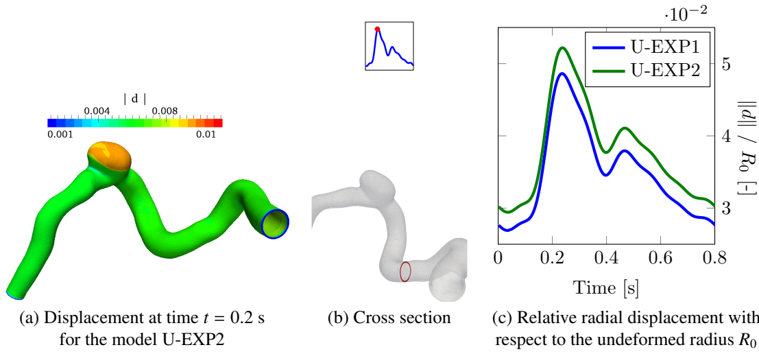
Figure 28: Vessel wall displacement: (a) snapshot at time t = 0.2 s; (b) location of the cross section for the evaluation of the relative vessel wall displacement; (c) relative parent vessel displacement on the internal surface with respect to the internal radius R_0 . Blood flow is right to left.
