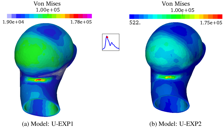
Figure 32: Von Mises stress in the aneurysm dome at the time t = 0.239 s
