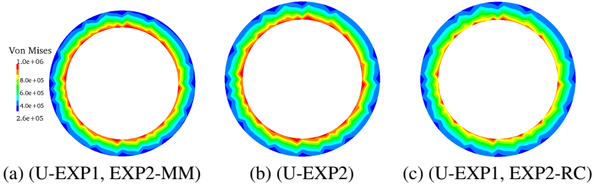
Figure 23: Case 1: Von Mises stress [dyn/cm 2 ] on the undeformed cross section at z = 1 cm and \Delta P = 110 mmHg.
