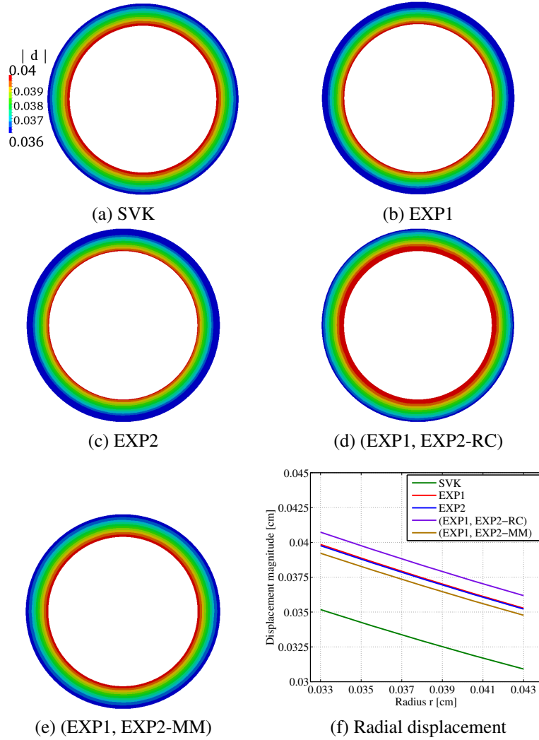
Figure 8: Displacement magnitude [cm] at the cross section at z = 1 cm and \Delta P = 150 mmHg for different material models.
