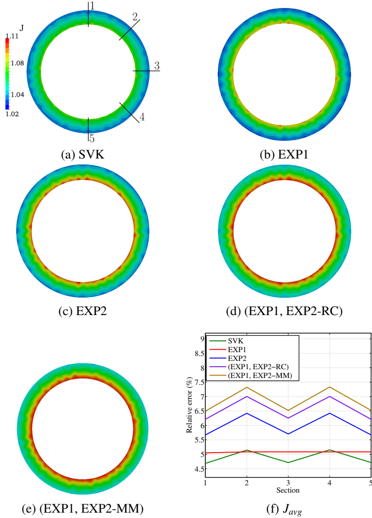
Figure 14: Volume ratio J and J_{avg} at z = 1 cm, \Delta P = 150 mmHg for the different material models; \kappa = 9.0 \cdot 10^6 dyn/cm 2 .
