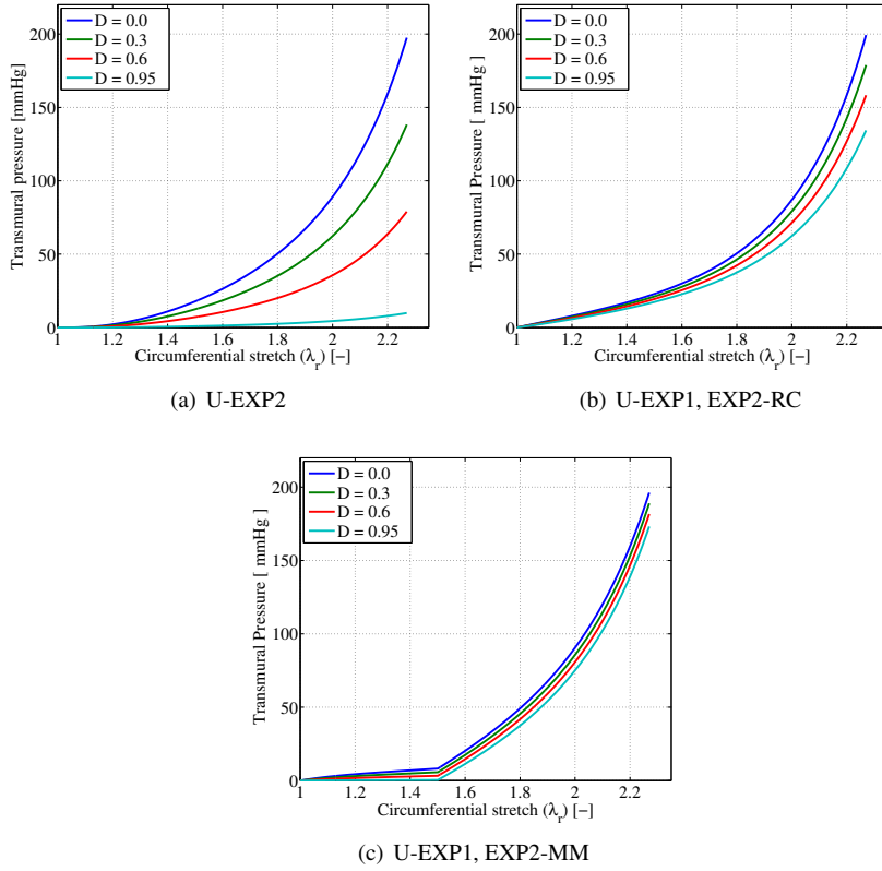
Figure 5: Functions \mathcal{T}(\lambda_r) for different values of the weakening parameter D .
