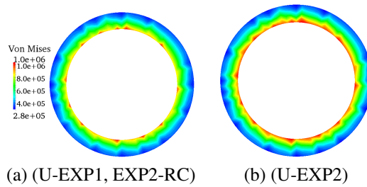
Figure 24: Case 2: Von Mises stress [dyn/cm 2 ] on the undeformed cross section at z = 1 cm and \Delta P = 110 mmHg.
