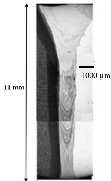
(b) Cross-sectional weld macrograph
