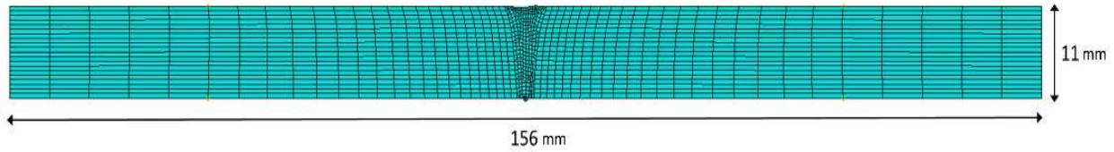
Fig. 5. Finite element mesh of the 2D cross-sectional model for dissimilar metal EB welded plate [20]
