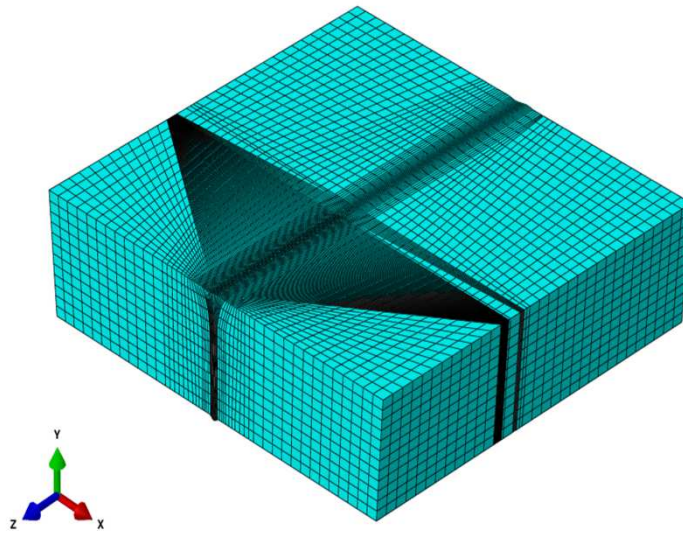
(b) FE mesh
