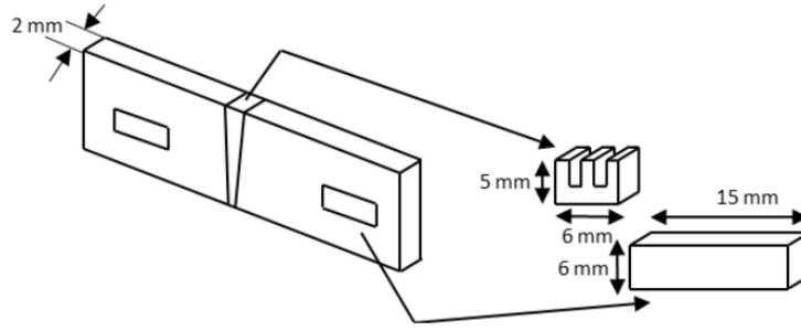
Fig. 4. Schematic of the d_0 specimens.
