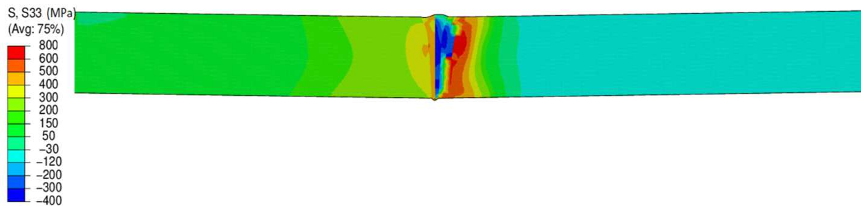
Fig. 13. Contour map showing the longitudinal residual stress profile at mid-section of the plate.
