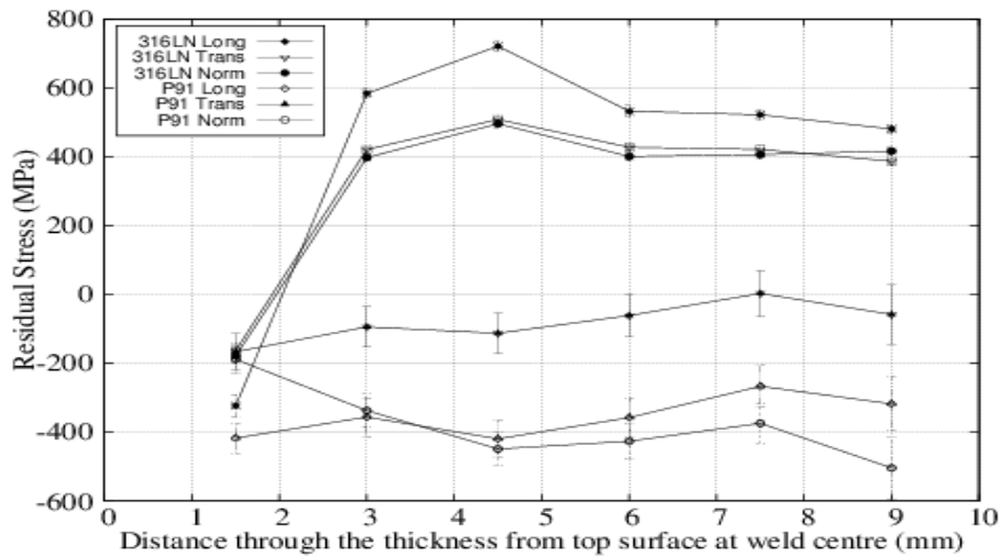
Fig. 12. Stress through the weld fusion zone at the weld centre.
