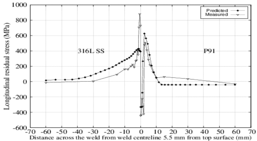
Fig. 14. Comparison of predicted and measured longitudinal residual stress across the weld.
