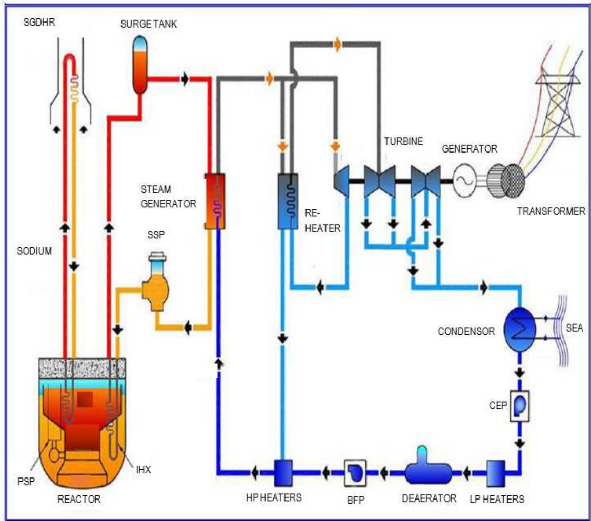
(a) Schematic of the prototype fast breeder reactor
