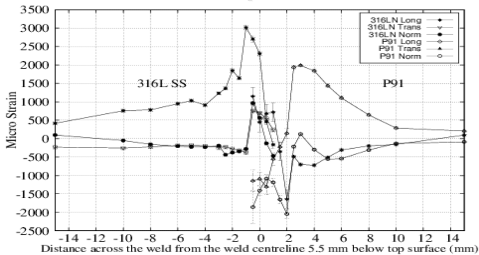
Fig. 9. Strain across the weld in 316LN and P91 materials.
