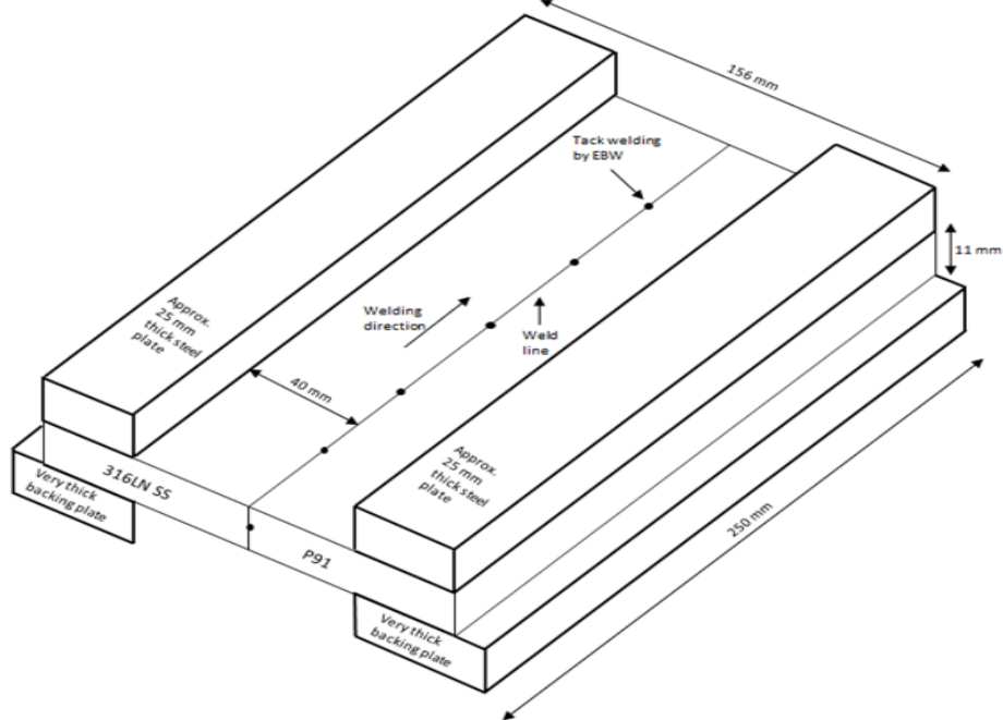
(a) Schematic of the dissimilar metal EB welded sample with restraining larger steel plates
