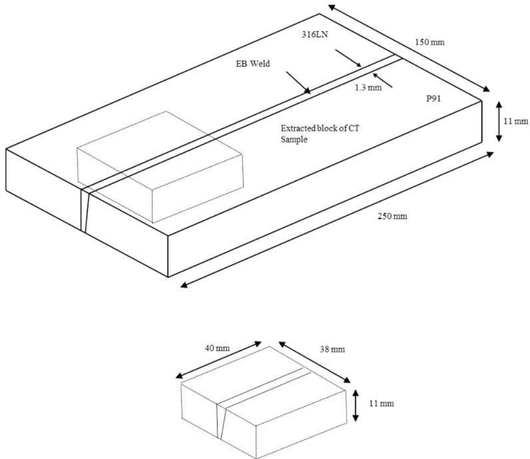
Fig. 6. Schematic of the C(T) specimen location in the dissimilar metal welded plate.
