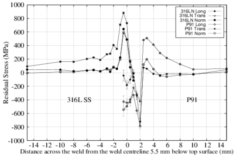
Fig. 11. Stress across the weld in 316LN and P91 materials.
