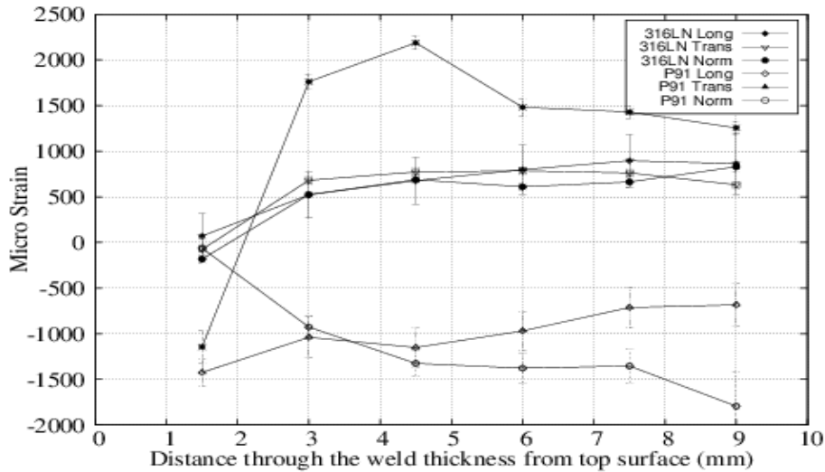
Fig. 10. Strain through the weld fusion zone at the weld centre.
