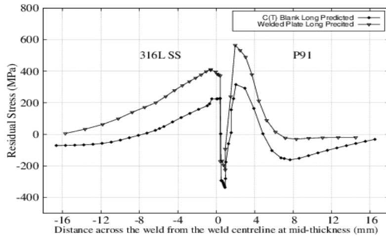
(a) Residual stress in the welded plate and the C(T) specimen
