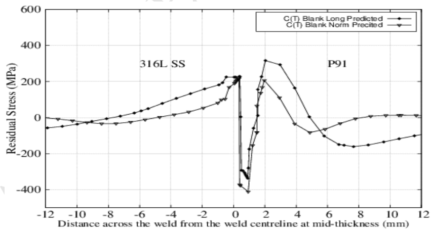
Fig. 16. Predicted longitudinal and normal residual stress in the C(T) blank specimen.
