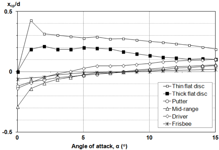
Figure 6 Location of X_{cp}/d for commercial golf discs.
