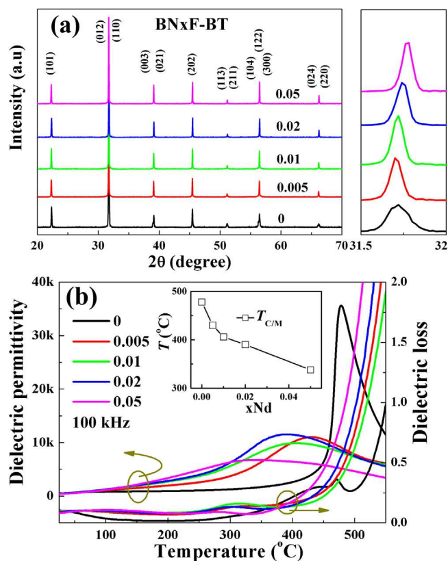
Fig. 1. (a) RT XRD patterns of \text{BNxF-BT} and (b) Temperature dependence of \epsilon_r and \tan \delta at 100 kHz for \text{BNxF-BT} , inset shows T_{C/M} as a function of Nd concentration.
