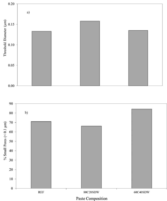
Fig. 3. Influence of SDW content on a) the threshold diameter (TD) and b) the percentage of small pores (< 0.1 µm) of pastes P1, P2 and P3.
