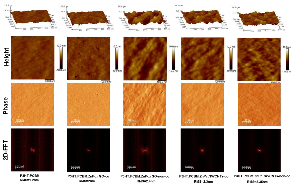
Fig. 2 AFM images of P3HT:PCBM:ZnPc-hybrid films with phase contrast and 2D-FFT analysis.
