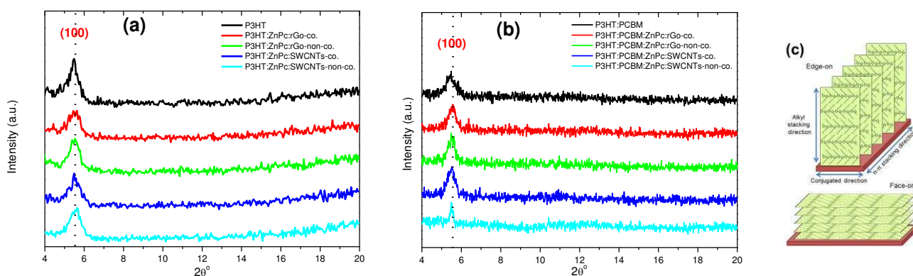
Fig. 6 (a) XRD patterns of P3HT-hybrid films; (b) XRD patterns of P3HT:PCBM:ZnPc-hybrid films; and (c) orientation of P3HT
