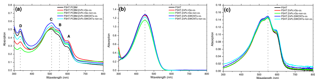
Fig. 5 (a) The absorption spectra of P3HT:PCBM:ZnPc-hybrid films; (b) Absorption spectra of P3HT-hybrid solution samples; and (c) Absorption spectra of P3HT-hybrid films samples
