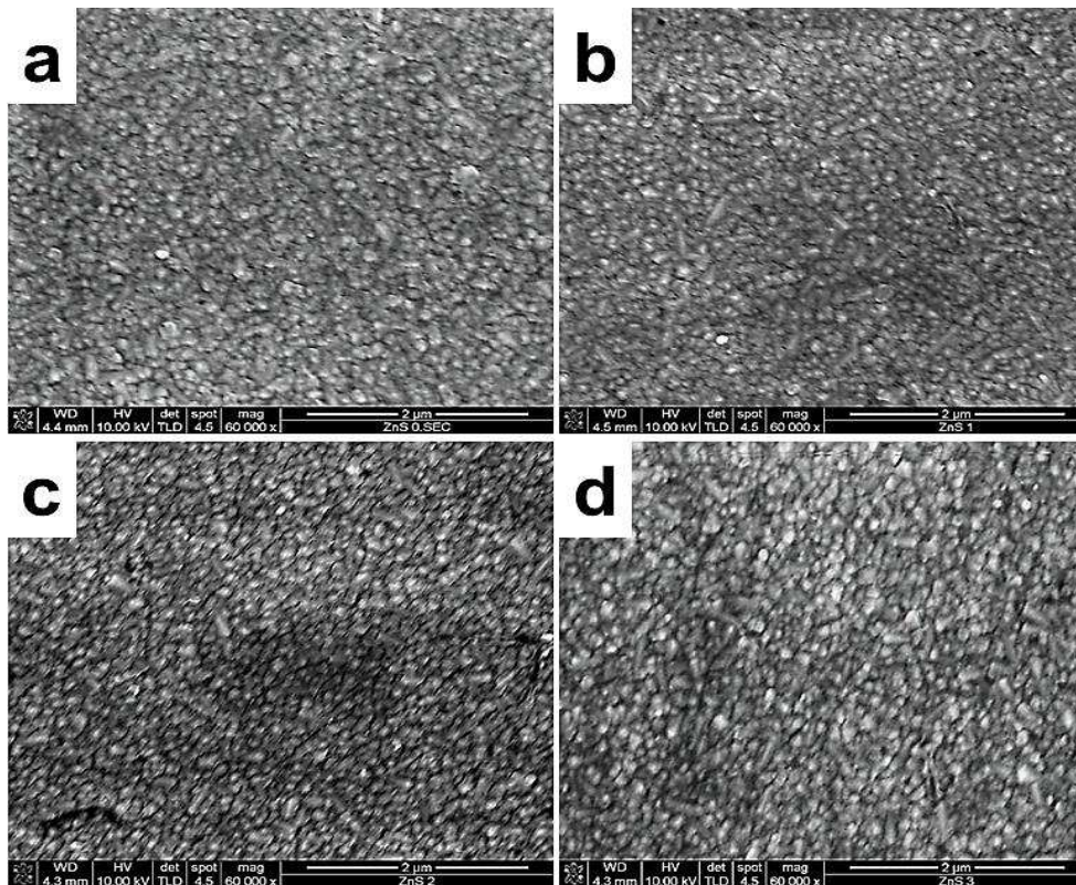
Figure 6: SEM images for (a) as-deposited and (b), (c), and (d) for heat-treated glass/FTO/ZnS layers at 100°C, 200°C and 300°C respectively for 15 min in air. The layer was grown at 1450 mV, to obtain a thickness of ~880 nm.
