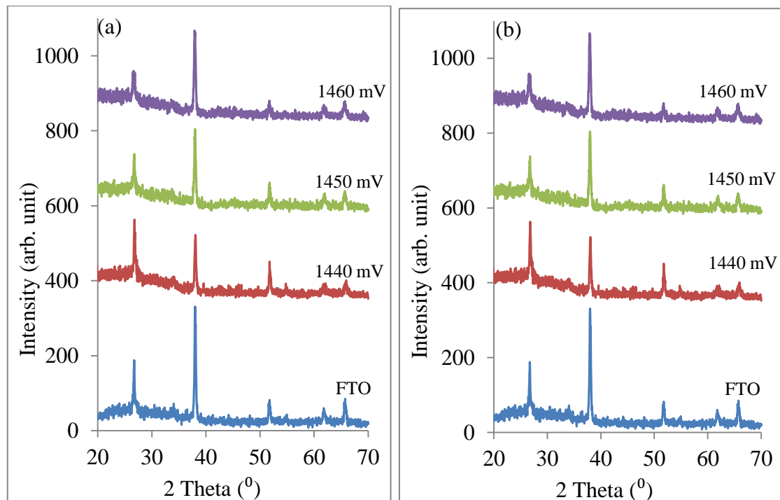
Figure 3: XRD patterns of ZnS layers grown on glass/FTO substrate at different cathodic potentials for (a) as-deposited and (b) heat-treated (at 350°C for 15 minutes in air) layers.
