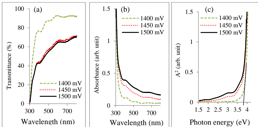
Figure 5: (a) transmittance (b) absorbance and (c) optical bandgap of heat-treated ZnS thin films deposited at different growth voltages.
