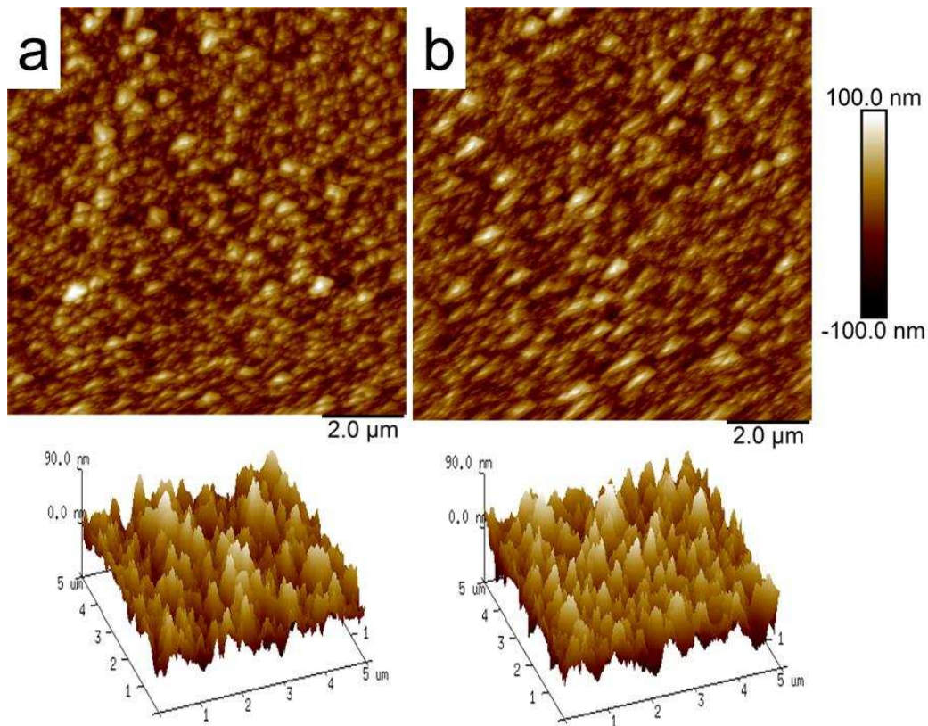
Figure 7: 2D and 3D AFM images of (a) as-deposited and (b) heat-treated ZnS layers grown on glass/FTO substrate.
