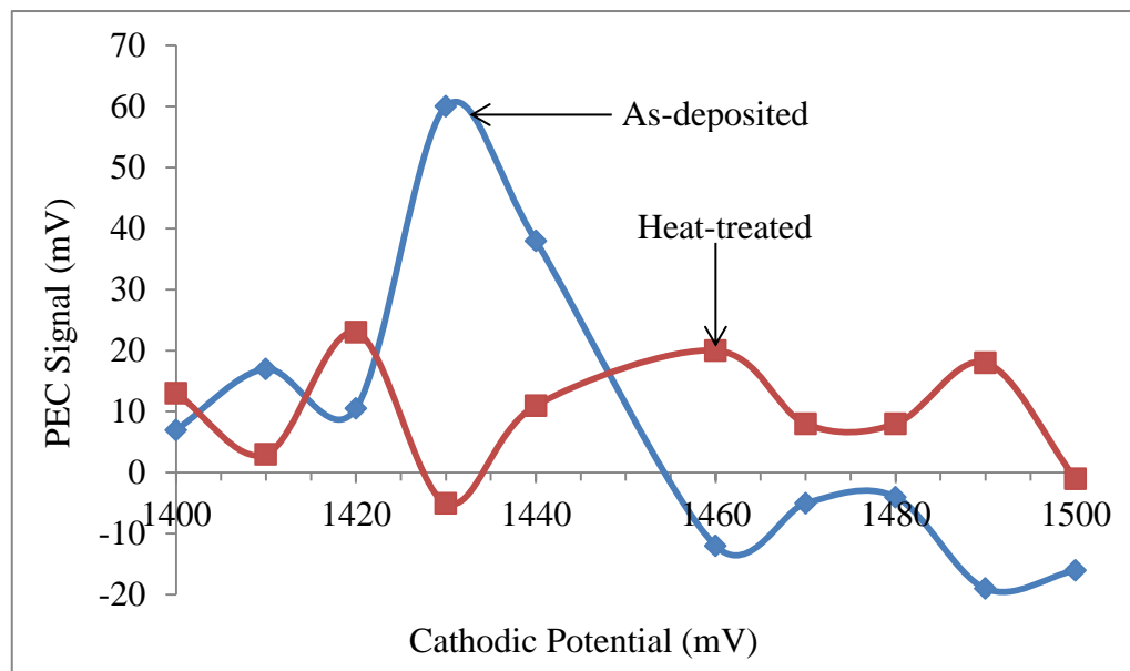
Figure 2: PEC cell measurement for both as-deposited and heat-treated ZnS layers.
