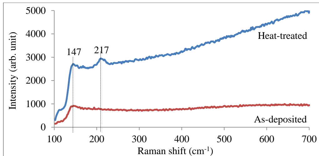
Figure 4: Typical Raman scattering spectra recorded on glass/FTO/ZnS thin films of as-deposited and heat-treated (at 350°C for 15 min in air) samples.
