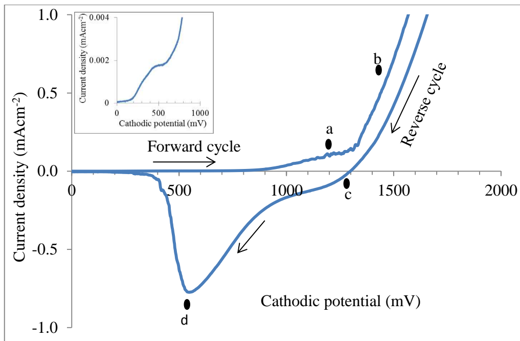
Figure 1: Cyclic voltammogram of the aqueous solution containing 0.15M \text{ZnSO}_4 + 0.15M (\text{NH}_4)_2\text{S}_2\text{O}_3 in 400 ml of de-ionised water. Both the growth temperature and the pH were set to \sim 30^\circ\text{C} and 4.00 \pm 0.02 respectively.
