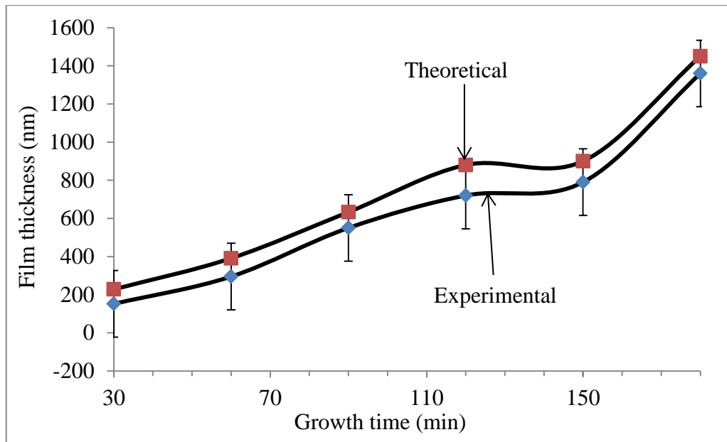
Figure 8: Plot of theoretical and experimental thickness estimated for electroplated ZnS films.
