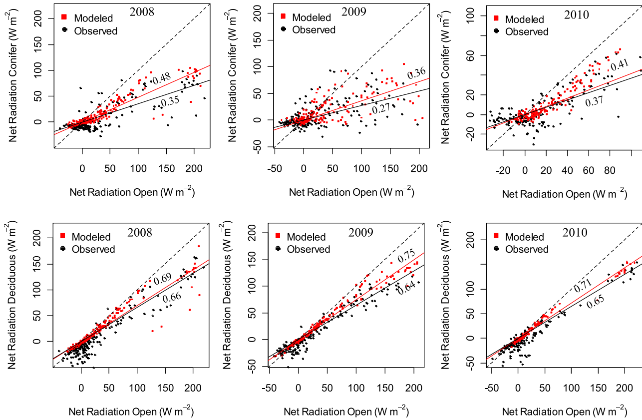
Figure 11. Observed and modeled below canopy net radiation presented in comparison to open area net radiation (observed and modeled) for the years 2008, 2009 and 2010. Solid lines are least square fits constrained to go through the origin. The regression slope is indicated for each line and gives the average fraction of under canopy net radiation as compared to net radiation in the open.
