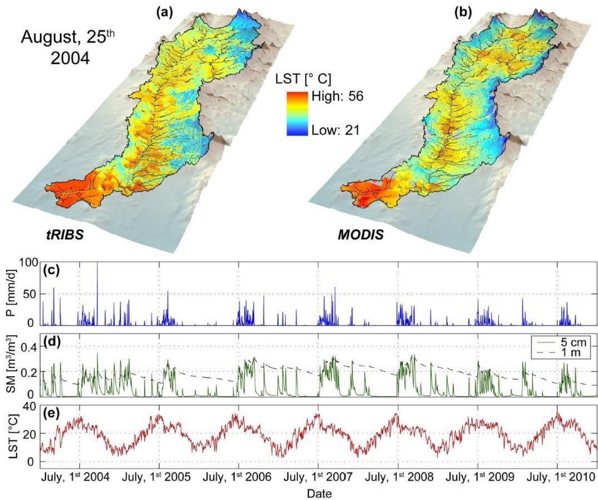
Figure 2. High-resolution ( \sim 70 m) hydrologic simulations with the tRIBS model in the Rio San Miguel basin ( 3796 \text{ km}^2 ), Mexico, from January, 1 st 2004 to December 31 st , 2010. Spatially-distributed hydrometeorological forcings were provided by hourly products from the North America Land Data Assimilation System (NLDAS), bias-corrected with ground observations. Hydrologic simulations were validated by comparing (i) time series of simulated and observed soil moisture (SM) and land surface temperature (LST) at nine distributed locations, and (ii) simulated SM and LST maps against remote sensing products from the 2D-Synthetic Aperture Radiometer (2D-STAR) and Moderate Resolution Imaging Spectroradiometer (MODIS), respectively. The LST maps simulated by tRIBS and observed by MODIS on August, 25th 2004 are presented in panels (a) and (b), respectively. A root mean square error of 4.0 \text{ }^\circ\text{C} and a correlation coefficient of 0.67 were obtained after resampling the
