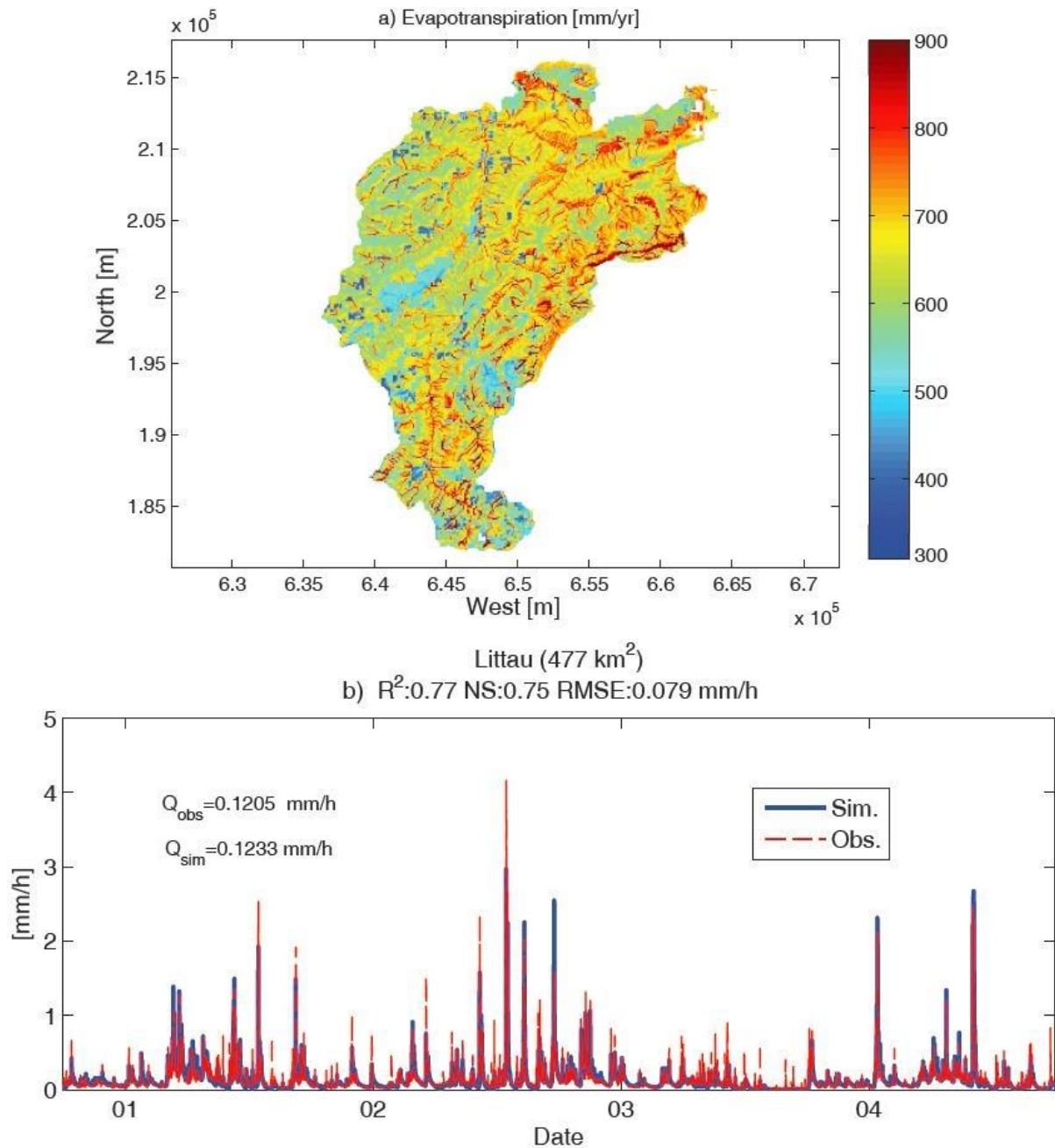
Figure 1. High-resolution (~100 m) un-calibrated hydrological simulations with the process-based ecohydrological model Tethys-Chloris at the hourly time scale for the Kleine-Emme catchment (477 km 2 ) (Switzerland) for the period 1 st October 2000 to 30 th September 2004. Spatially distributed forcing was provided by Meteo-Swiss and includes hourly station measurements of air temperature, wind speed, relative humidity, shortwave radiation and a gridded precipitation product RhiresD. Simulation results are presented for distributed evapotranspiration averaged over the four years (a) and streamflow at the catchment outlet (b). The match in water budget amount ( Q_{obs} and Q_{sim} are the observed and simulated annual mean
