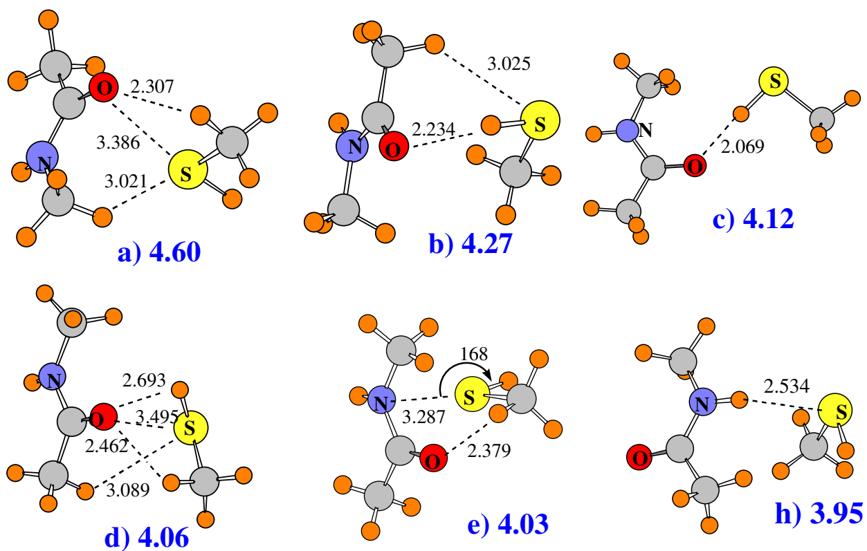
Fig 1. Optimized geometries of various minima on the potential energy surface of the CH 3 SH/NMA heterodimer. Large blue numbers represent binding energies, in kcal/mol. Distances in Å and angles in degrees.
