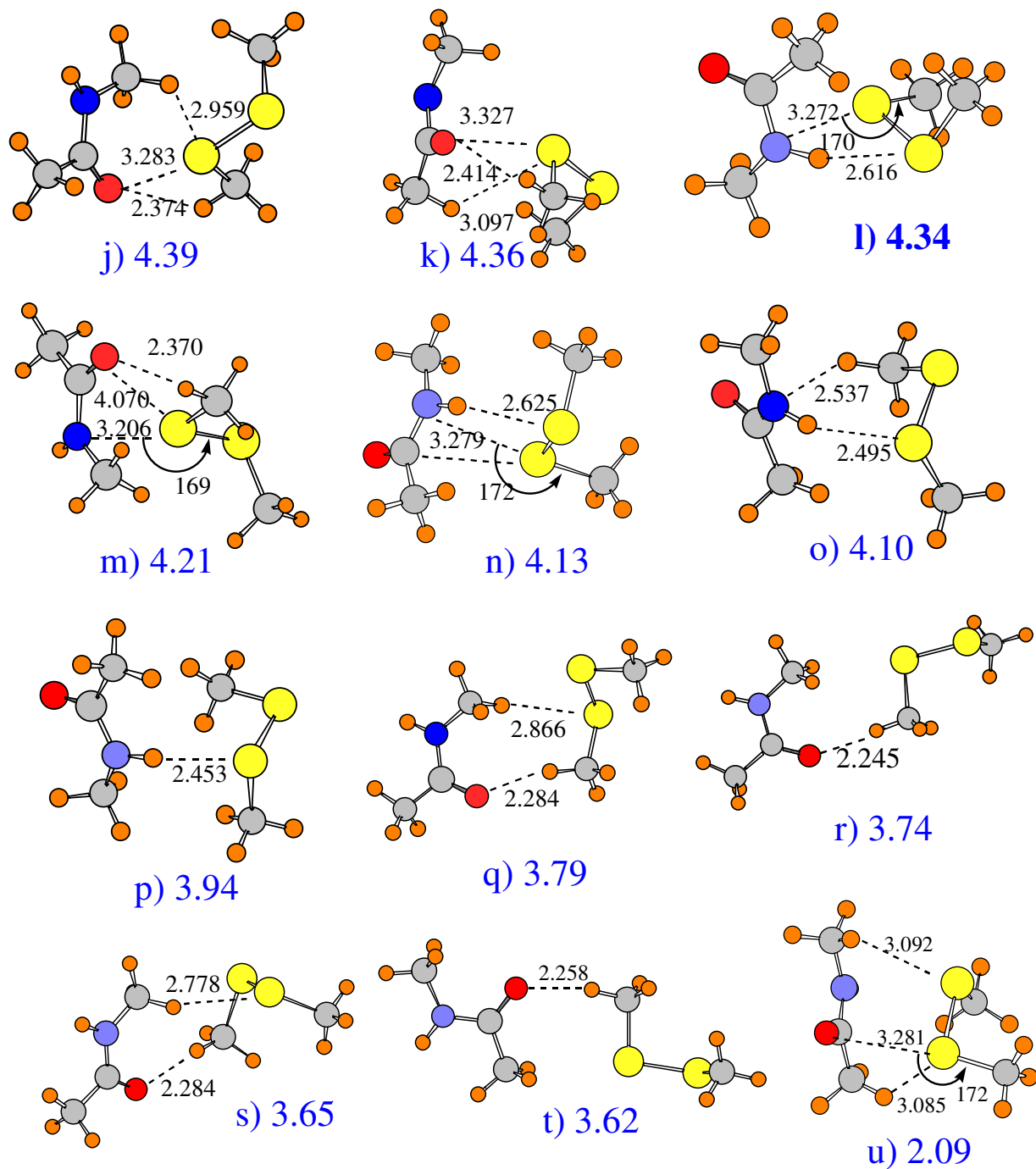
Fig S3. Optimized geometries of various minima on the potential energy surface of the \text{CH}_3\text{SSCH}_3/\text{NMA} heterodimer. Large blue numbers represent binding energies, in kcal/mol. Distances in Å and angles in degrees.
