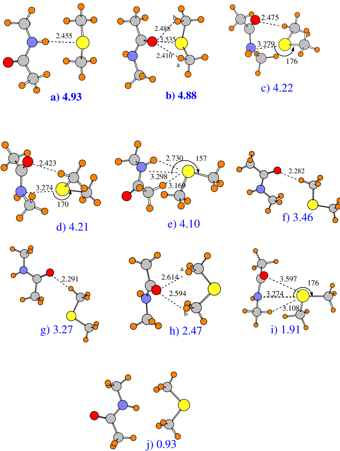
Fig S2. Optimized geometries of various minima on the potential energy surface of the \text{CH}_3\text{SCH}_3/\text{NMA} heterodimer. Large blue numbers represent binding energies, in kcal/mol. Distances in Å and angles in degrees.
