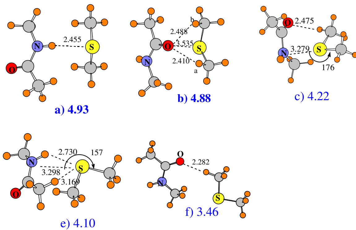
Fig 2. Optimized geometries of various minima on the potential energy surface of the CH 3 SCH 3 /NMA heterodimer. Large blue numbers represent binding energies, in kcal/mol. Distances in Å and angles in degrees.
