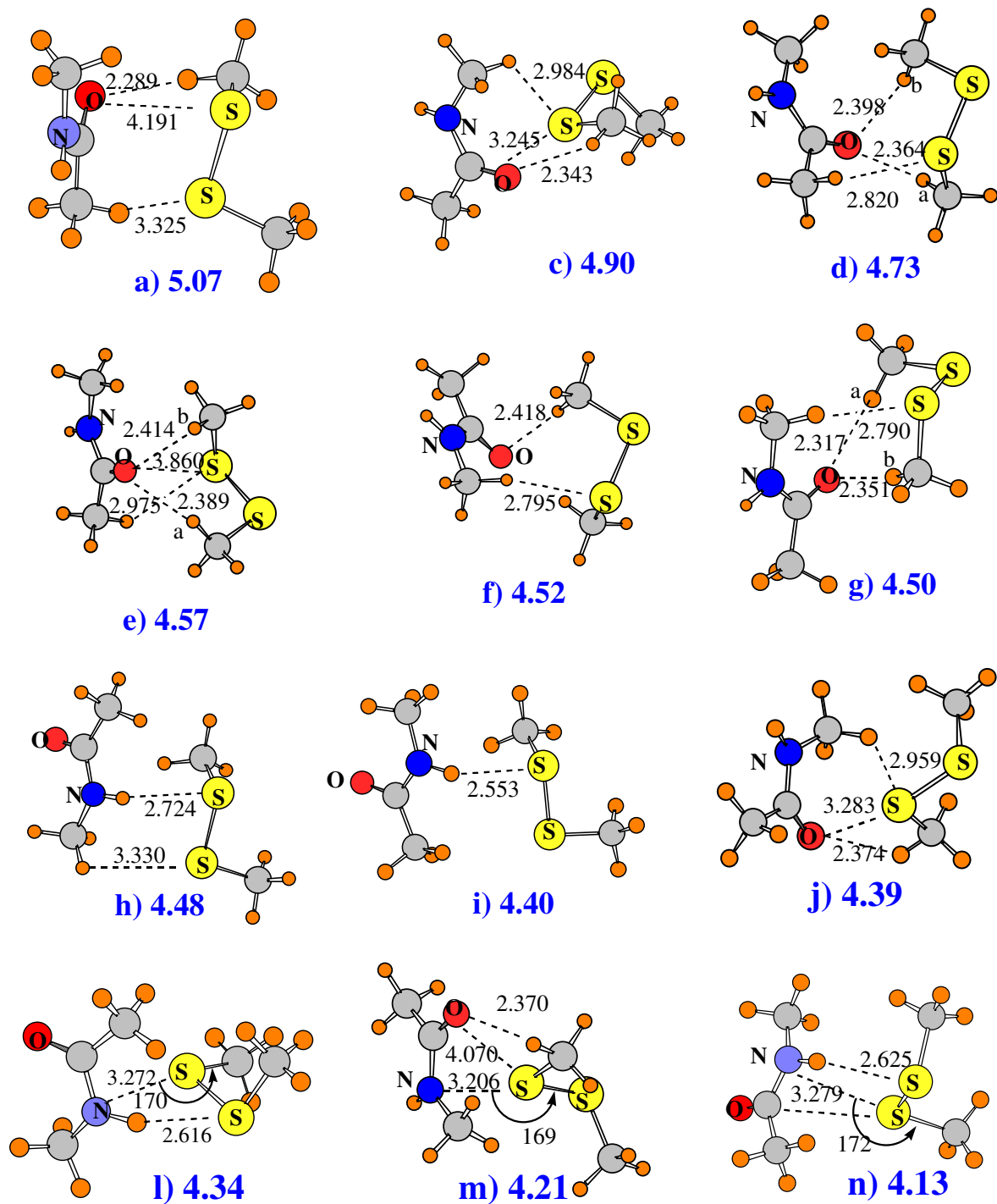
Fig 3. Optimized geometries of various minima on the potential energy surface of the \text{CH}_3\text{SSCH}_3/\text{NMA} heterodimer. Large blue numbers represent binding energies, in kcal/mol. Distances in Å and angles in degrees.
