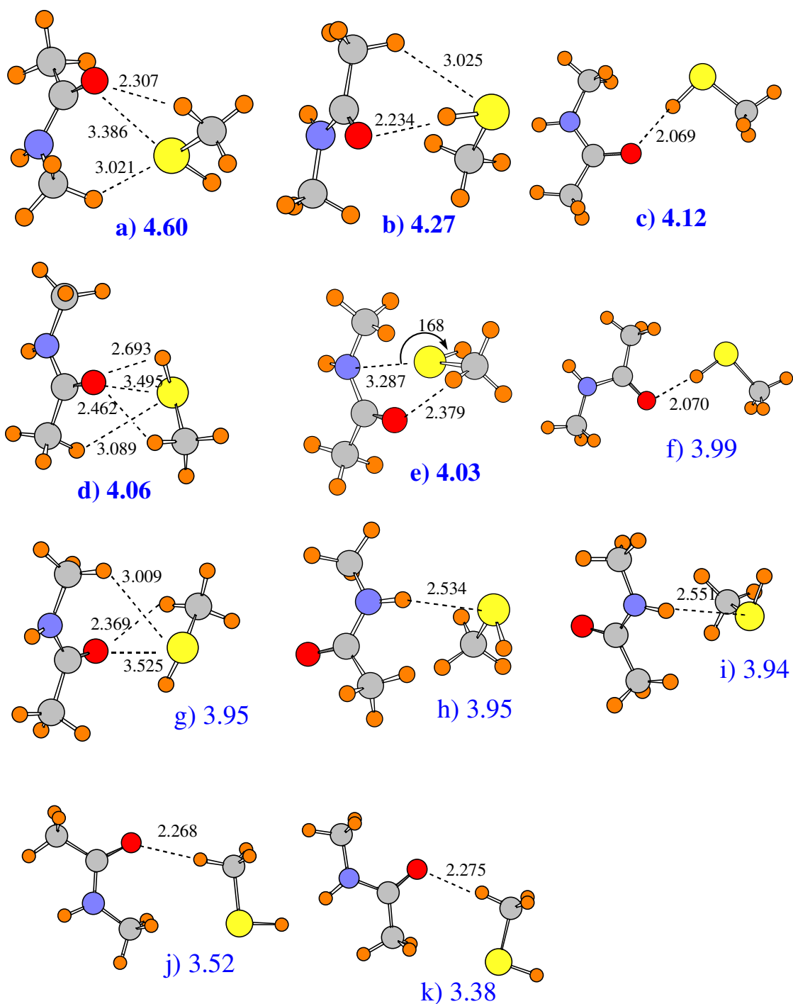
Fig S1. Optimized geometries of various minima on the potential energy surface of the CH 3 SH/NMA heterodimer. Large blue numbers represent binding energies, in kcal/mol. Distances in Å and angles in degrees.
