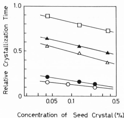
Figure 6. Relationship between relative crystallization time of cocoa butter and concentration of seed materials at T_c = 30^\circ\text{C} : (●) cocoa butter (Form VI); (○) SOS ( \beta_1 ); (Δ) BOB ( \beta_2 ); (▲) BOB (pseudo- \beta' ); (□) SSS ( \beta ) (Hachiya et al., 1989a).
