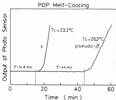
Figure 4. Output of photo sensor in case of simple cooling of POP at T_c = 23.2 and 26.3 °C (Koyano et al., 1989). The crystallization rates differ for the two polymorphs.
