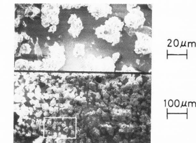
Figure 10. Cryo-scanning electron micrograph, taken at -100^{\circ}\text{C} \sim -130^{\circ}\text{C} of BOB ( \beta_2 ) powders pulverized at -60^{\circ}\text{C} \sim -100^{\circ}\text{C} .
