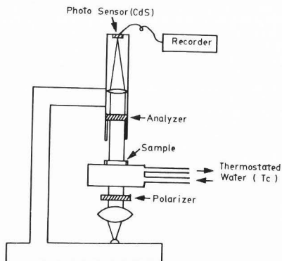
Figure 3. Optical system for induction time measurement of melt crystallization. (Koyano et al., 1989).
