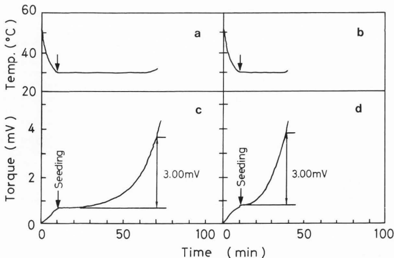
Figure 5. Changes of torque and temperature of dark chocolate seeded with SOS ( \beta_1 ) at T_c = 30^\circ\text{C} : (a, c) 0.035 weight %, and (b, d) 0.5 weight % (Hachiya et al., 1989a).
