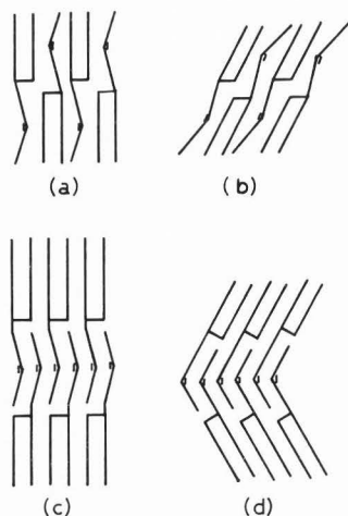
Figure 2. Postulated structure models of POP polymorphs: (a) \alpha , (b) pseudo- \beta' , both are double chain length, (c) \gamma , and (d) \beta_2 and \beta_1 , which are triple chain length of POP (Sato et al., 1989). Unsaturation chains are indicated by dash (-) parallel to the chain.
