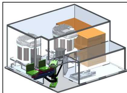
Fig. 1. First prototype of the low-cost rehab robot developed at BYU
