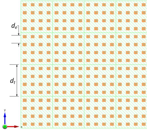
Fig. 8. Array panel consisting of 4 \times 4 tiles.
