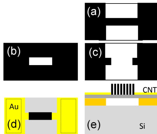
Fig. 5 (a) mask 1 (b) Mask 2 (c) Mask 3 (d) Top view and (e) side view of the CNT bolometer.
