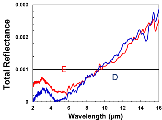
Fig. 3 CNT forest of E (red) is about twice as tall as D (blue) but their CNT density is about the same.
