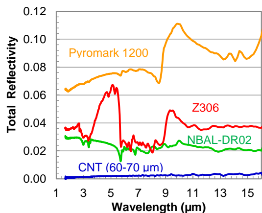
Fig. 1 Total reflectance of a CNT forest of 60-70 \mu\text{m} in height comparing with those of black paints.
