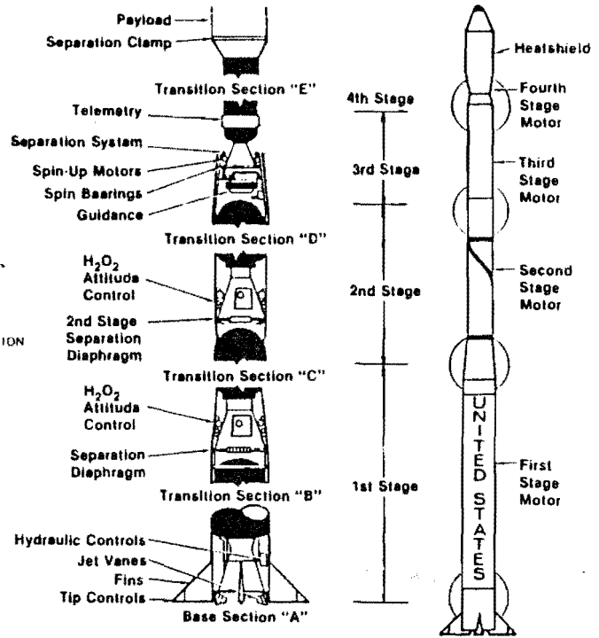
Figure 7: Major Assemblies
