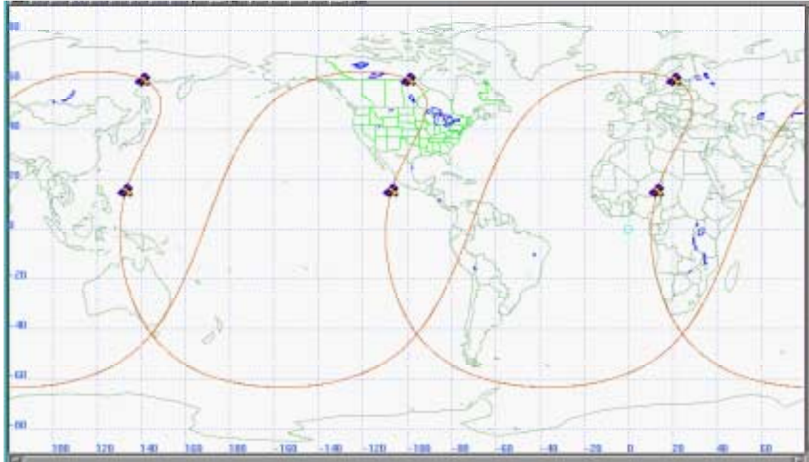
Fig. 4 Right Leaning COBRA Track with Six Satellites (Satellites at 60°N are at start of active arc; those at 15°N are at end of active arc)
