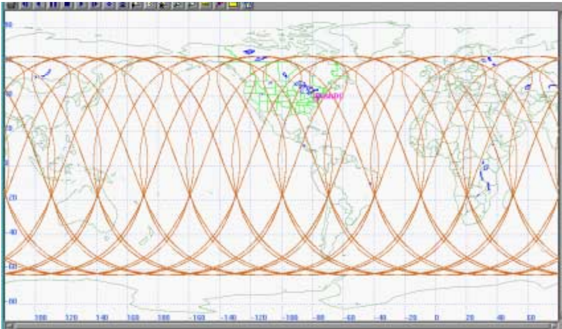
Fig. 6 Diagram Showing 12 Northern Hemisphere Teardrops. (This is the Maximum Number Possible While Maintaining at Least Two Degrees Separation between Adjacent Teardrops)
