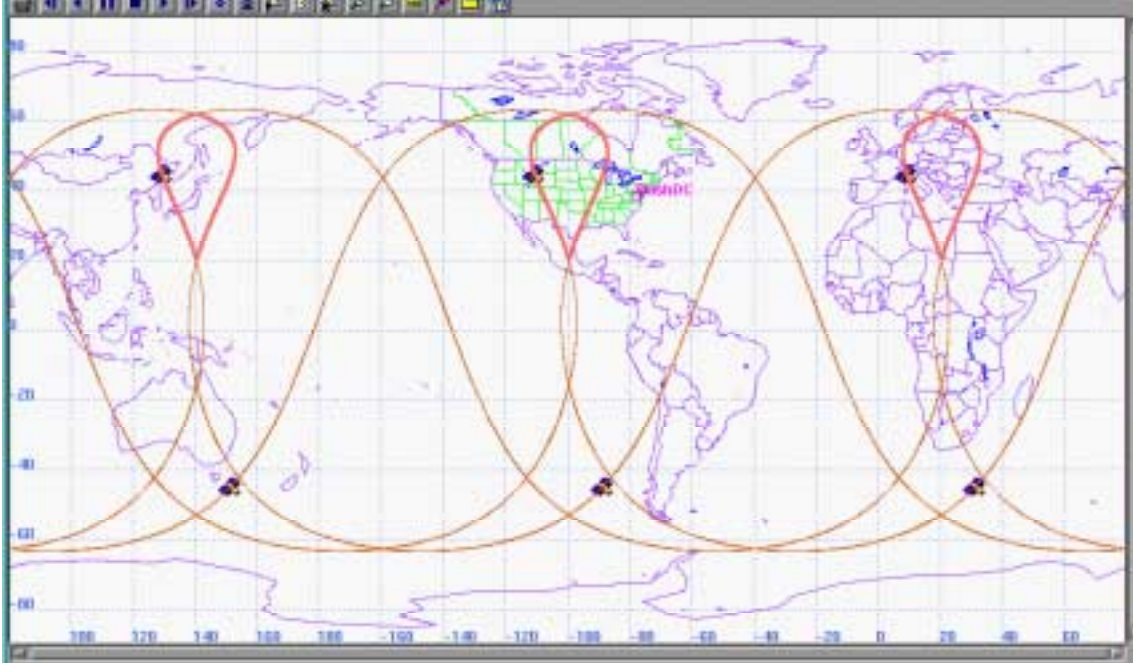
Fig. 5 Basic 6-Satellite Teardrop Array. Left-Leaning Satellites at Apogees; Right-Leaning Satellites at Perigees
