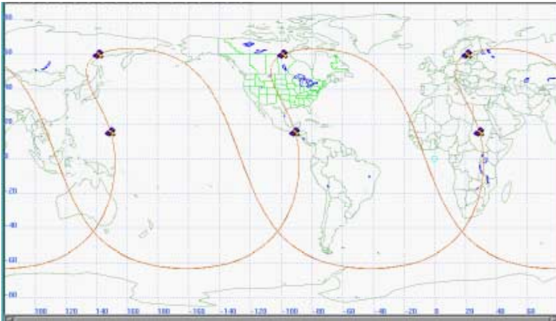
Fig. 3 Left Leaning COBRA Track with Six Satellites (Satellites at 15°N are at Start of Active Arc. Those at 60°N are at End of Active Arc)
