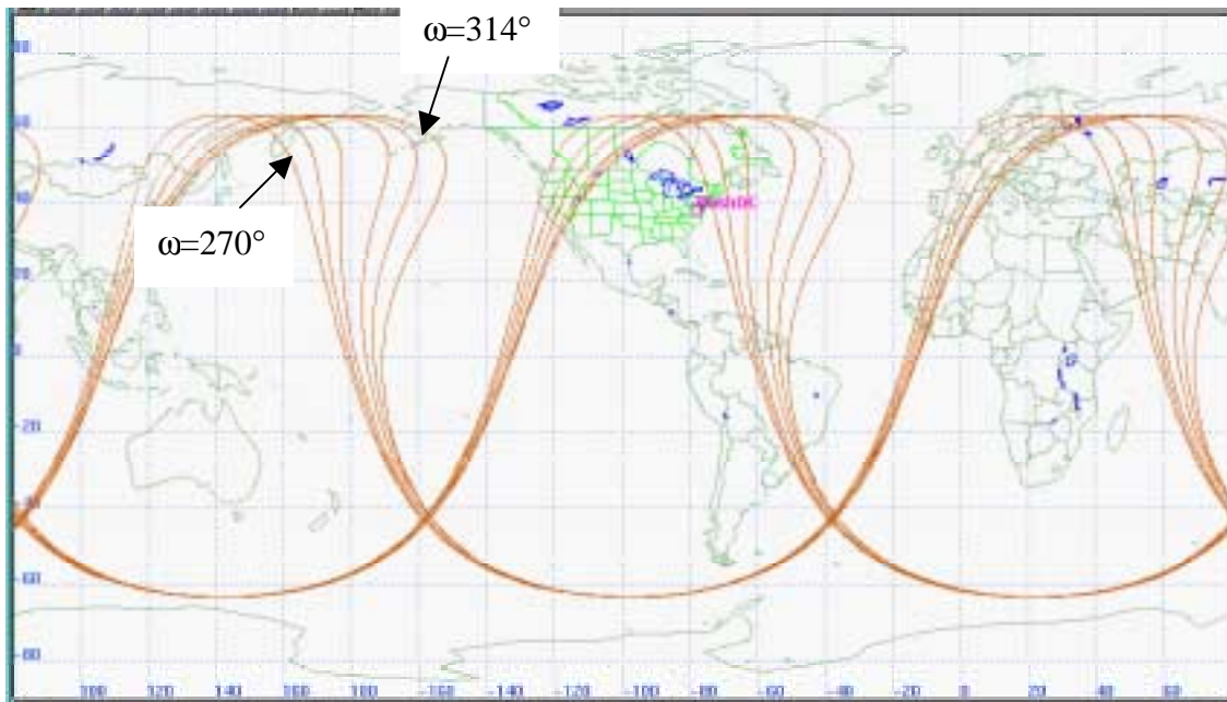
Figure 2 8-Hr Elliptic Ground Tracks with Varying Amounts of “Right Lean”
