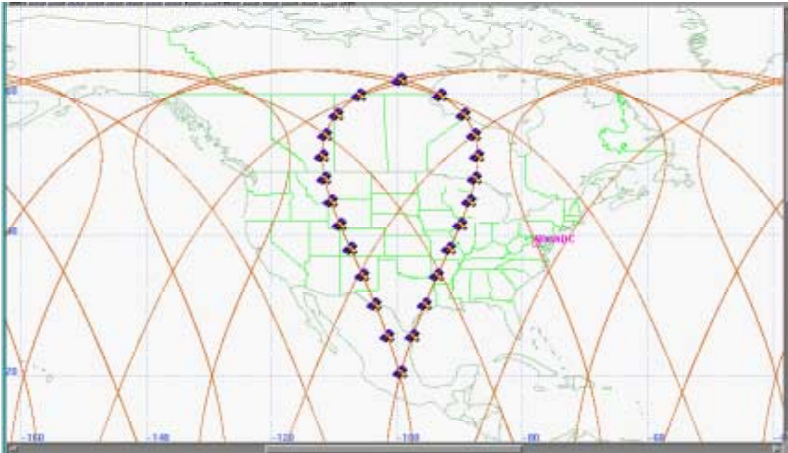
Fig. 7 Snapshot of Single Teardrop Showing Twenty-Four Active Satellites With a Minimum 2° In-Track Separation
