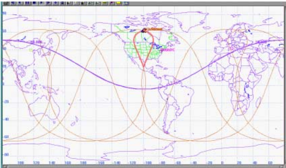
Fig. 9 Snapshot of US Teardrop Demo with Both Satellites at Northern Crossover Point over North America with minimum of 15-20 km separation to avoid collision (10° Elevation Angle Contour Line Shown)
