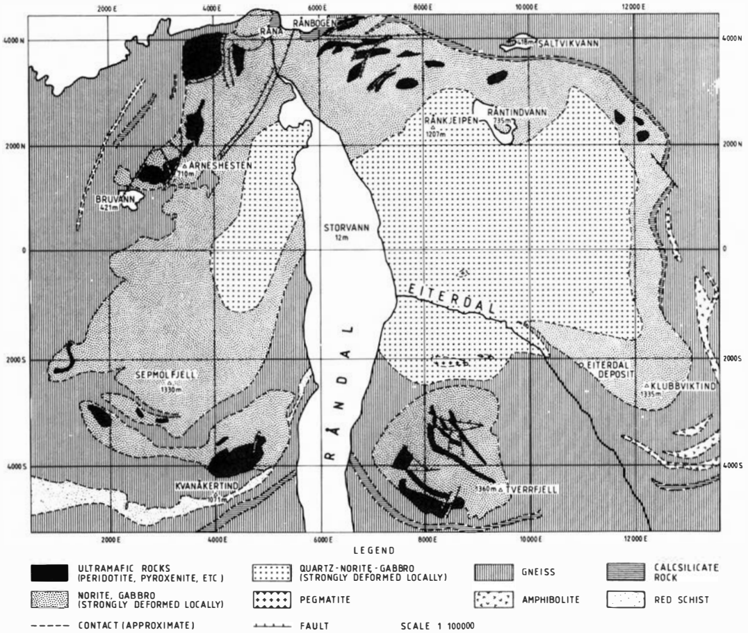
Fig. 2. Simplified geological map of the Råna area (Boyd & Mathiesen 1979). The coordinates are in metres.
