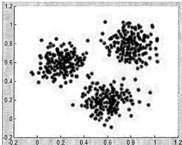
Figure3.8.: The less cluster radius is selected, the more clusters are defined. The maximum number of classes would correspond to the number of individuals.
