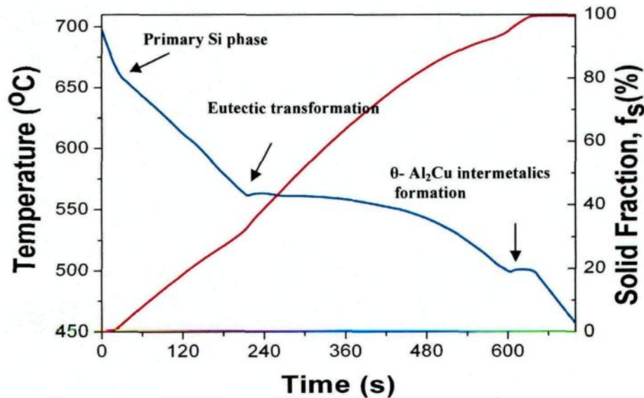
Fig. 7.1 Temperature and fraction solid versus time for A390 aluminum alloy cooled in steel mould.
