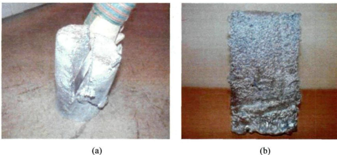
Fig. 4.2 The novel method of preparing the semi-solid slurries provides ingots that are self-supporting and easy to cut.
