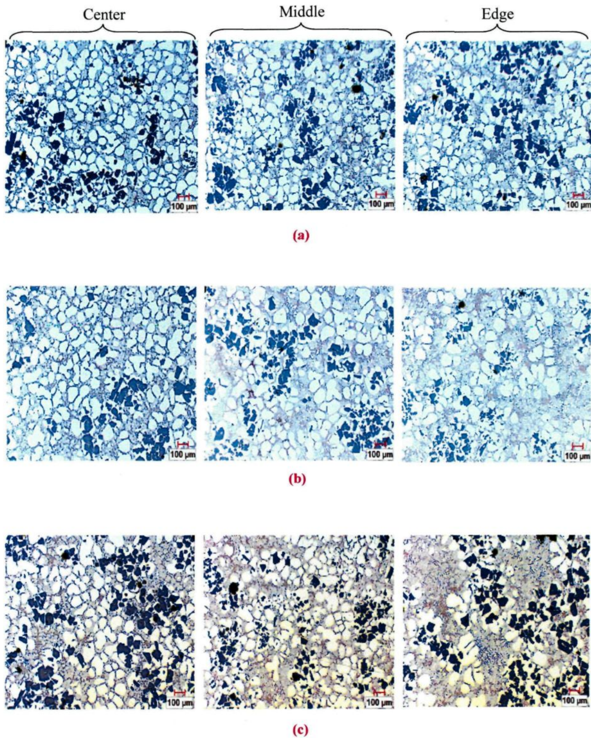
Fig. 7.3 Microstructure of P-refined A390 SSM billets from the center to the edge, deformed at different solid fractions: (a) at 0.6, (b) 0.5, (c) 0.4.
