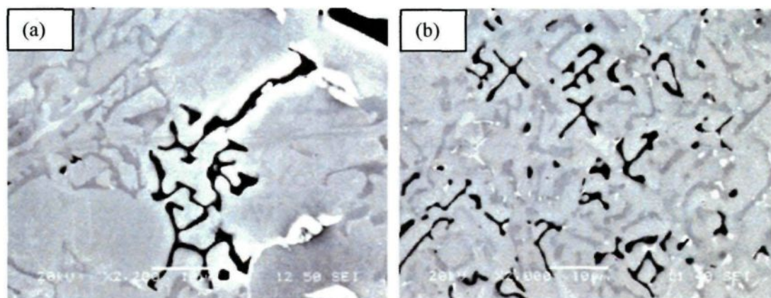
Fig. 6.9 SEM micrographs showing the eutectic Mg_2Si deep etched samples of the Al-15Si-14Mg-4Cu alloy modified with (a) 0 % Sr; (b) 0.08 % Sr.
