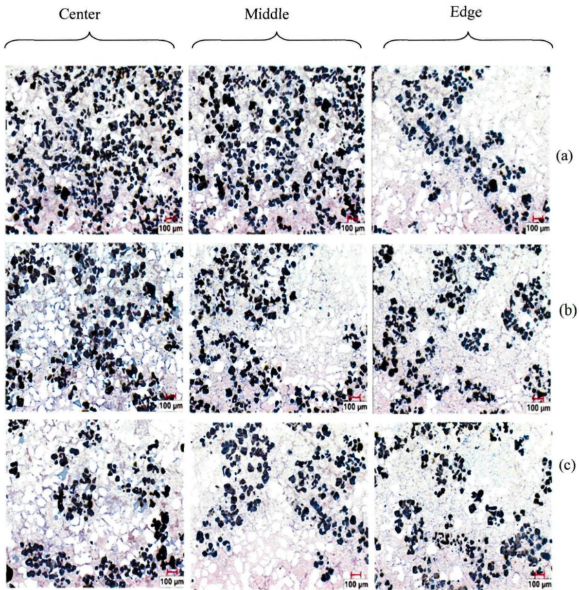
Fig. 7.11 Microstructure of Al-15Si-13.5Mg-4Cu SSM billets from the center to the wall deformed at different solid fractions: (a) at 0.6, (b) 0.5, (c) 0.4.
