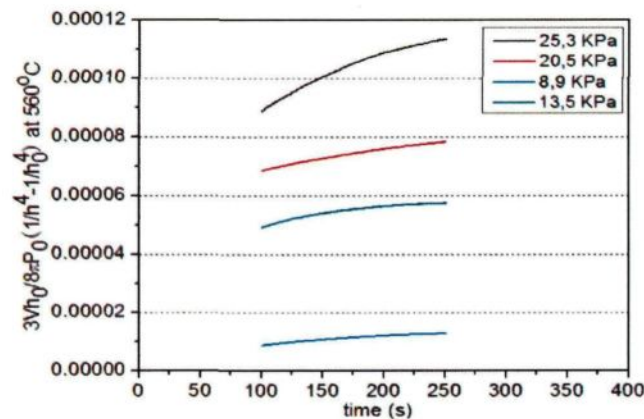
Fig. 7.7 Typical plot of [(3Vh_0/8\pi P_0) (1/h^4 - 1/h_0^4), \text{Pa}^{-1}] , against time for the unrefined samples at 560^\circ\text{C} .
