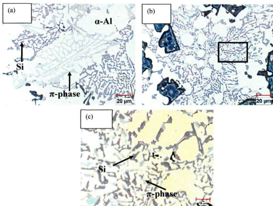
Fig. 6.13 Optical micrographs of: (a) alloy without modifier, (b) alloy with 0.08 pct Sr, (c) high magnification micrograph corresponding to the inset shown in (b).
