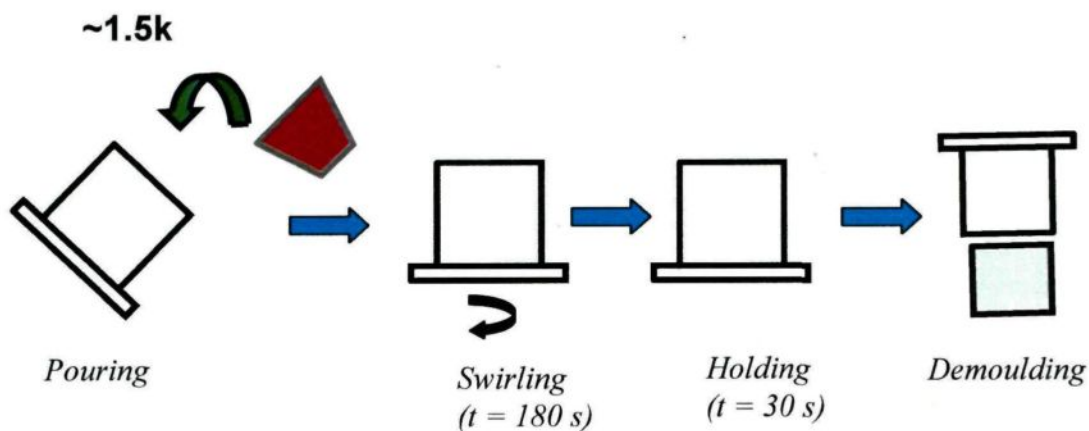
Fig. 3.5 Illustration of the steps involved in the conventional SEED process.
