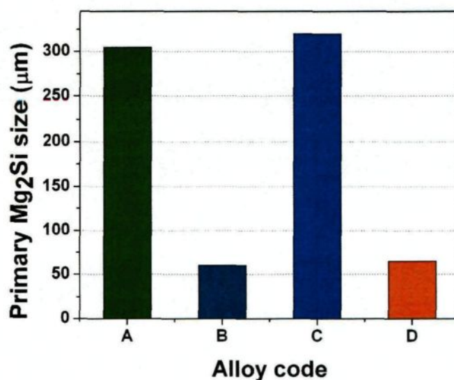
Fig. 6.4: The size of primary Mg_2Si particles in the alloy A (base alloy), alloy B (0.4% P), alloy C (0.08% Sr), and alloy D (0.08% Sr + 0.4% P).
