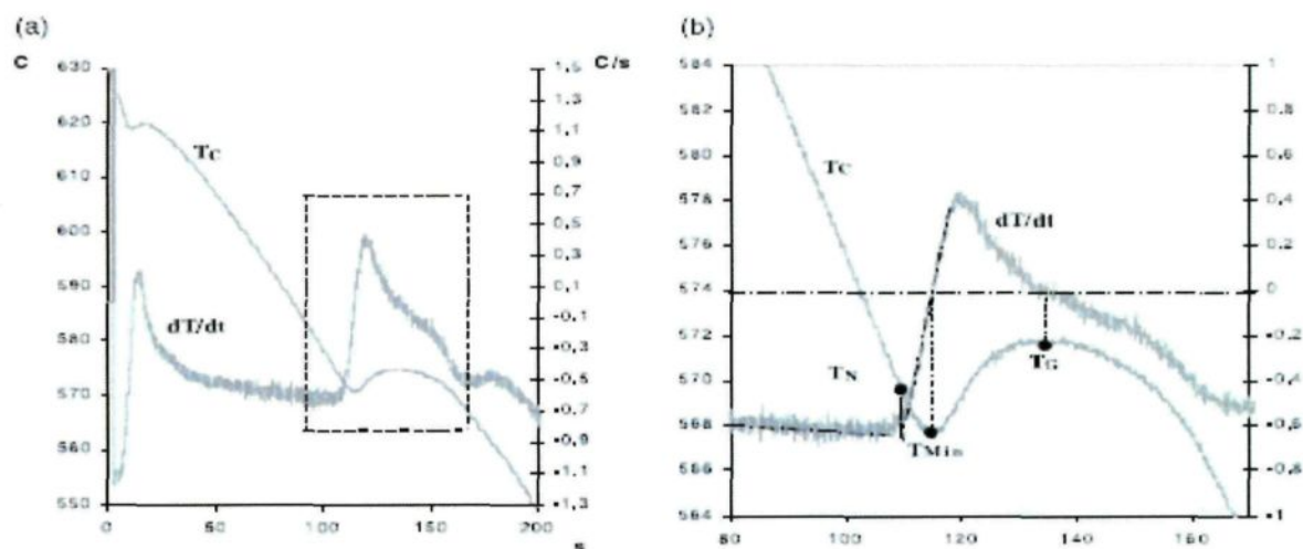
Fig. 3.4 Cooling curve, (a) first derivative and (b) representation of nucleation, growth and minimum temperatures.
