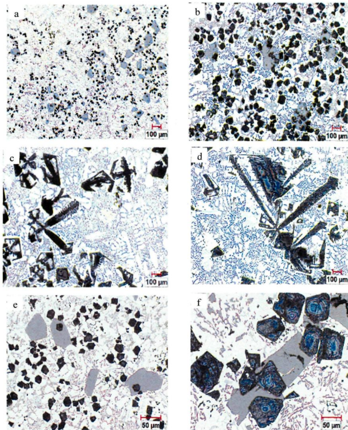
Fig. 5.3 Optical micrographs showing the typical structures obtained in the four alloys studied, containing (a) 6.15%, (b) 8.42%, (c) 12.82%, and (d) 14.86% Mg; (e, f) High magnification micrographs of (e) Alloy A, and (f) Alloy B. Note the change in size, morphology, and area fraction of the primary Mg 2 Si (black) and Si (grey) particles.
