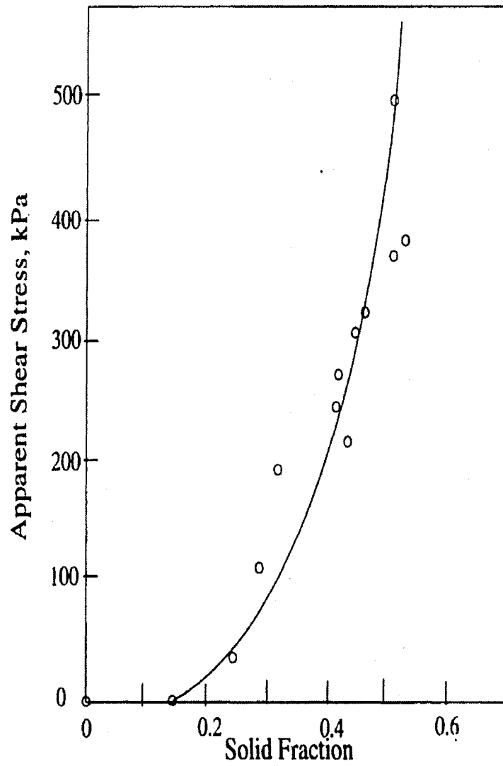
Fig. 2.10 Variation in yield stress with solid fraction for Sn-15%Pb alloy with dendritic structure [38].
