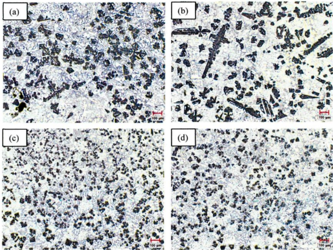
Fig. 6.2: Primary Mg_2Si morphologies of Al-15Si-14Mg-4Cu alloy containing: (a) no addition of P or Sr; (b) 0.08 % Sr; (c) 0.4 % P; (d) 0.08 % Sr and 0.4 % P.
