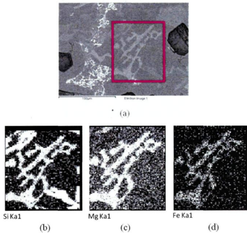
Fig. 5.10 (a) Backscattered electron image of alloy A and corresponding X-ray images showing distribution of (b) Si, (c) Mg, and (d) Fe in the \pi -Al 8 Mg 3 FeSi 6 phase shown in the inset in (a).
