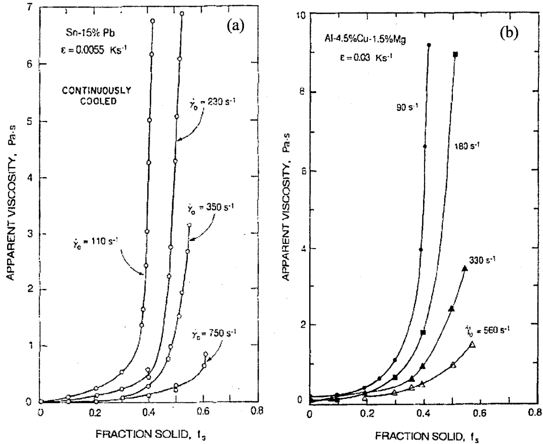
Fig.2-14 Influence of shear rate on apparent viscosity of semi-solid alloys (a) Sn-15wt.%Pb [42] and (b) Al-4.5wt.%Cu-1.5 wt.%Mg [10].
