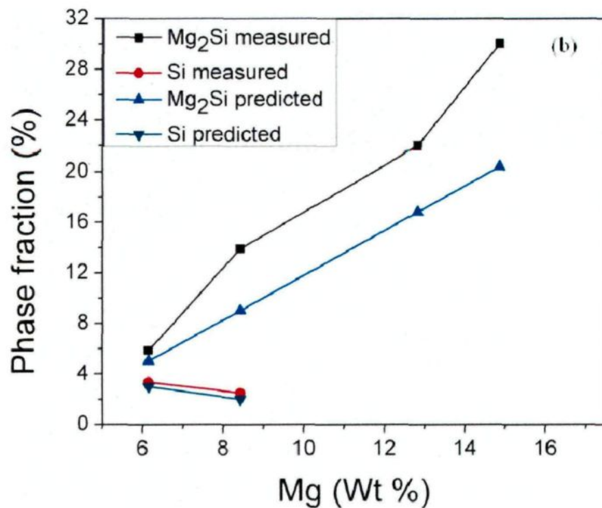
Fig. 5.7 Effect of Mg contents on the (a) mean particle size, (b) phase fraction of hypereutectic Al-Si-Cu-Mg alloys.
