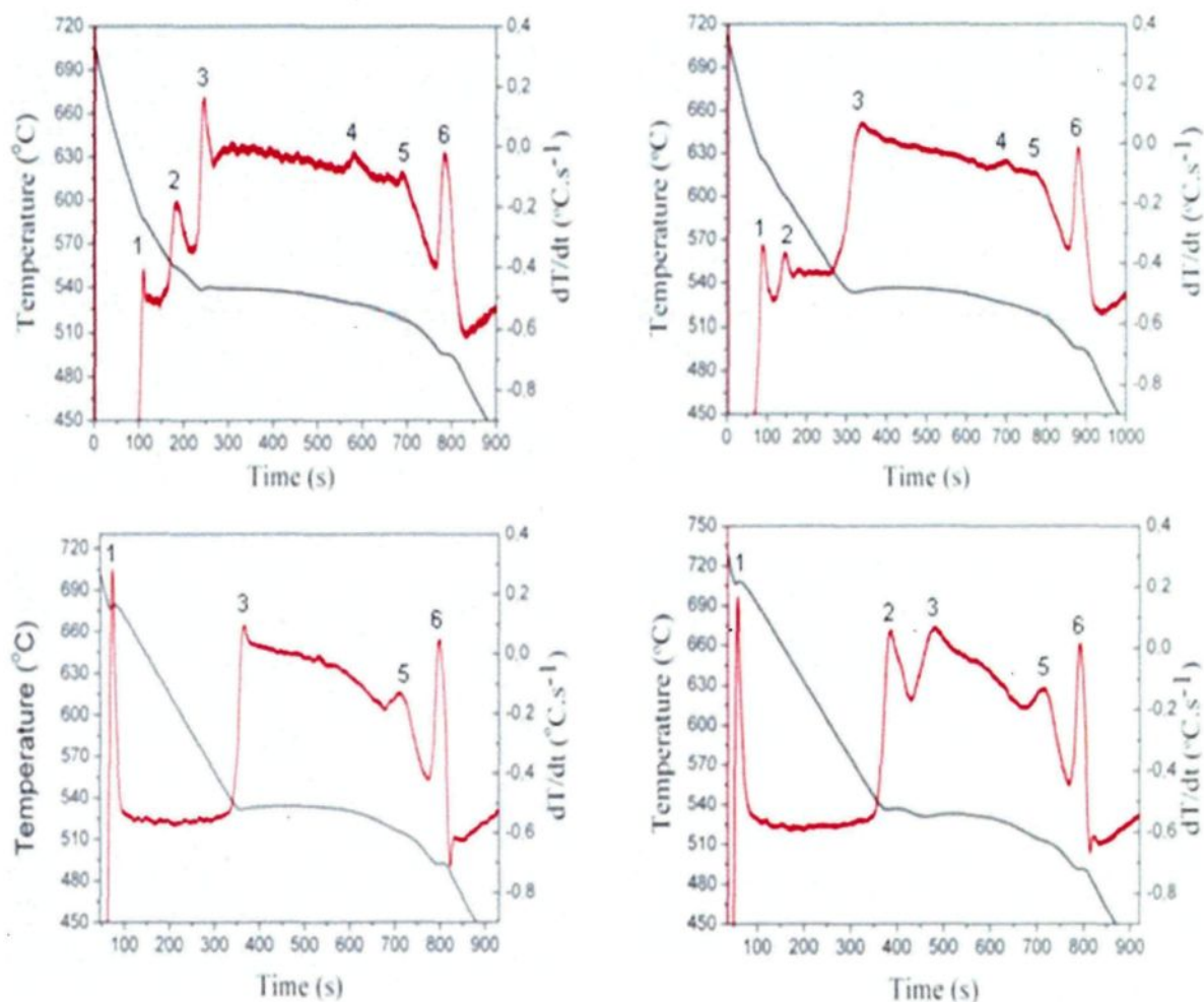
Fig. 5.8 Temperature vs time cooling curves and their first derivatives obtained for: (a) Alloy A, (b) Alloy B, (c) Alloy C, and (d) Alloy D.
