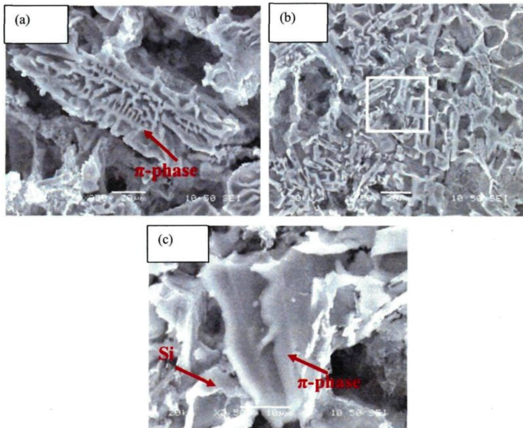
Fig. 6.14 SEM images showing \pi -Fe morphology in deep etched samples of: (a) alloy without modifier, (b) alloy with 0.08 pct Sr, (c) high magnification image of inset shown in (b).
