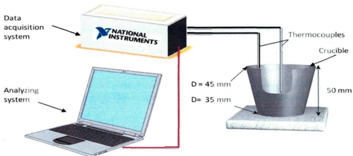
Fig. 3.3 Schematic illustration of the thermal analysis setup.
