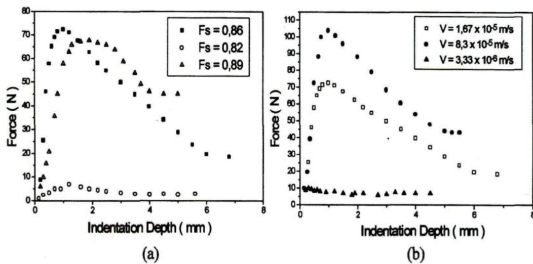
Fig. 2.20 Results of the indentation test for (a) constant penetration speeds and different f_s ; (b) different penetration speeds at f_s = 0.86 [49].
