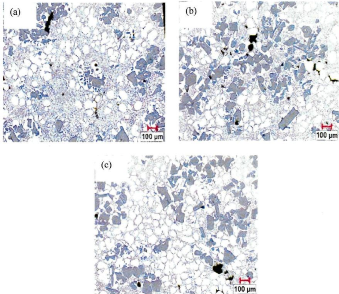
Fig. 4.4 Effect of the amount of addition of solid alloy on the microstructure of A390 slurry, a) 50g (A390), b) 85g (A390), c) 50g (A390) + 42g (A356).
