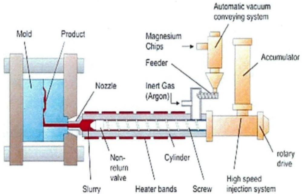
Fig. 2.9 Schematic diagram of a thixomolding machine [25].
