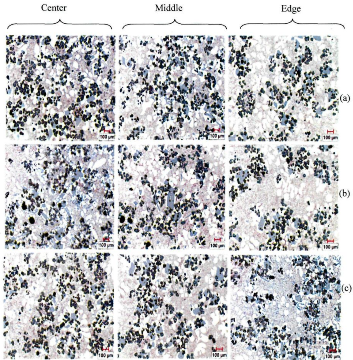
Fig. 7.10 Microstructure of Al-15Si-10.5Mg-4Cu SSM billets from the center to the wall deformed at different solid fractions: (a) at 0.6, (b) 0.5, (c) 0.4.
