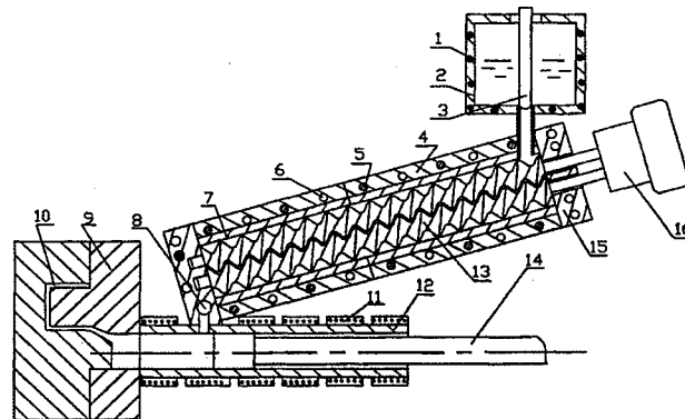
Fig. 2.6 Schematic illustration of the twin-screw rheomoulding process. 1, Heating elements; 2, crucible; 3, stopping rod; 4, barrel; 5, heating elements; 6, cooling channels; 7, barrel liner; 8, transfer valve; 9, die; 10, mould cavity; 11, heating elements; 12, shot sleeve; 13, twin-screw; 14, piston; 15, end cup; 16, driving system [15].
