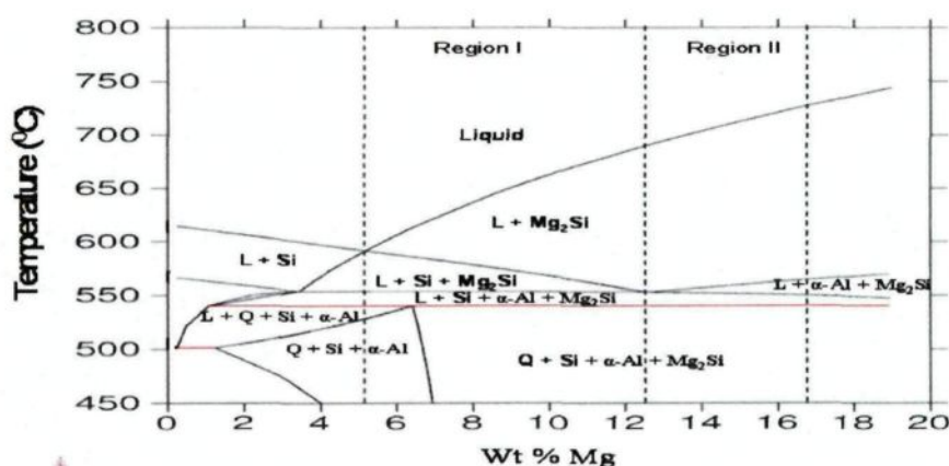
Fig. 6.1: Phase diagram of Al-Si-Cu-Mg system.
