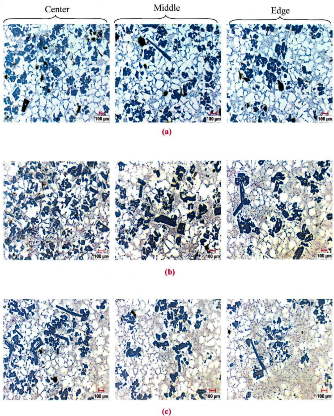
Fig. 7.2 Microstructure of unrefined A390 SSM billets from the center to the edge, deformed at different solid fractions: (a) at 0.6, (b) 0.5, (c) 0.4.
