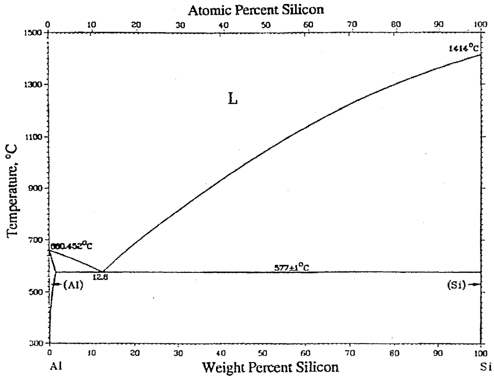
Fig. 2.22: Equilibrium phase diagram of Al-Si system [59].
