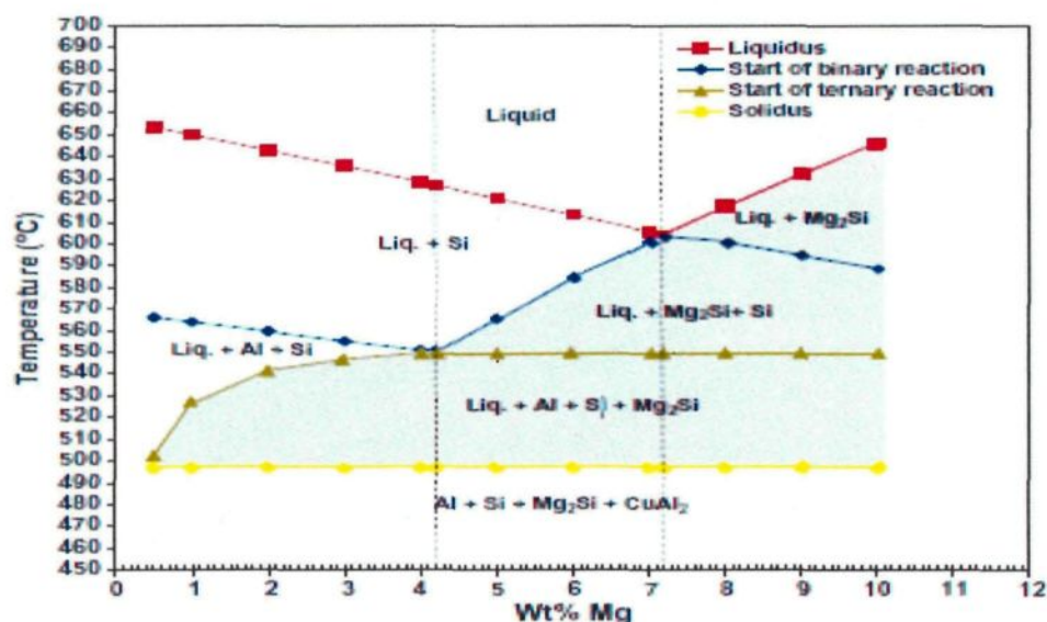
Fig. 2.23 Equilibrium phase diagram of Al-Si-Mg system [74].
