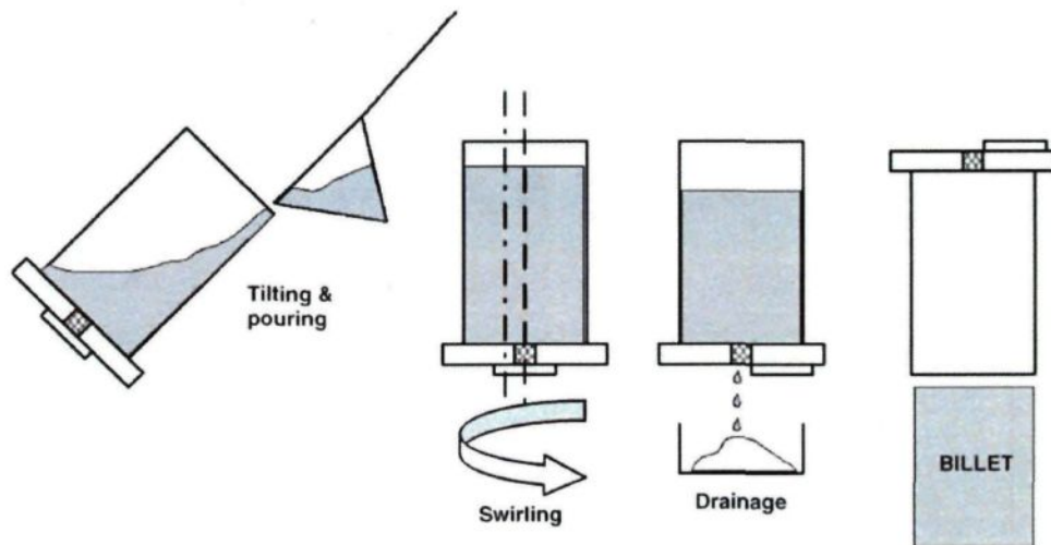
Fig. 2.5 Schematic illustration of the SEED process [14].
