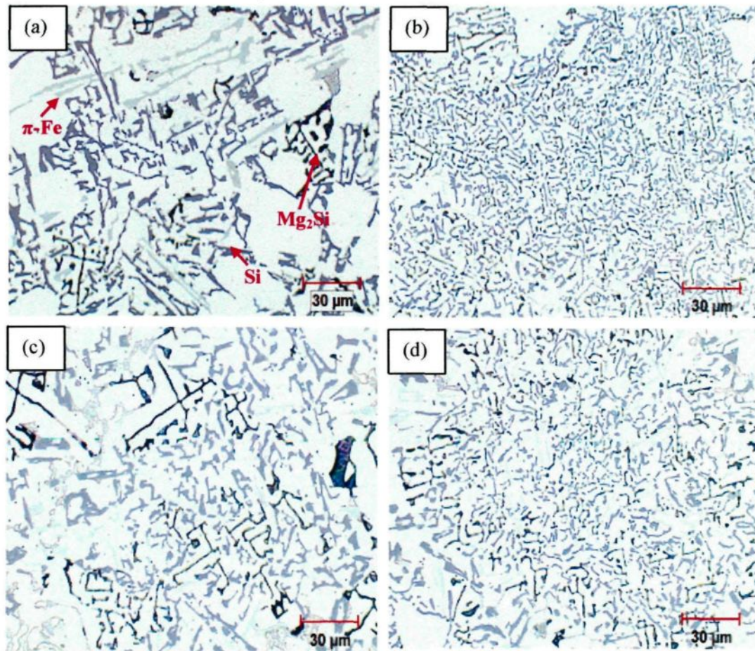
Fig. 6.7: Optical micrographs showing the effect of P and Sr on the eutectic matrix in the (a) unmodified alloy and alloys containing; (b) 0.08 % Sr; (c) 0.4 % P; (d) 0.08 % Sr + 0.4 % P.
