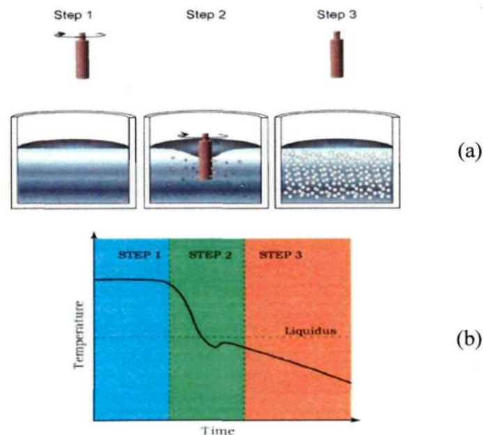
Fig. 2.4 (a) Sequence of steps employed in the « new MIT process »; (b) Melt thermal history [13].
