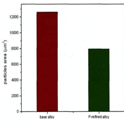
Fig. 7.4 The particles area of primary Si phase as function of phosphorus.
