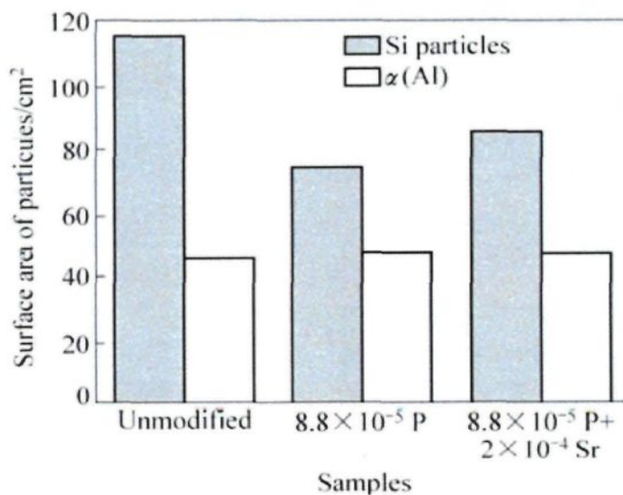
Fig. 4.7 Effect of solid alloy (50 g A390+42 g A356) with P and Sr addition on particle surface area of primary silicon and \alpha (Al).
