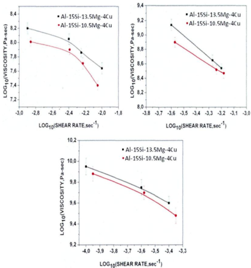
Fig. 7.14 Plots viscosity – shear rate curves of Al-15Si-10.5Mg-4Cu, and Al-15Si-13.5Mg-4Cu alloys with different solid fractions of (a) 40 %, (b) 50 %, (c) 60 %.
