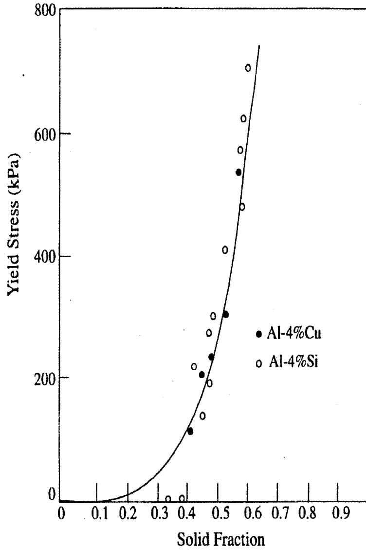
Fig. 2.11 Variation in yield stress under shear with solid fraction for dendritic Al-4%Cu and Al-4%Si alloys [37].
