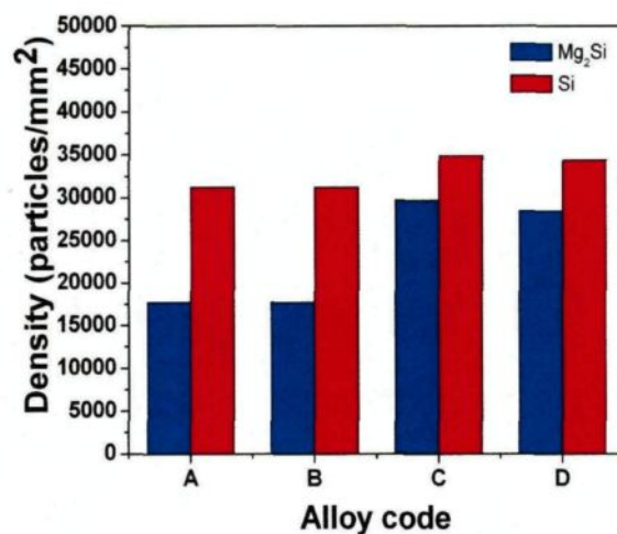
Fig. 6.11: Density of eutectic particles in the alloy A (no addition of P or Sr), alloy B (0.4% P), alloy C (0.08% Sr), and alloy D (0.08% Sr + 0.4% P).
