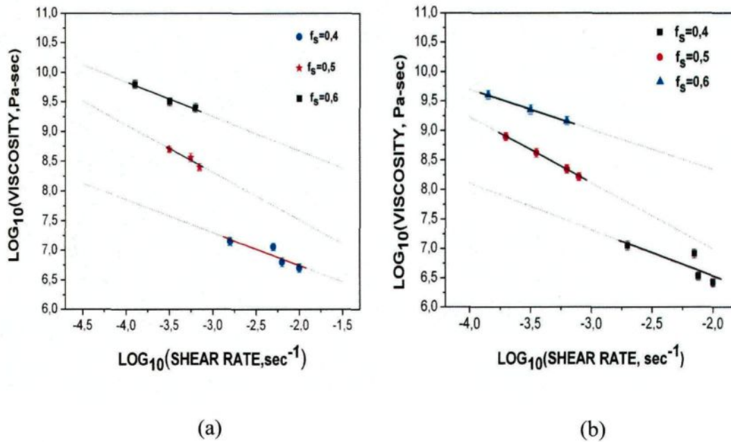
Fig. 7.8 Calculated apparent viscosity against average shear rates for the unrefined and refined A390 alloys, at different initial pressures for each fraction solid: (a) unrefined alloy, (b) P-refined alloy.
