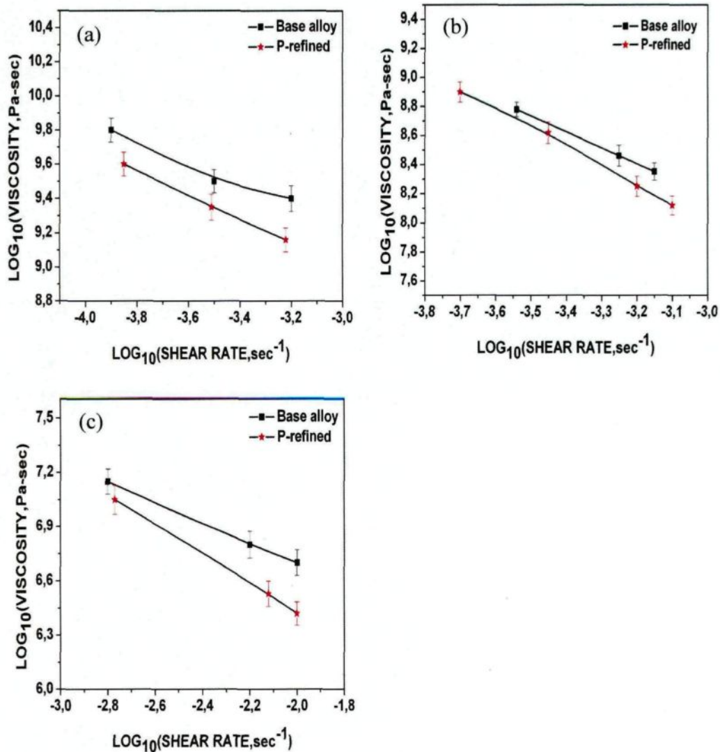
Fig.7.9 Effect of Phosphorus addition on the apparent viscosity of A390 alloy at different temperatures, (a) 552 °C, (b) 558 °C , (c) 560 °C, corresponding to solid fractions of 60 %, 50 %, and 40 % respectively.
