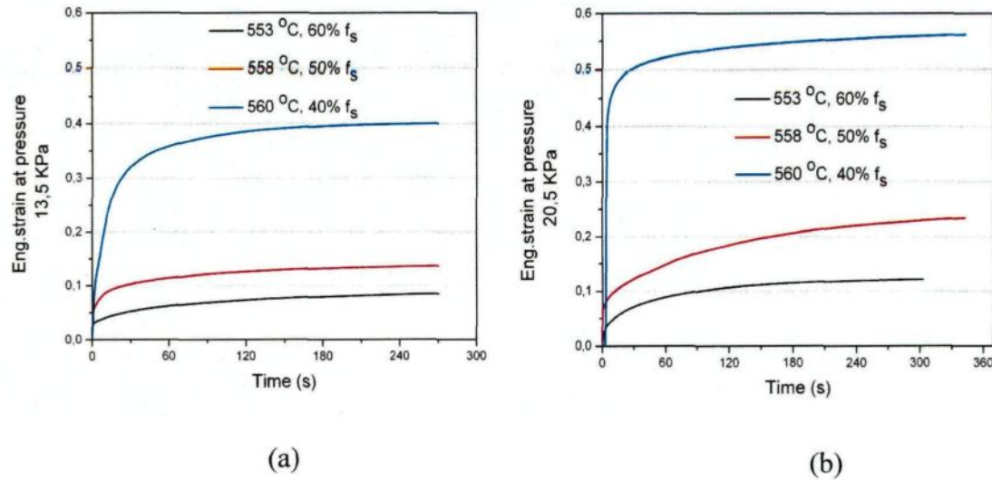
Fig. 7.6 Typical engineering strain-time curves at different temperatures and pressures, (a) 13.5 KPa, (b) 20.5 KPa.
