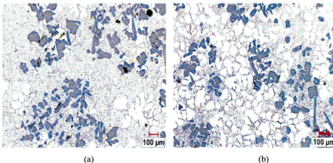
Fig. 4.3 Microstructure of semi-solid A390 obtained using a) conventional SEED process and b) modified SEED process.
