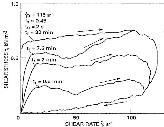
Fig. 2.16 Effect of rest time on hysteresis loops displayed by Sn-15wt.%Pb alloy[42].
