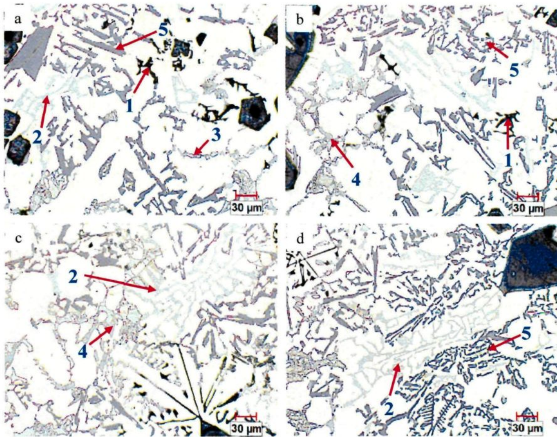
Fig. 5.6 Optical micrographs obtained from the eutectic regions of the four alloys in the as-cast condition: (a) Alloy A, (b) Alloy B, (c) Alloy C, and (d) Alloy D, showing the presence of (1) eutectic Mg_2Si , (2) \pi-Al_8Mg_5FeSi_6 , (3) \theta-Al_2Cu , (4) Q-Al_5Mg_8Cu_2Si_6 , and (5) eutectic Si.
