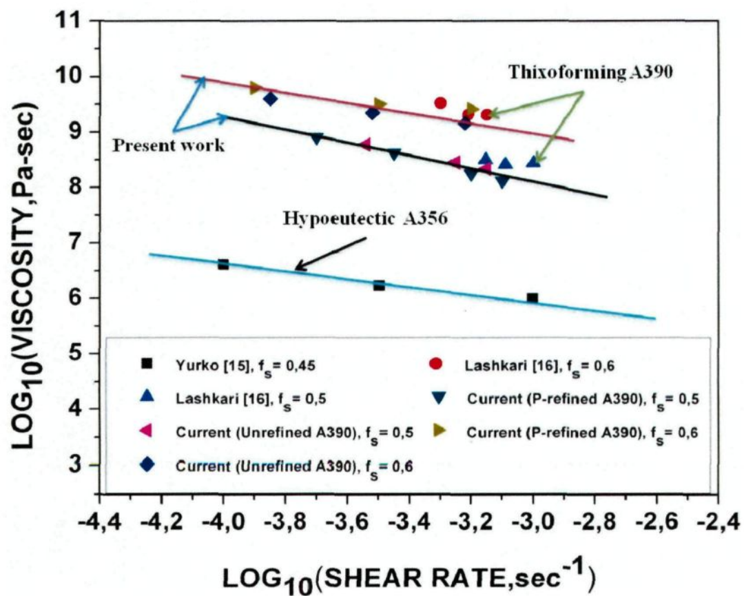
Fig. 7.18 Comparison of the apparent viscosities reported in the literature with the current results.
