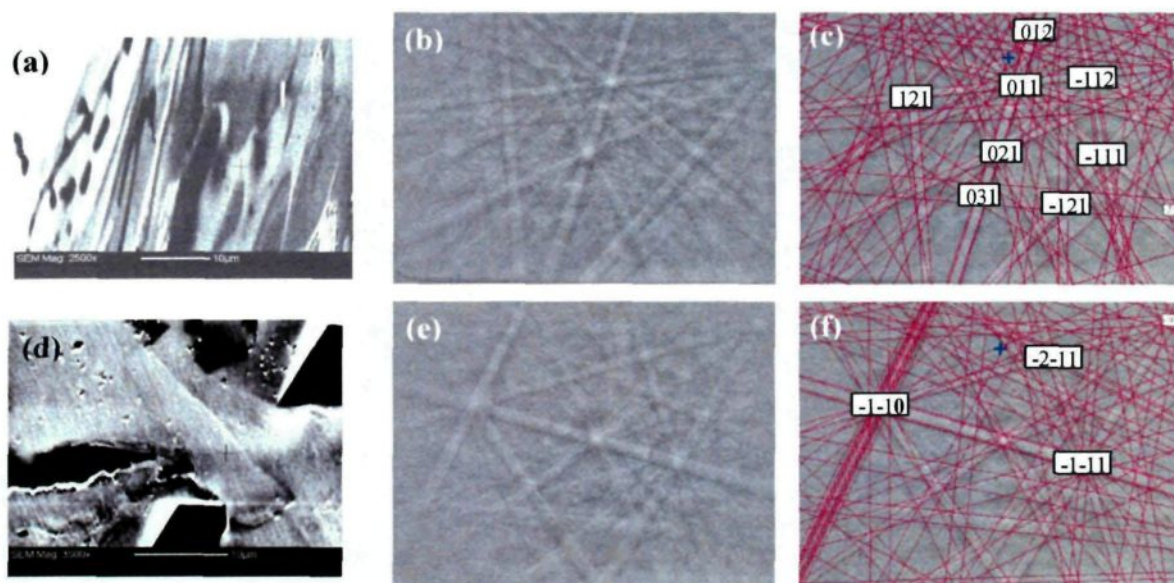
Fig. 6.15 SEM image and representative experimental EBSD patterns with HKL Channel 5 simulations (a-c) unmodified alloy (MAD = 0.209), (d-f) Sr-modified alloy (MAD = 0.201).
