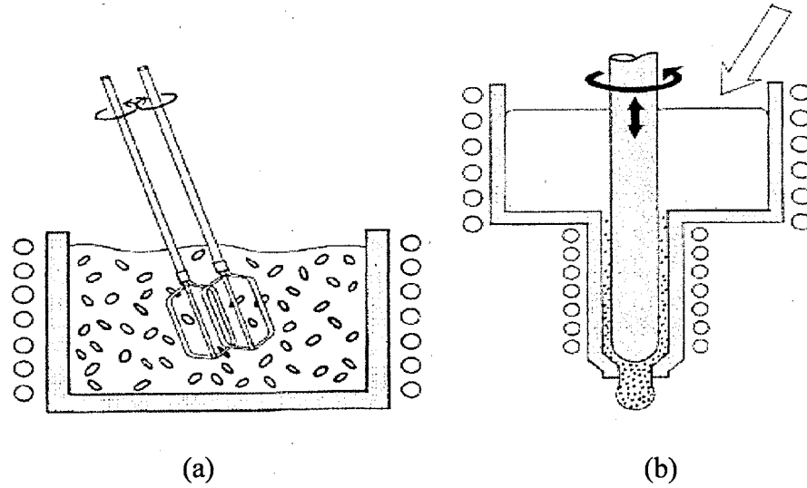
Fig. 2.2 Schematic diagram of apparatus of producing globular structures: (a) batch, (b) continuous [10].
