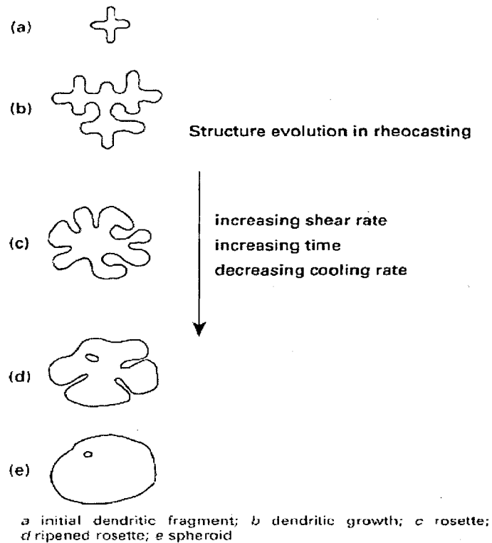
Fig. 2.1 Schematic illustration of structure evolution during solidification with forced convection: (a) initial dendritic fragment, (b) equiaxed dendrite, (c) rosette, (d) ripened rosette, and (e) globule [10].
