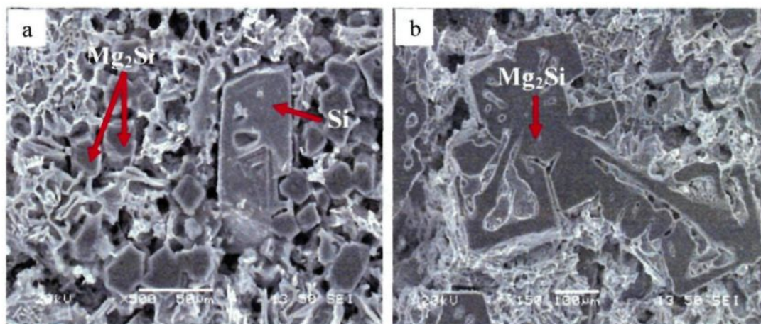
Fig.5.4 SEM micrographs of deeply etched primary Mg_2Si and Si particles in (a) Alloy A, and (b) Alloy C.
