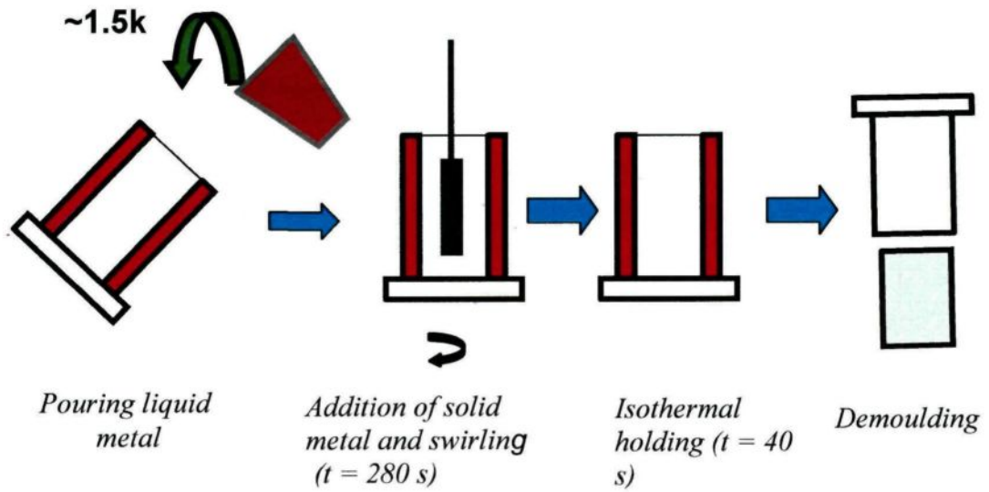
Fig. 3.2 Illustration of the steps involved in the new variation of the SEED rheocasting process.
