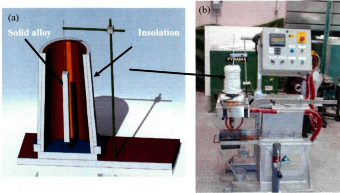
Fig. 3.1 (a) Schematic and (b) an actual overview of new variation of SEED rheocasting process.
