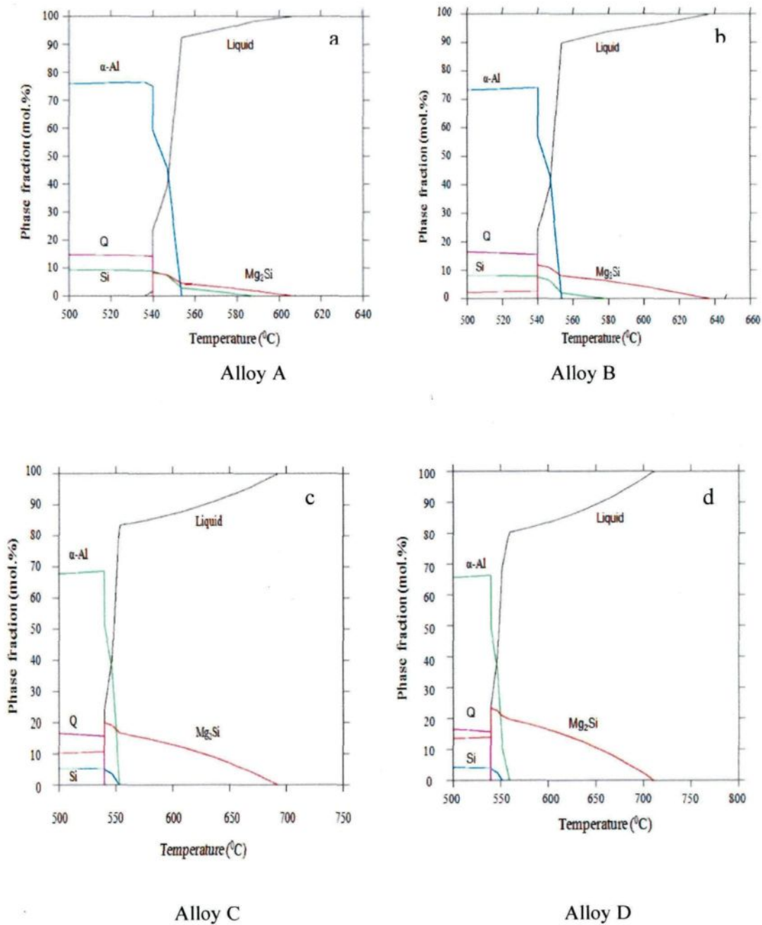
Fig. 5.2 Calculated phase fractions for the four alloys studied, showing the amounts of the phases present under equilibrium conditions, as a function of temperature.
