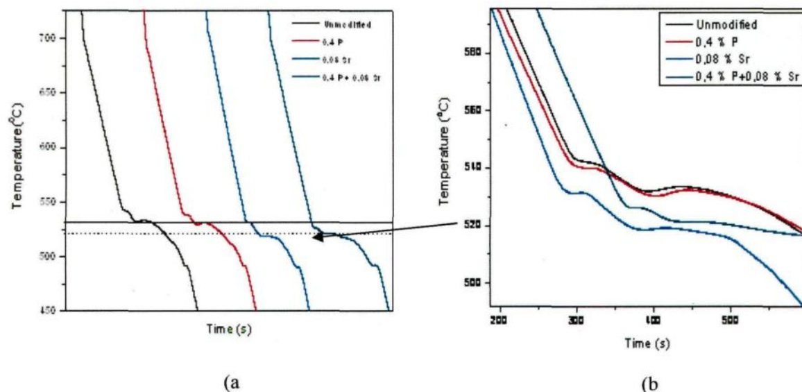
Fig. 6.6: (a) Cooling curves of Al-15Si-14Mg-4Cu alloys, and (b) enlarged image of the arrowed area in (a).
