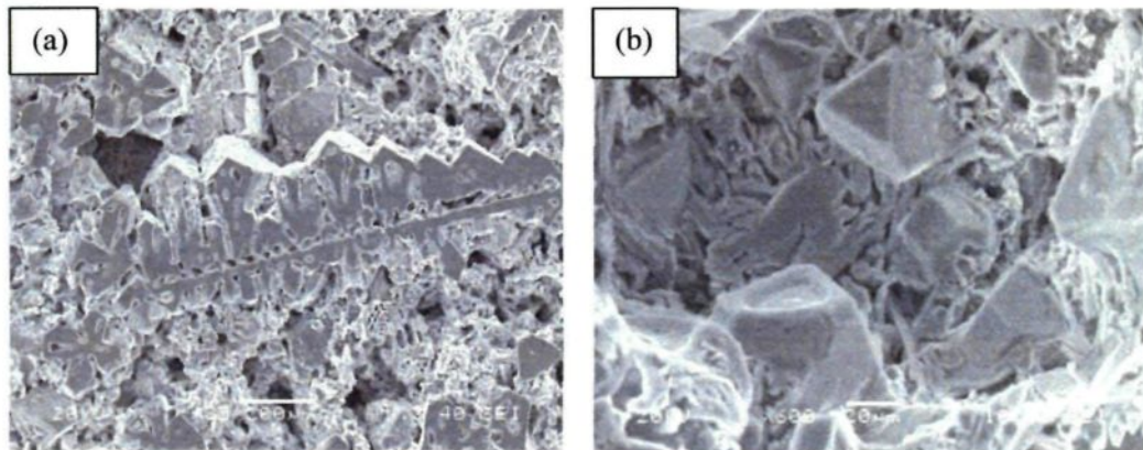
Fig. 6.3: The morphologies of primary Mg_2Si particles (a) unmodified (b) with 0.4% P.
