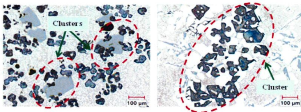
Fig. 7.13 Microstructure of deformed billets showing cluster formation, (a) alloy containing 10.5% Mg and (b) alloy containing 13.5% Mg.
