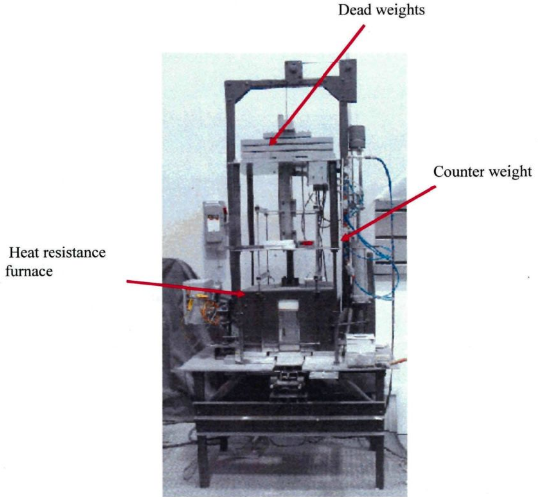
Fig. 3.6 An overview of the parallel plate compression test machine.
