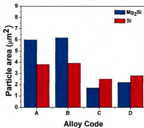
Fig. 6.10: The particle area of eutectic Mg_2Si and Si in the alloy A (no addition of P or Sr), alloy B (0.4% P), alloy C (0.08% Sr), and alloy D (0.08%
