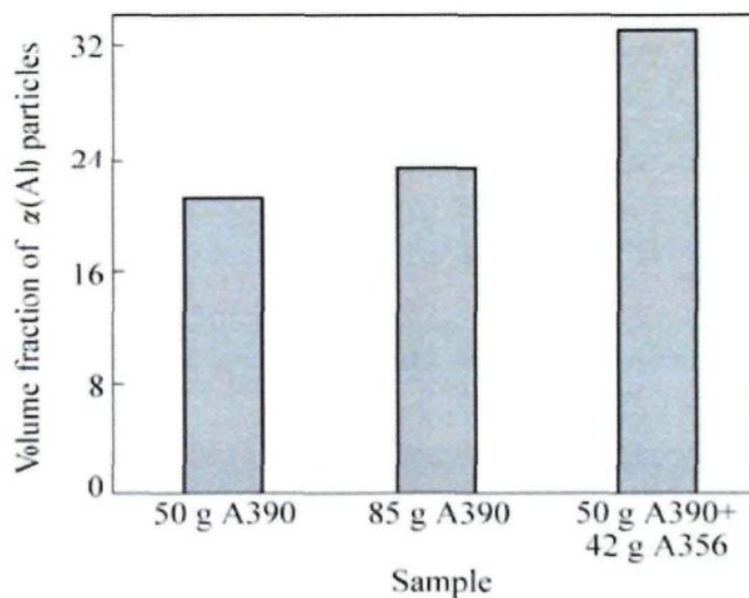
Fig. 4.6 Effect of mass and composition of solid alloy on volume fraction of \alpha (Al) particles.
