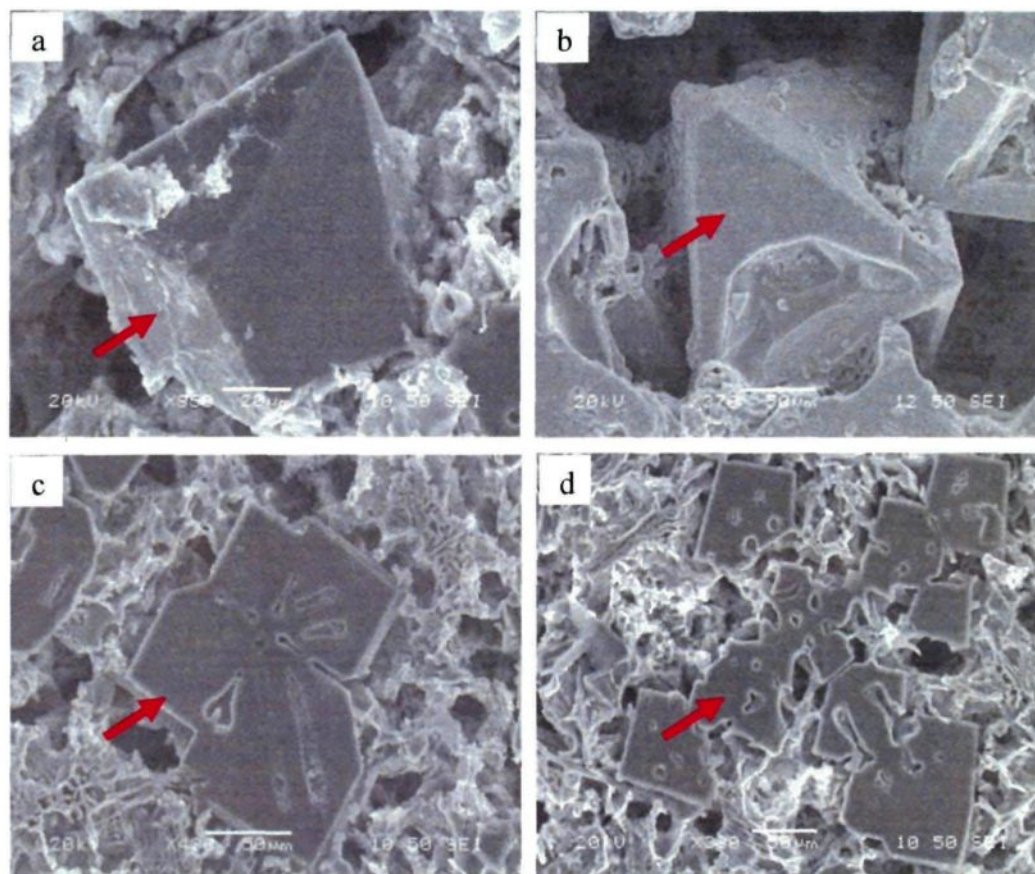
Fig. 5.5 SEM micrographs showing the morphological evolution of Mg_2Si phase with increase in Mg addition: (a) Alloy A, (b) Alloy B, (c) Alloy C, and (d) Alloy D.
