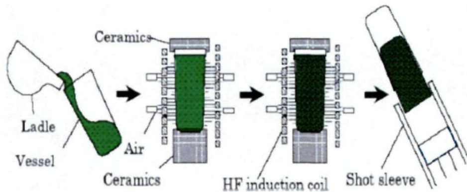
Fig. 2.7 Schematic of the NRC process (Courtesy of UBE Machineries) [16].
