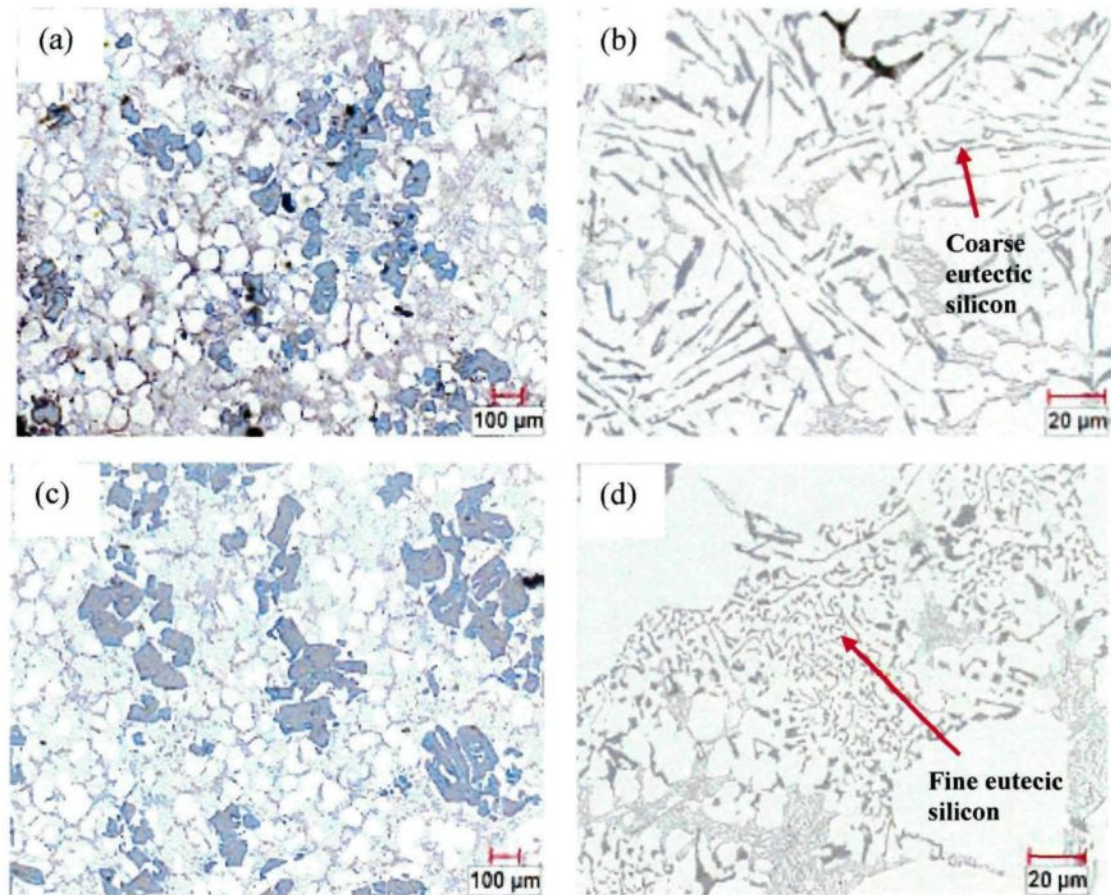
Fig. 4.5 Microstructure of semi-solid A390 with addition of (a) 50 g of A390 alloy + 42 g of A356 alloy of solid metal, (b) with 88ppm P + 0ppm Sr and (c) and (d) with 88ppm P + 200ppm Sr.
