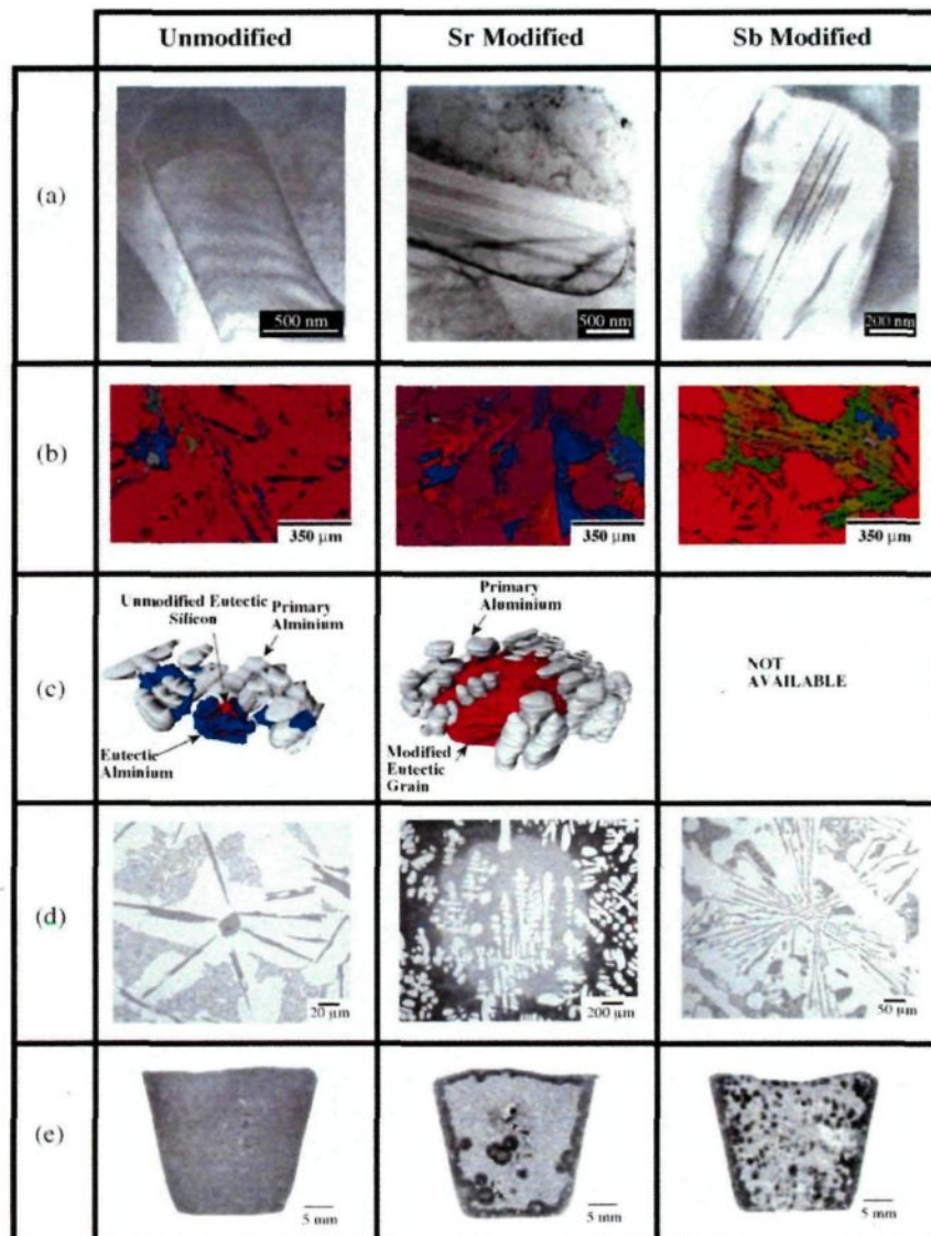
Fig. 2.24 Comparison of unmodified and Sr-modified structures: (a) TEM images of silicon crystals; (b) EBSD maps illustrating the orientation of the eutectic aluminum relative to the primary aluminum dendrites; (c) 3D reconstruction of eutectic grains derived from serial sectioning of quenched samples (the unmodified sample is 85 /in deep, the modified one is 117/in deep); (d) Optical micrographs of quenched samples; and (e) macrographs of quenched samples [77].
