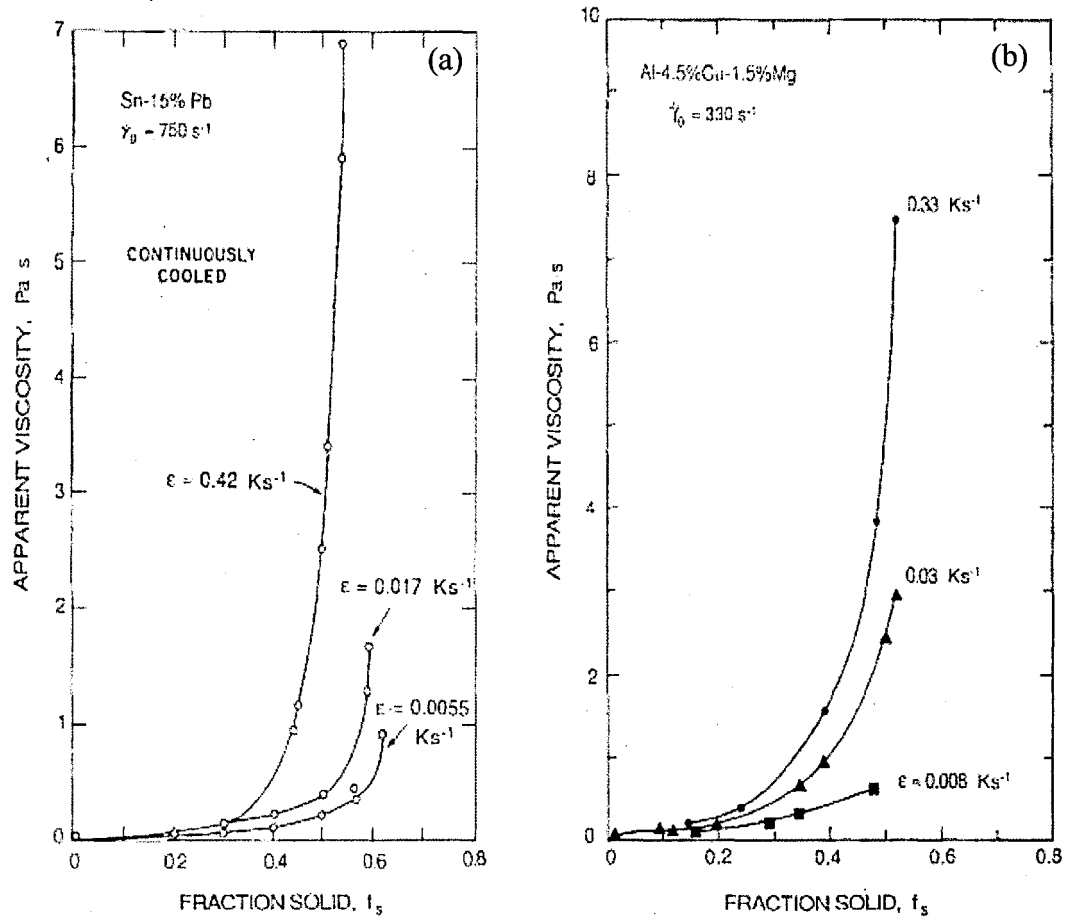
Fig. 2.15 Influence of cooling rate on apparent viscosity of semi-solid alloys: (a) Sn-15wt.%Pb [10], and (b) Al-4.5wt.%Cu-1.5 wt.%Mg [44].
