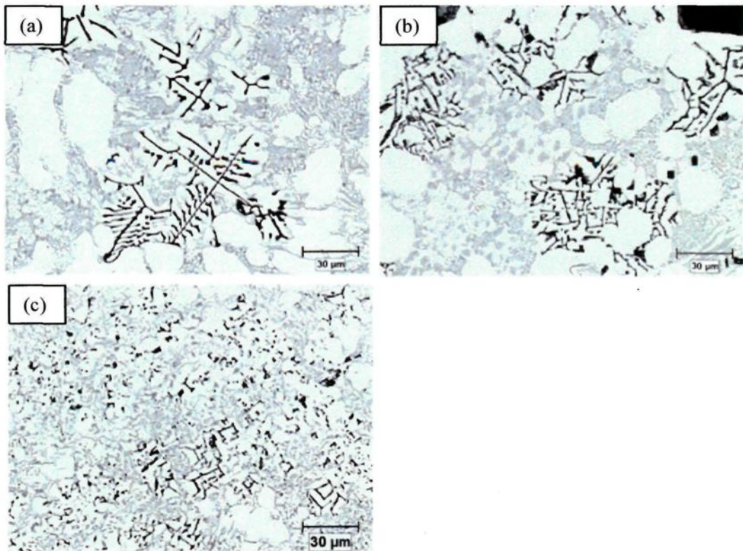
Fig. 6.8: Eutectic Mg_2Si morphologies of Al-15Si-14Mg-4Cu alloy modified with (a) 0 % Sr; (b) 0.04 % Sr; (c) 0.08 % Sr.
