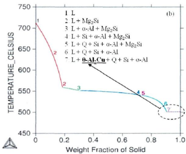
Fig. 5.11 Calculated Scheil solidification paths for (a) Alloy B with 8.4% Mg, and (b) Alloy D with 14.86% Mg.
