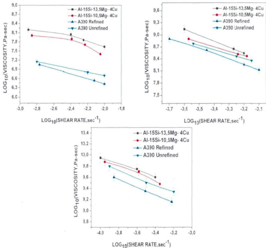
Fig. 7.15 Plots viscosity – shear rate curves of unrefined A390, refined A390, Al-15Si-10.5Mg-4Cu, and Al-15Si-13.5Mg-4Cu alloys with different solid fractions of (a) 40 %, (b) 50 %, (c) 60 %.
