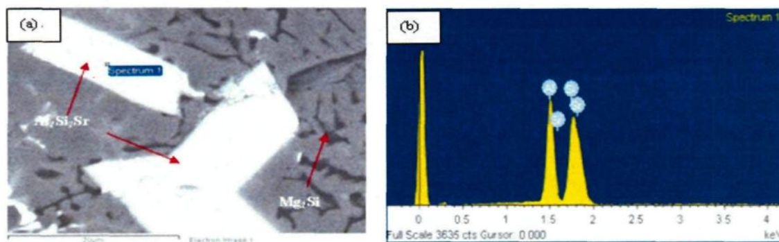
Fig. 6.12 (a) SEM image of the Al_2Si_2Sr intermetallic phase in Sr-modified Al-15Si-14Mg-4Cu alloy and (b) EDX of the Al_2Si_2Sr phase.
