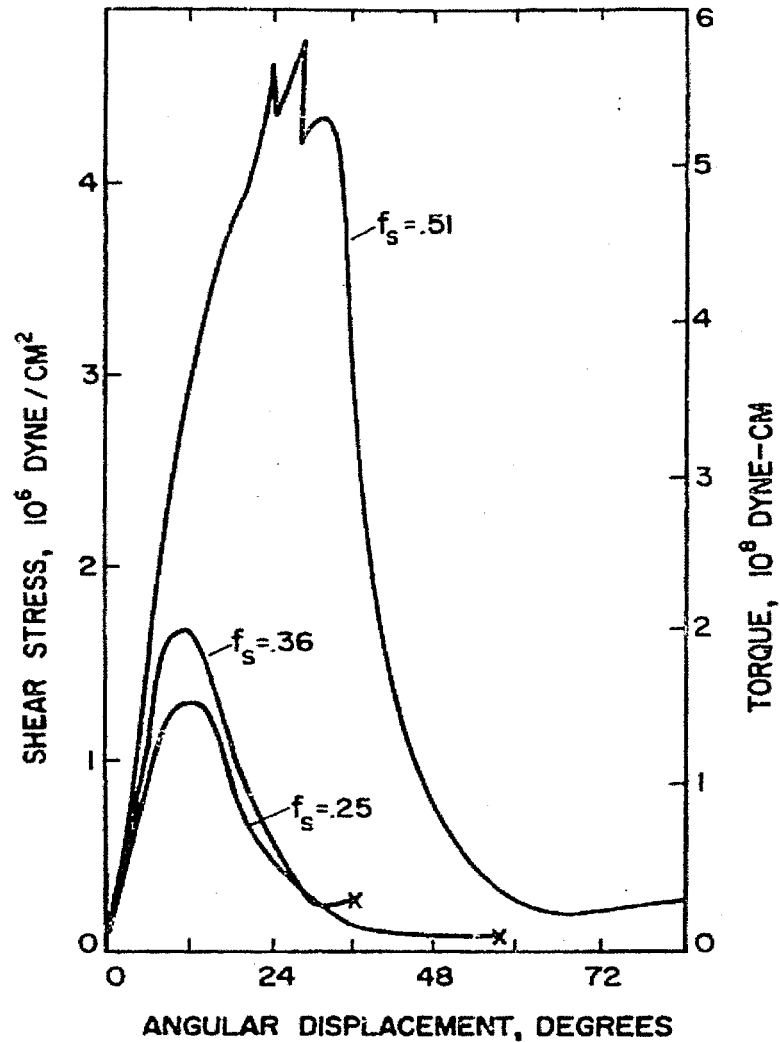
Fig. 2.12 Shear stress and torque versus versus angular displacement for various volume fraction solid values [38].
