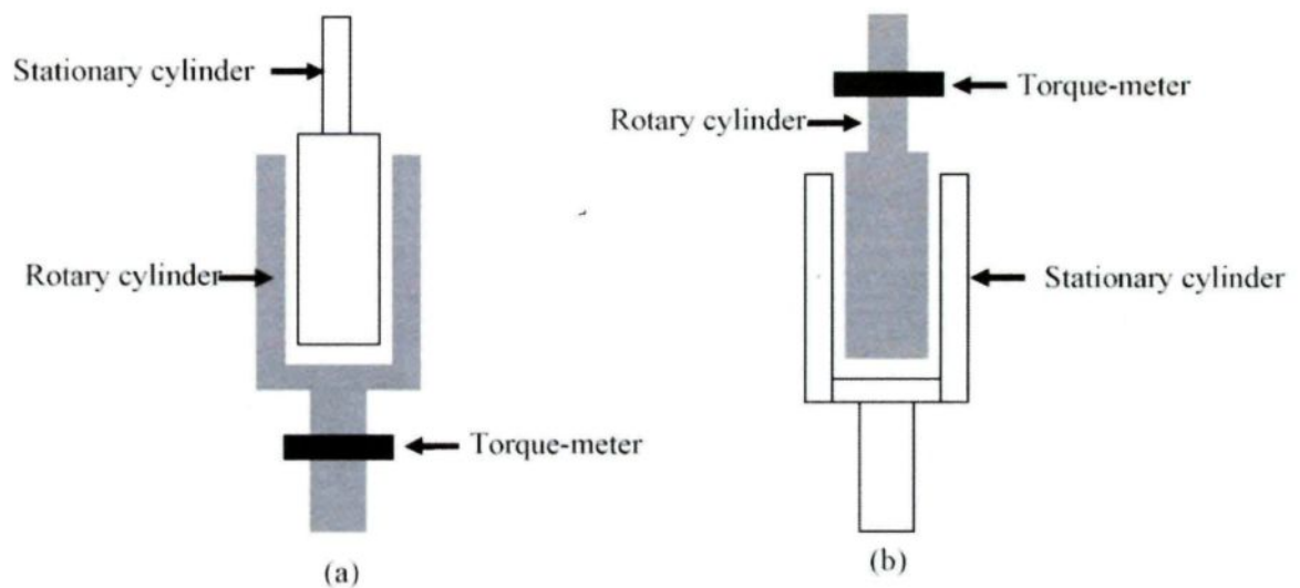
Fig. 2.17 The two types of viscometers (a) Couette and (b) Searle.
