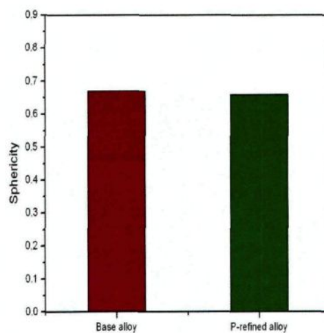
Fig. 7.5 Sphericity of \alpha -Al particles in the unrefined and refined A390 alloys.
