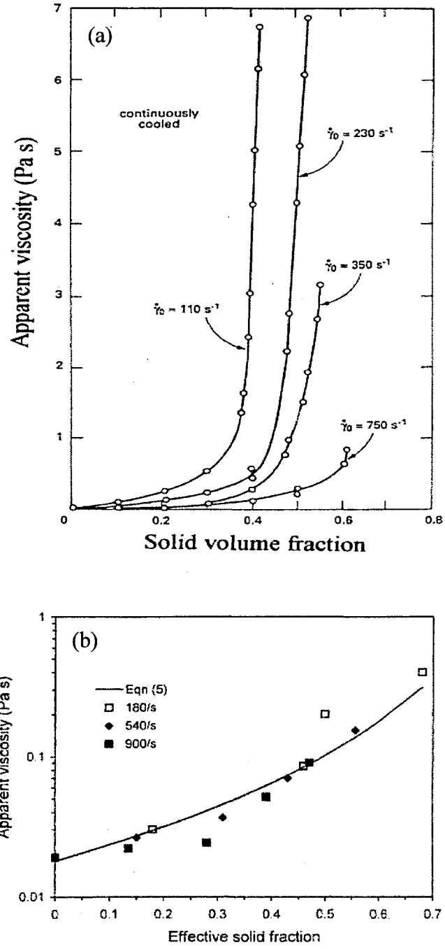
Fig. 2.13 (a) Apparent viscosity as function of fraction solid of Sn-15wt.%Pb sheared continuously and cooled at 0.33 K min -1 [42], (b) apparent viscosity versus effective solid fraction [47].
