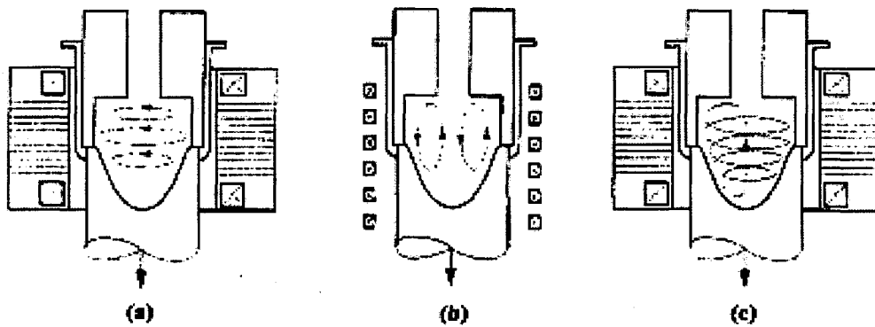
Fig. 2.3 Schematic representation of electromagnetic coils for MHD stirring: (a) Horizontal agitation, (b) Vertical agitation, (c) Helicoidal stirring [12].
