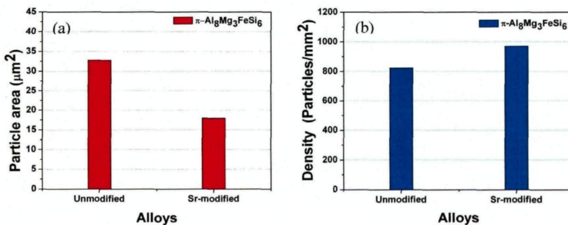
Fig. 6.16 Effect of Sr addition on the (a) particle area of \pi -phase particles, (b) density of \pi -phase particles of Al-15Si-14Mg-4Cu alloy.
