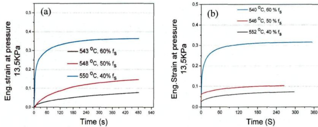
Fig.7.12 Strain-time graphs obtained at different temperatures of (a) Al-15Si-10.5Mg-4Cu alloy, and (b) Al-15Si-13.5Mg-4Cu alloy.
