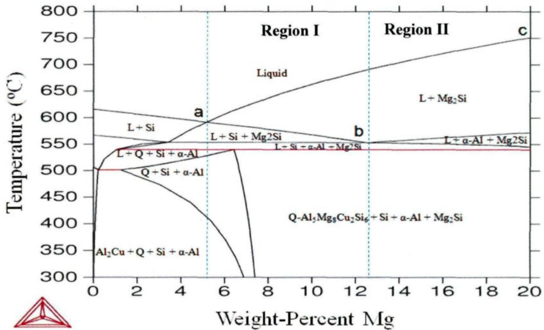
Fig. 5.1 Calculated phase diagram of Al-Si-Cu-Mg system. The dashed lines represent respectively the critical compositions of Al-15Si-4Cu-xMg at 5.16% Mg and 12.5% Mg.
