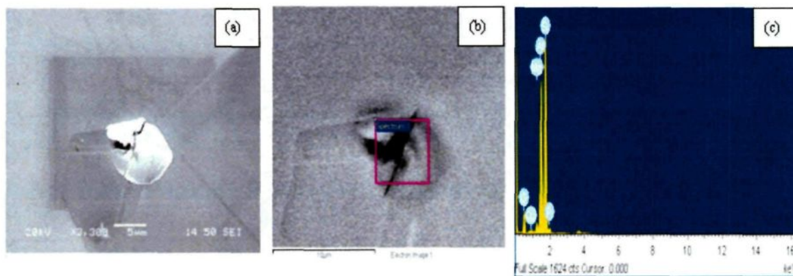
Fig. 6.5: SEM microstructure and EDS analysis of the P-containing phase in the 0.4% P modified alloy: (a) and (b) morphology and (c) EDS of P containing phase.
