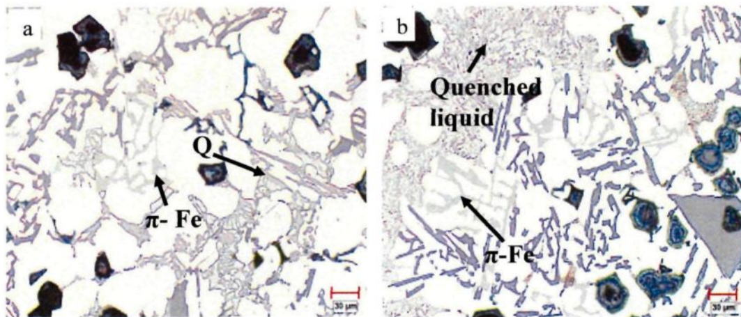
Fig. 5.9 Microstructure of Al-15Si-4Cu-6.15Mg alloy (Alloy A) water quenched at different temperatures (a) at 510 °C, (b) between 528 °C and 520 °C.
