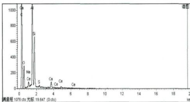
Figure 4.16. EDS patterns of the Ce element in carbon anode A
