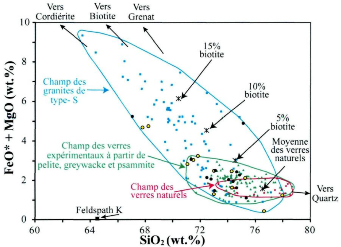
Figure 5.3: Diagramme \text{SiO}_2 vs \text{FeO}^* + \text{MgO}
