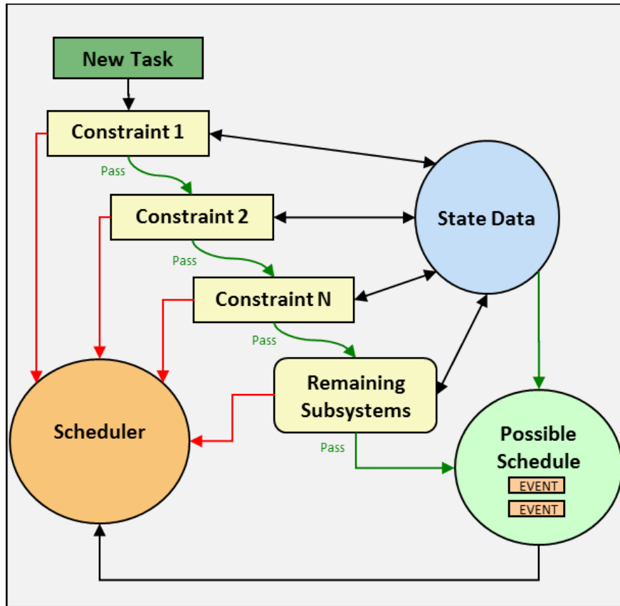
Figure 4: Constraint Cascade
