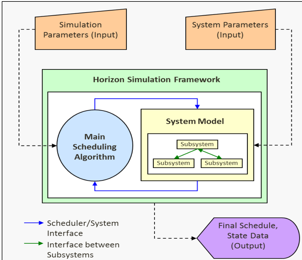
Figure 2: HSF Structure 14
