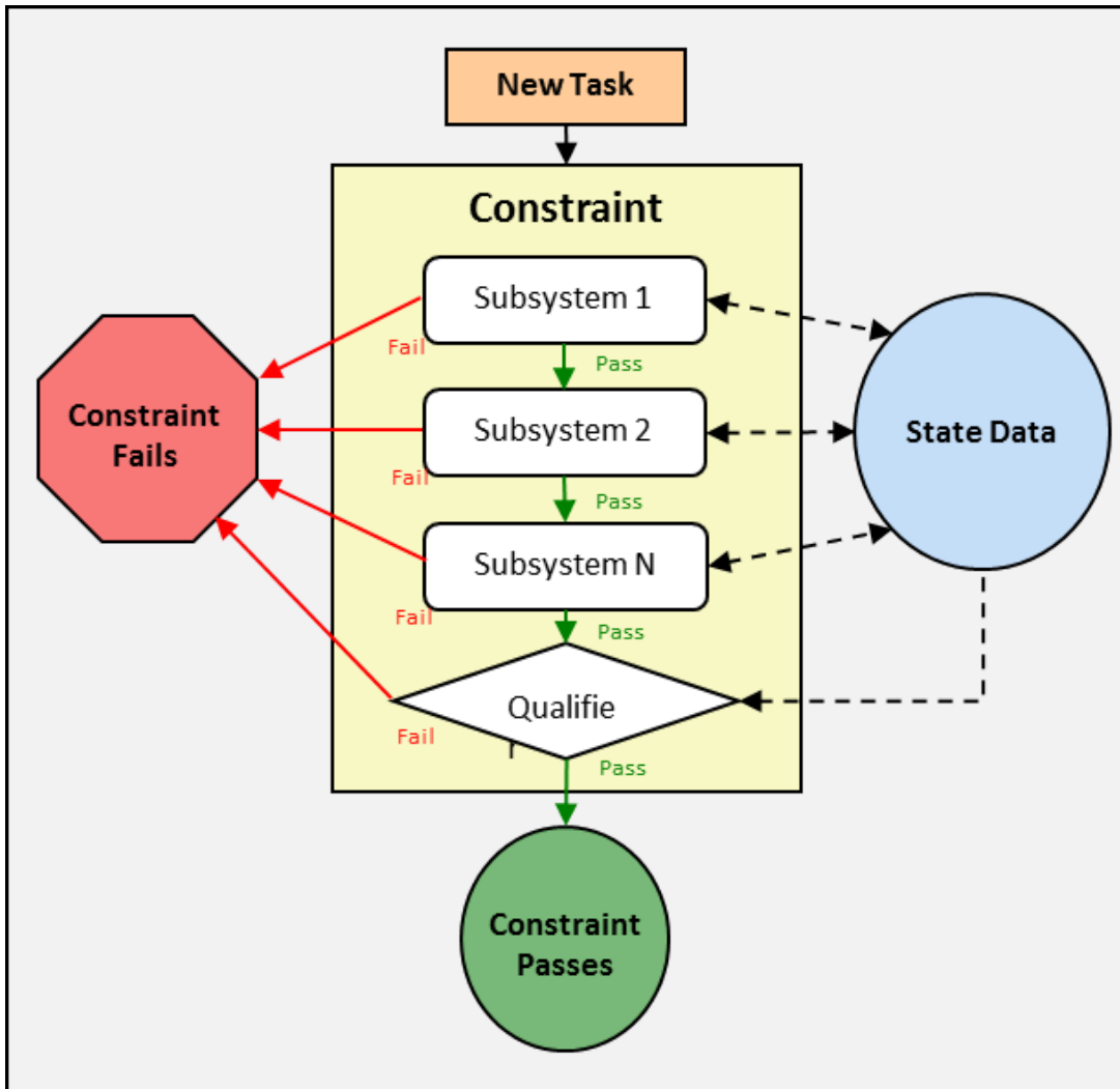
Figure 3: Subsystem Checking
