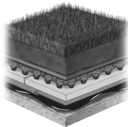
Figure 1: Section of a typical green roof. The insulation layer is optional. Source: American Hydrotech, Inc.
