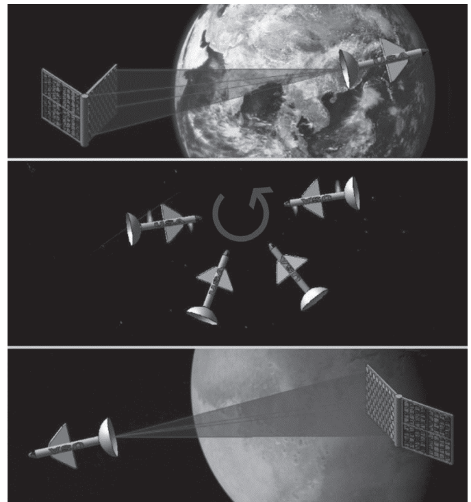
Fig. 16 A second DE-STAR photon drive at the mission destination can decelerated the spacecraft under controlled conditions. This deceleration is achieved by a “ping-pong” method where the spacecraft rotates and first one DE-STAR and then the second provide opposing forces to the reflector.
