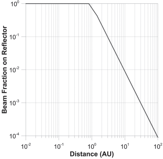
Fig. 7 Plot of beam fraction on reflector (D_s/D)^2 versus distance for the case of a craft with a 30 m reflector being illuminated by a DE-STAR 4 array. (D_s/D)^2 is the fraction of laser power intercepted by the reflector. After approximately 1 AU (or \sim 3 days for the case of a 100 kg craft) the laser spot size exceeds the size of the reflector at which point the fraction of the beam intercepted by the reflector decreases. This plot is the same independent of the mass of the craft but the time to a given distance changes.
