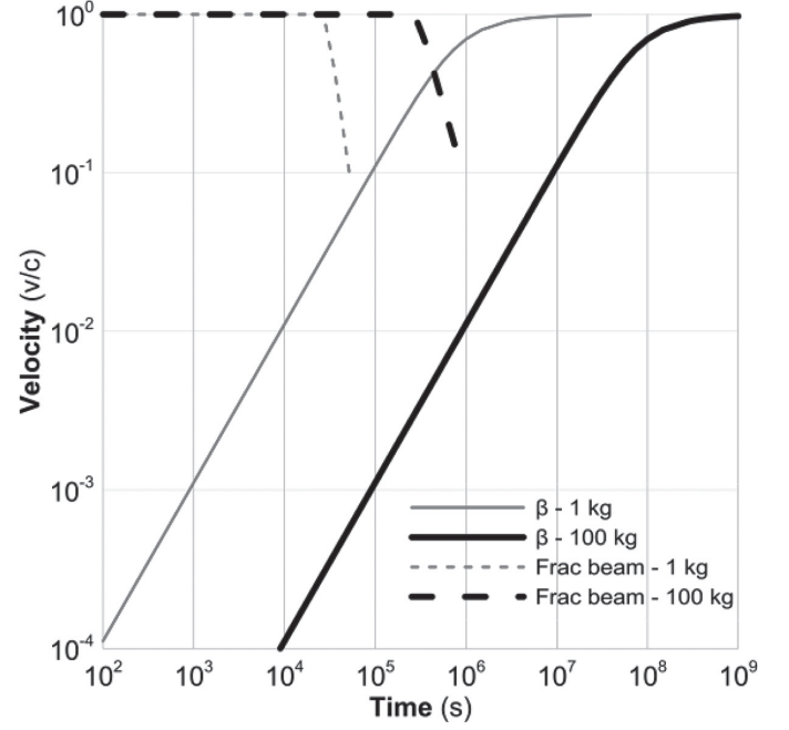
Fig. 3 Speed versus time using the inverted equation for time (7), for both a m_0 = 1 and 100 kg spacecraft+sail, P_0 = 50 GW (DE-STAR 4) with \varepsilon_r = 1 . The speed assumes the reflector is large enough to accommodate the beam divergence but the beam fraction refers to a 30 m diameter sail. The 100 mg case assumes a 10 micron thick sail that has a mass of 9 kg while the 1 kg case assume a 1 micron thick sail that has a mass of about 1 kg. As the speed increases, the spacecraft begins to display relativistic effects as is readily seen. The 1 kg system achieves about 5% c in about 10 hours while the 100 kg system achieves about 0.6% c in about 6 days again both with a 30 m sail.
