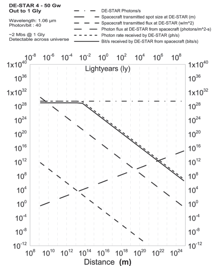
Fig. 11 Communications or searches between two civilizations with DE-STAR 4 units at each civilization vs distance out to 1 Gly. The conclusion is that we would get an equivalent bit rate at 1 Gly of about 2 Mbps. This implies that this “modest” technology that we have now advanced to envisioning implies that civilizations across the entire universe could send high speed information to each other modulo the time of flight. The implications for SETI searches are profound.
