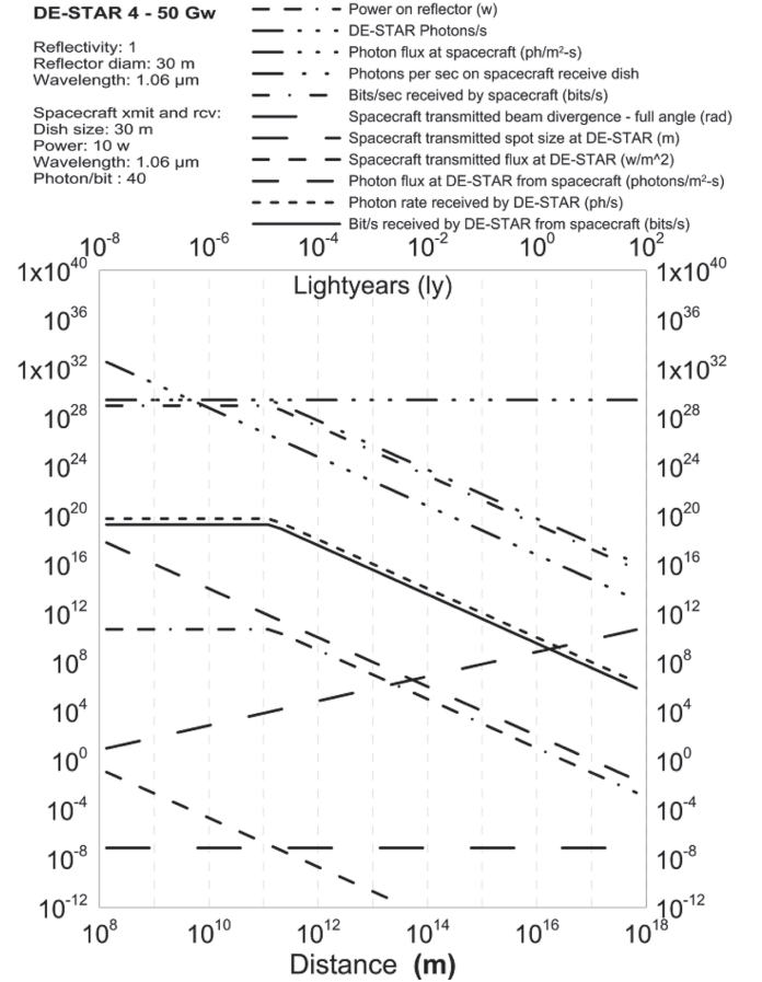
Fig. 10 Communications parameters between a DE-STAR 4 and a small robotic spacecraft vs. distance to spacecraft. The spacecraft is assumed to have a 10 watt burst mode (hibernates most of the time) IR transmitter and uses a 30 m reflector as both the drive and the transmit/receive reflector. Both uplink (DE-STAR to spacecraft) and downlink (spacecraft to DE-STAR) are shown.
