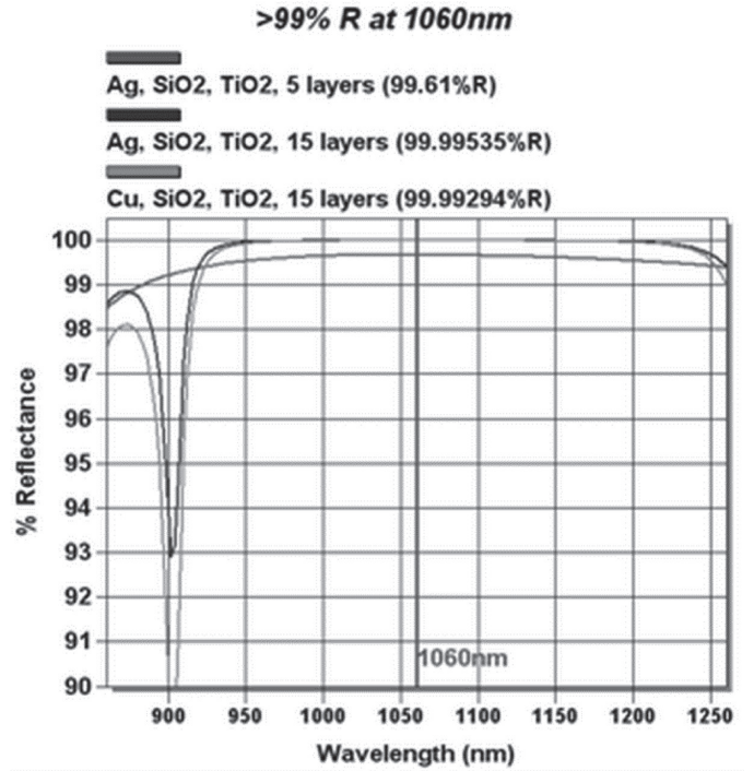
Fig. 9 Graph of the percent reflectance for a practical thin film roll to roll reflector design. The green line of 1,060 nm corresponds to DE-STAR’s laser wavelength. (Source: figure and data from Surface Optics - private communications (2013)). Reflectivities in excess of 99.995% are achievable now on thin film plastics and with further refinements 99.999% looks feasible.
