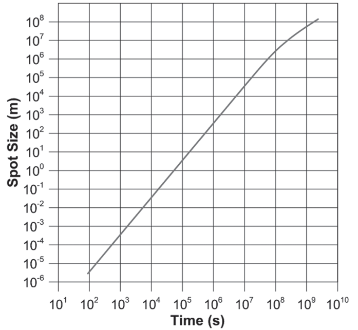
Fig. 5 Plot of DE-STAR spot size (reflector size required) with respect to time for the 100 kg craft case. This assumes the reflector is illuminated fully the entire time.
