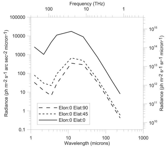
Fig. 13 Zodiacal emission from the COBE DIRBE measurements showing day 100 of the COBE mission at observation from the along the ecliptic plane to 45^\circ to 90^\circ (ecliptic pole). William Reach private communication (2012). Note the radiated peak from solar system dust around 15 \mu\text{m} due to the dust temperature being about 200 \text{ K} and the scattered rise near 1 \mu\text{m} due to the zodi dust scattered sunlight.
