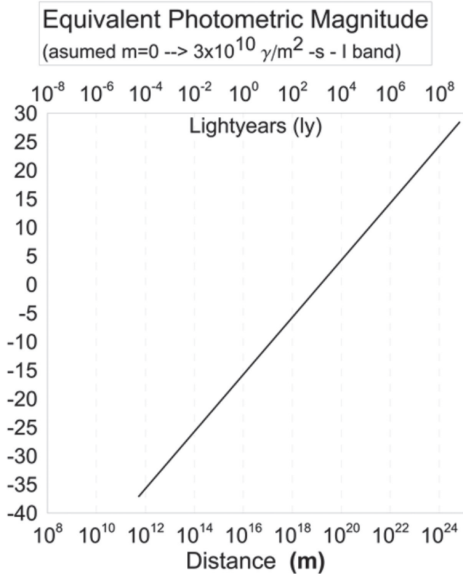
Fig. 12 Photometric (broad band equivalent) magnitude vs distance for a DE-STAR 4 out to 1 Gly. The I band equivalent photometric magnitude at 1 Gly from a DE-STAR 4 is approximate m = 30 or roughly the limit of the HST.
