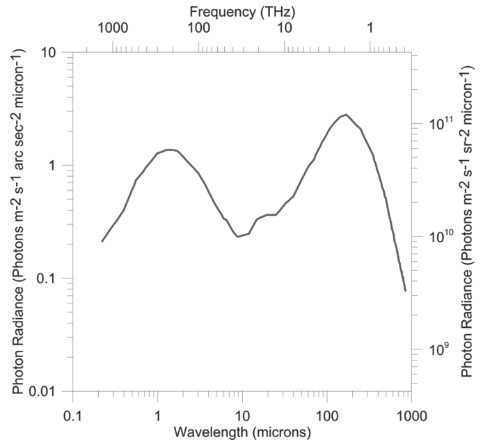
Fig. 14 Cosmic Infrared Background (CIB) radiation from COBE DIRBE and subsequent measurements.
