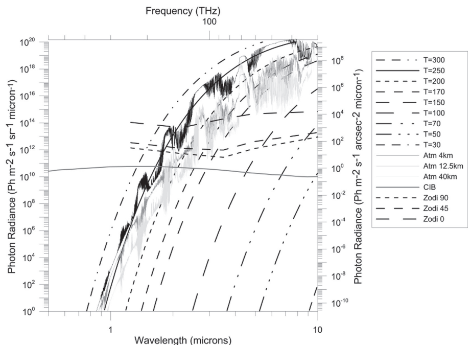
Fig. 15 Comparison of optical emission vs optics temperature assuming emissivity is unity, atmospheric emission for various altitudes, Cosmic Infrared Background and Zodiacal light at various ecliptic inclinations (day 100 from COBE) vs wavelength for 0.5 to 10 \mu\text{m} . Note the left hand and right hand vertical axes are reversed compared to Figs. 13 and 14. The bottom line is that at 1 \mu\text{m} ; the optical emission is small compared to the Zodi and CIB.
