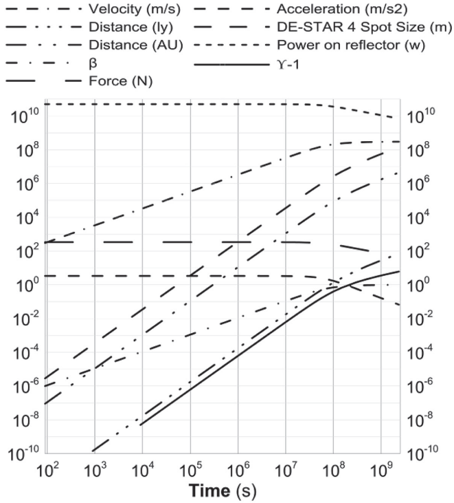
Fig. 8 Numerical solution to relativistic equation of motion for 100 kg rest mass with a reflector that is assumed to grow as large as is needed to intercept the full beam and a DE-STAR 4 - 50 GW drive. As discussed the case of a fixed reflector of 30 m diameter that is reasonable for a 100 kg craft will only reach about 3% the speed of light and then coast. The decrease of power on the reflector is from relativistic effects. See Fig. 9.
