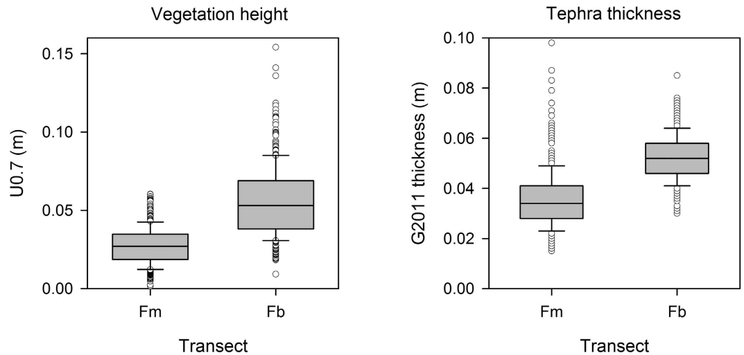
Figure 2. Vegetation height (left) and tephra thickness measurements for each transect.
