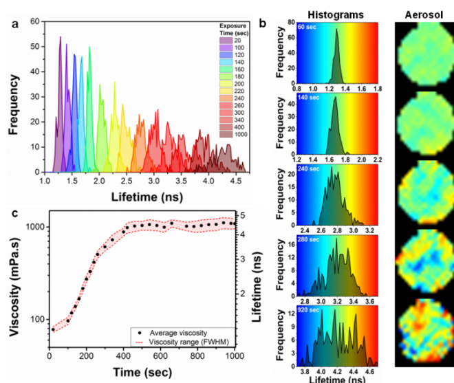
Fig. 5 Development of oleic acid droplet heterogeneity with exposure to ozone. a) Lifetime histograms recorded for an individual droplet (69.4 \mu\text{m} diameter) upon exposure to 377 ppm of ozone for 1000 sec. b) Selected histograms from (a) are shown next to their images, plotted against a rainbow colour hue of 1 ns width (same increment). c) The increasing average viscosity (●) and a viscosity spread indicating heterogeneity (---) during ozone exposure; Gaussian fit of histograms in (a) provided peak centres as average viscosity values and the FWHM of histograms provided the spread.
