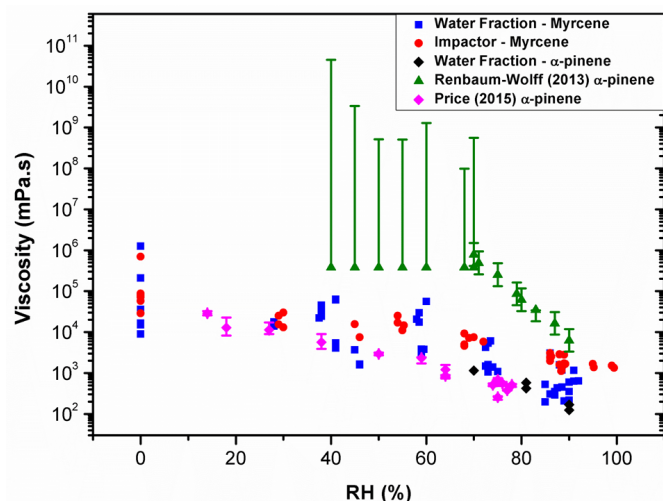
Fig. 2: Measuring viscosity of oxidised SOA during RH change using various techniques. The data recorded in this study for myrcene (■ •) and \alpha -pinene (◆), compared to the data in Renbaum-Wolff 10 and Price 12 (converted into inferred microviscosity values using the Stokes-Einstein relation) for the water-extracted \alpha -pinene. The viscosities measured in this work of \alpha -pinene-SOA are very close to those for myrcene SOA. While viscosities derived from water diffusion measurements 12 agree well with the values measured in this work, bulk techniques such as 10 determine significantly higher viscosities.
