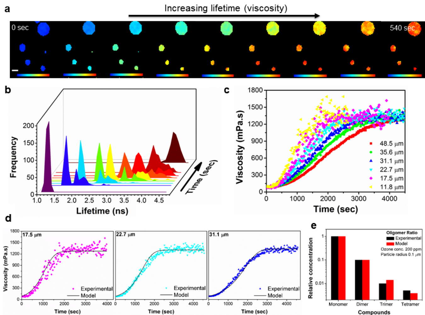
Fig. 4: Time-dependent FLIM imaging of oleic acid droplets of varied diameter upon exposure to ozone. a) FLIM images recorded at 0, 120, 160, 200, 220, 260, 300, 360 and 540 sec after the beginning of exposure to 377 ppm of O_3 ; rainbow scale under each image represents the lifetime values from 1 to 4.8 ns and scale bar is 40 \mu m . The high concentration of O_3 was chosen to optimise the experimental running time, however, the observations remain the same for O_3 concentrations down to 1.5 ppm. b) Lifetime histograms extracted from the images in (a). c) Kinetic response of the individual droplet viscosity to exposure to 12.5 ppm of O_3 for various droplet sizes. The lifetime recorded in the absence of ozone (Fig. S7) does not change on this timescale. d) Selected traces from (c) plotted together with simulated viscosity curves obtained using the KM-SUB model (see Supplementary Information for further details). e) Experimental monomer : dimer : trimer : tetramer signal intensities normalized to the signal intensity of the sum of all major monomers obtained from a fully oxidised sample using mass spectrometry are shown along with concentration ratios obtained in a corresponding model simulation (see also Fig. S8).
