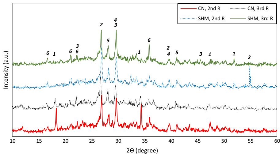
Fig. 12. XRD of the healing products after 2nd round and 3rd round of cracking [1: \text{Ca}(\text{OH})_2 ; 2: \text{SiO}_2 ; 3: \text{CaCO}_3 ; 4: C–S–H; 5: \text{C}_3\text{S}/\text{C}_2\text{S} ; 6: \text{Ca}_6\text{Al}_2(\text{SO}_4)_3 (\text{OH})_{12} \cdot 26 \text{H}_2\text{O} ].
