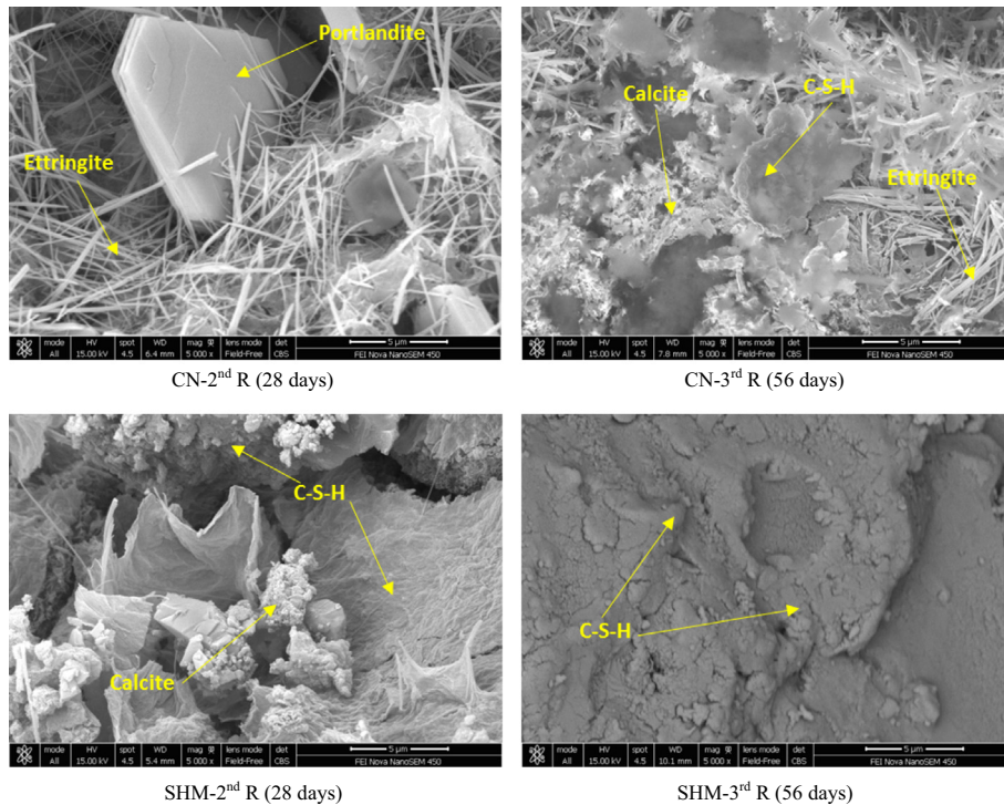
Fig. 14. BSEM images of healing products at crack surfaces.
