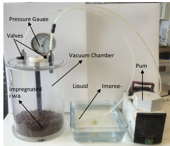
Fig. 1. Vacuum impregnation set-up.
