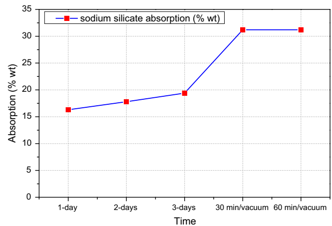
Fig. 2. Sodium silicate absorption of the lightweight aggregates.
