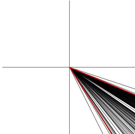
FIGURE 3. The supports of all the walls (\mathfrak{d}, f_{\mathfrak{d}}) in \mathfrak{D}_{(3,2)} such that f_{\mathfrak{d}} \not\equiv 1 \pmod{\mathfrak{m}^{100}} ; the boundary rays of the irrational cone are highlighted.
