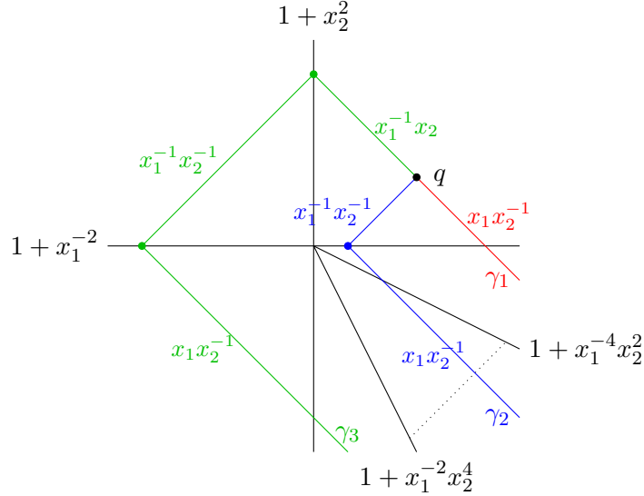
FIGURE 4. The scattering diagram \mathfrak{D}_{(2,2)} and the broken lines described in Example 3.8.
