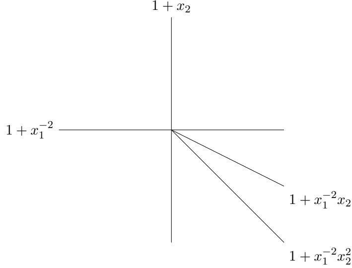
FIGURE 2. The scattering diagram \mathfrak{D}_{(2,1)} . Since the initial diagram \mathfrak{D}_{\text{in},(2,1)} consists of the walls (\mathbb{R}(-1,0), 1 + x_1^{-2}) and (\mathbb{R}(0,1), 1 + x_2) , the associated consistent scattering diagram \mathfrak{D}_{(2,1)} contains \mathfrak{D}_{\text{in},(2,1)} together with the two walls (\mathbb{R}_{\leq 0}(-1,1), 1 + x_1^{-2}x_2^2) and (\mathbb{R}_{\leq 0}(-2,1), 1 + x_1^{-2}x_2) .
