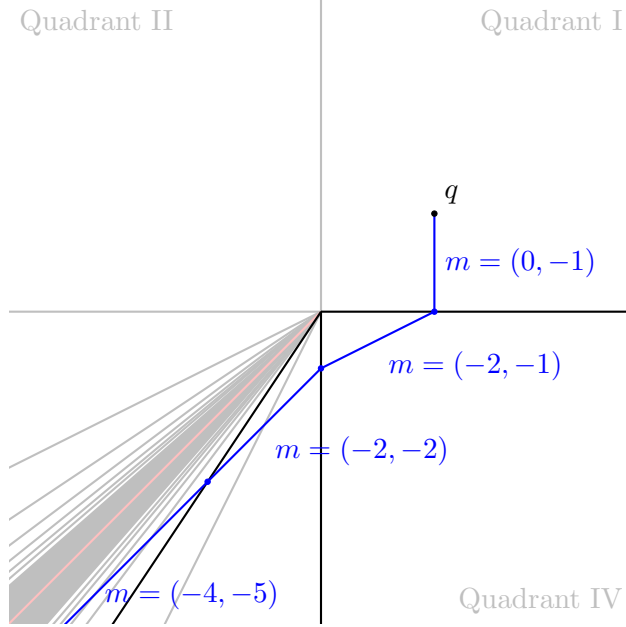
FIGURE 6. A broken line with positive angular momentum
