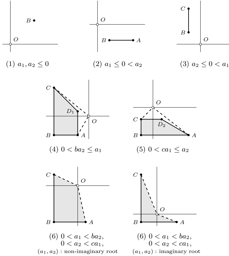
FIGURE 1. Consider the points O = (0, 0) , A = (-a_1 + ba_2, -a_2) , B = (-a_1, -a_2) , C = (-a_1, -a_2 + ca_1) , D_1 = (-a_1 + ba_2, ca_1 - (bc + 1)a_2) , and D_2 = (ba_2 - (bc + 1)a_1, -a_2 + ca_1) . Then the support region of x[a_1, a_2] can be visualized as above.
