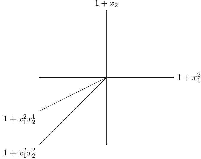
FIGURE 5. The scattering diagram \mathfrak{D}_{(2,1)}^{\mathbf{d}} .
