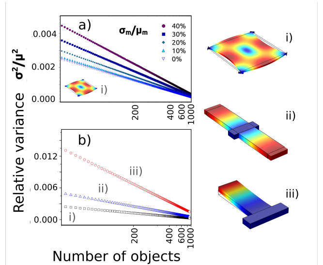
FIG. 2: Relative variance as a function of the number of objects on the sensor (see Eq. (5)). a) Effect of stochastic processes in the sensing environment. Graph showing the relative variance as function of the inverse of the number of objects for a square resonator excited in Lamé mode. The relative variance increases with the coefficient of variation ( c_v = \sigma_m/\mu_m ) which represents the ratio of the width of the mass distribution to the mean. b) Case of a given number of objects of identical mass ( \sigma_m = 0 and \sigma_n = 0 ). Three sensors are compared; a square plate resonators excited in the Lamé mode (i), a beam excited in its first extensional mode (ii), and a cantilever excited in its first flexural mode (iii). The mode shapes of each resonator (top to bottom) are presented on the right.
