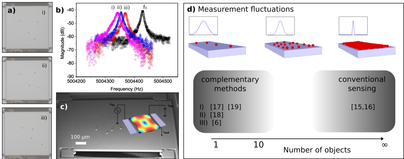
FIG. 1: Effect of the the position-dependent sensitivity of mechanical resonators operating as gravimetric sensors and regimes of operation. a) Images of four polystyrene particles of 10\ \mu\text{m} diameter on a square plate resonator excited in Lamé mode for three cases studied. b) Shows the amplitude response at resonance for each of the three cases presented and f_0 , the resonant frequency without mass loading. c) Scanning electron micrograph showing four PS particles on a square plate resonator and the measurement principle (inset). d) When the number of object is large, the average response resolves the measurement accurately. This assumption is valid for the case of distributed mass using thin film deposition for example (see [15, 16]). When the number of objects is small, the fluctuations become very large and complementary methods are necessary to resolve the measurements. Multimodal approaches (I) have been used to measure single objects [17] and up to 3 beads in [19]. Transfer function methods (II) and physico-chemical methods (III) were used to detect single objects [18] and [6] respectively. However the interpretation of results falling between these two regimes, that represent many cases of practical interest, are not described by current models.
