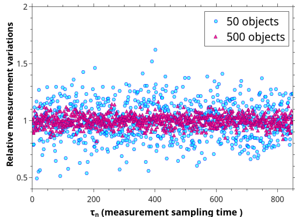
FIG. 4: Results from a discretized version of the Monte Carlo simulations model showing that non-specific interaction (transient binding and dissociation events) on a sensor with heterogeneous gravimetric sensitivity, in this case a cantilever excited in its first flexural mode, can appear as a noisy measurement (the variations decrease with the number of objects).
