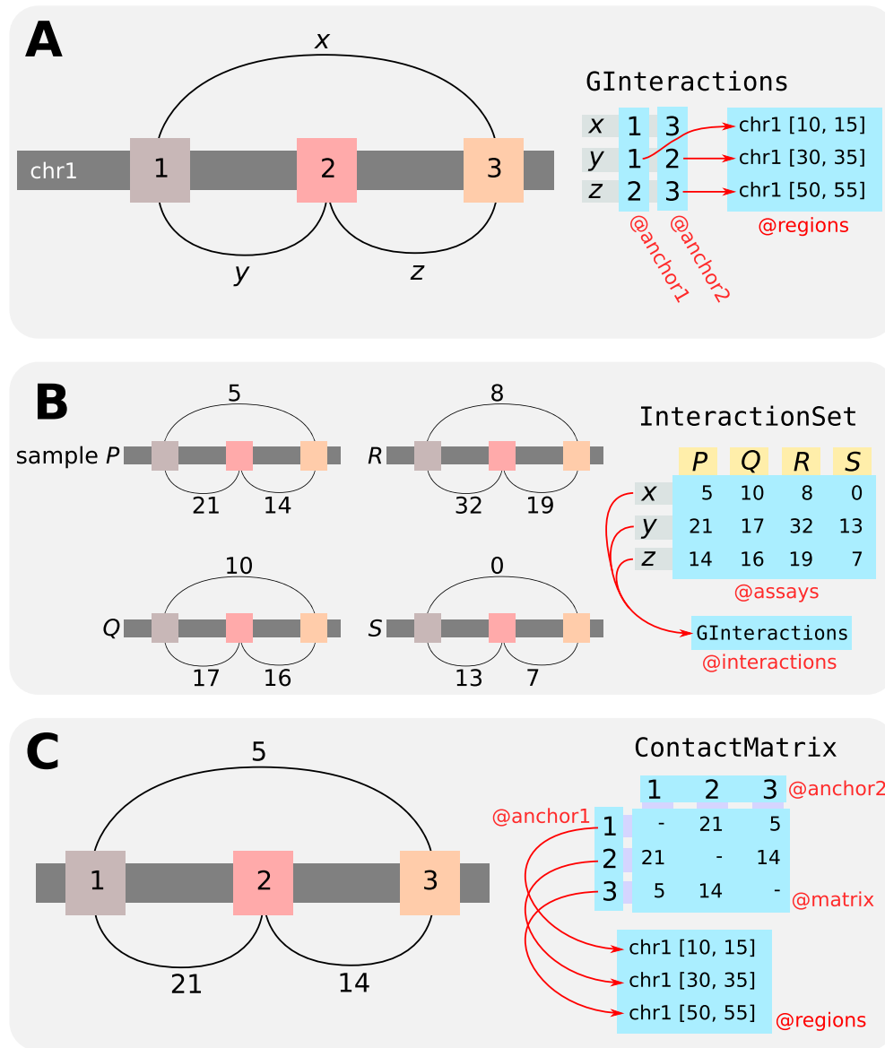
Figure 1. Overview of the classes in the InteractionSet package. Relevant slots of each class (i.e., data values stored in each object of the class) are labelled with a preceding “@”. (A) The GInteractions class represents pairwise interactions between genomic regions by storing pairs of anchor indices that refer to coordinates in a GenomicRanges object. (B) The InteractionSet class stores experimental data in an “assays” matrix where each row is an interaction and each column is a sample. Here, counts represent the number of read pairs mapped between each pair of interacting regions in each sample. (C) The ContactMatrix class represents the interaction space as a matrix, where each cell represents an interaction between the corresponding row/column regions.
