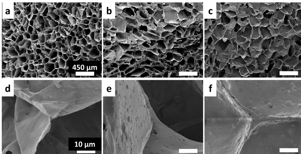
Fig. 3. Representative SEM micrographs of bulk collagen scaffolds (a–c), and triple points between pore walls (d–f) as a function of concentration in the precursor slurry: (a,d) 0.5%, (b,e) 1%, (c,f) 1.5%. While the bulk structure is qualitatively similar for all conditions, the size of the morphological features (pore strut and wall thicknesses) increases with collagen concentration.
