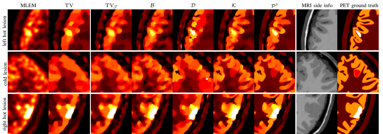
Fig. 4. Close-up of the lesions of the results with “optimal” chosen regularization parameter from figure 3. It can be seen that both \mathcal{K} and \mathcal{P} result in well-defined anatomical boundaries. Moreover, \mathcal{P} shows clearly defined lesions.
