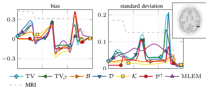
Fig. 8. Line profiles of bias and standard deviation for the software phantom, cf., figure 7. The line segment is marked in the image at the top right and a scaled version of the MRI serves as a reference about anatomical structure. All methods have spatially varying bias and standard deviation. While the methods that reduce to a quadratic prior, i.e., \mathcal{B} and \mathcal{K} , have a relatively flat standard deviation, the standard deviation of the other three methods (which reduce to total variation in the absence of anatomical information) are relatively peaked.
