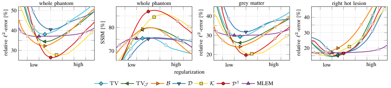
Fig. 2. Quantitative results for the software phantom with the amount of regularization (number of iterations for MLEM) on the horizontal axis. The optimal parameters are chosen based on the relative \ell^2 -error over the whole phantom (far left) and the results for this choice are marked solid in all four plots and shown in figure 3. Also shown (second left) the SSIM (structural similarity index) for the whole phantom. “Too low” and “too high” regularization, cf., figure 3, are marked with lighter shading. \mathcal{K} and \mathcal{P} perform best for the whole phantom and grey matter. Moreover, for this choice of regularization \mathcal{B} and \mathcal{D} perform worse for the right hot lesion than the other methods which all perform similarly. \dagger proposed method
