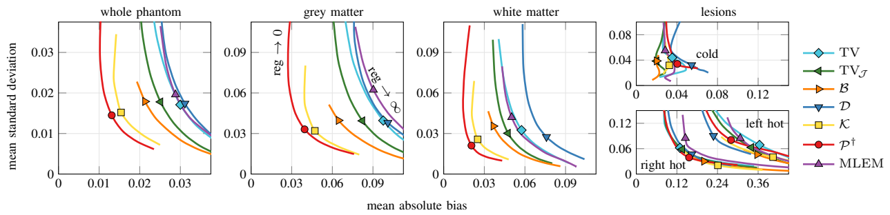
Fig. 6. Mean absolute bias-versus-mean standard deviation trade-off in different regions of interest. \mathcal{K} and \mathcal{P} have the best trade-off for the whole phantom, grey matter and white matter as their curves lie “underneath” the other curves but all methods have similar curves for the lesions (far right). Moreover, the solution that has the smallest expected mean squared error for the whole phantom (distance from the origin in the far left plot) is marked in all four graphs. It can be seen that these solutions have all roughly the same standard deviation for the whole phantom, grey matter and white matter but \mathcal{P} has always the smallest bias. In addition, the “optimal” solution for \mathcal{K} has a larger bias for the hot lesions.
