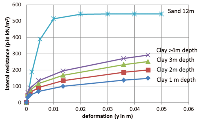
Fig. 22. (Color) p-y curves at different depths for clay and sand for pile diameter of 0.18 m according to API (1984) as used in Bijnagte and Luger (2000) (determined for a 11.5-m-thick saturated clay with c_u = 30 kN/m 2 ; \gamma' = 16 kN/m 3 ; empirical constant J = 0.25 ; and \epsilon_{50} = 0.01 and 0.5 m sand with \varphi' = 30^\circ ; \gamma' = 19.8 kN/m 3 ; K_0 = 0.5 ; factor for static loads A = 0.9 ; initial modulus of subgrade reaction k = 8,145 kN/m 3 ; and q_c = 13.5 MPa)
