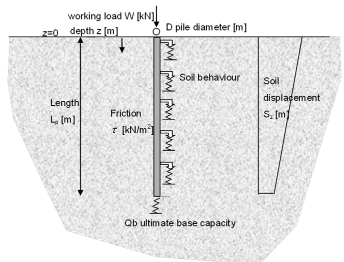
Fig. 3. Model schematization and parameters
