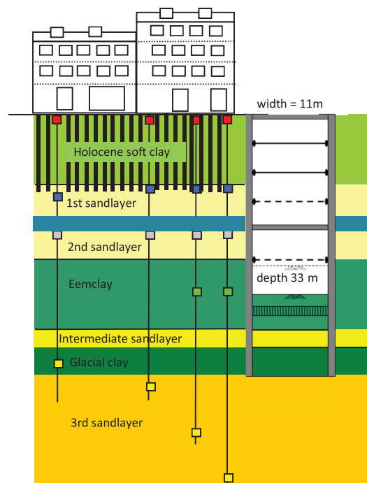
Fig. 12. (Color) Cross section of Ceintuurbaan Station with soil profile and extensometer locations
