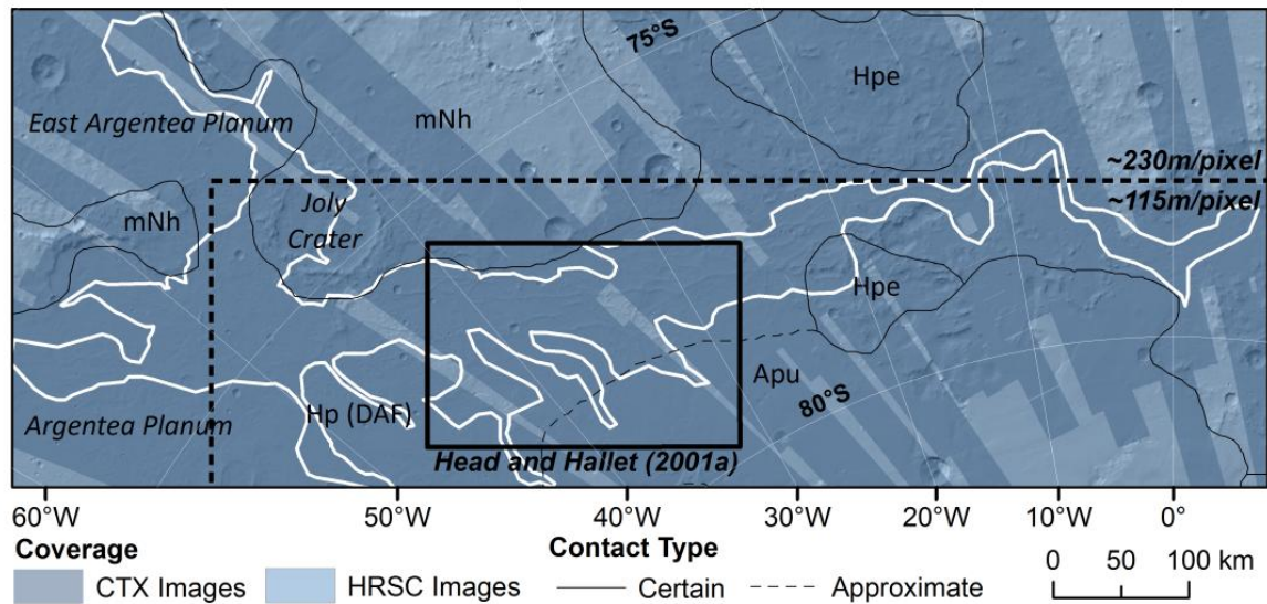
Figure 3: Data coverage map of the study region (extent displayed in Fig. 1) overlain on a hillshade map derived from the ~460 m/pixel MOLA DEM. The extent of the mapped ridges is outlined in white. The dashed line indicates the boundary between ~230m/pixel and ~115m/pixel MOLA DEMs. The solid box indicates the approximate study area of Head and Hallet (2001a). Projection is south polar stereographic. Surface units, labels and contacts are modified from Tanaka et al (2014a).
