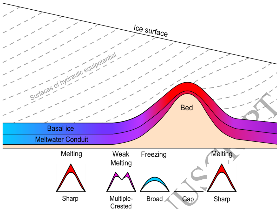
Figure 2: The relationship between esker crest morphology, dimensions and bed topography described by Shreve (1985a), based on Figure 5 from Shreve (1985a) and Figure 8.64 from Anderson and Anderson (2010). Temperature is represented on a gradient from light blue (cold) through to red (warm). Geometries are not accurate and dimensions are exaggerated for clarity. The reader is referred to the web-version of this article for interpretation of the colours in this figure.
