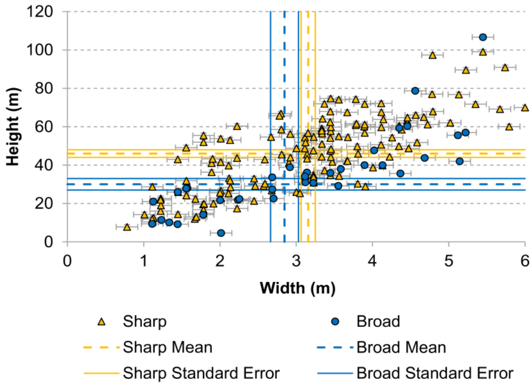
Figure 10: Scatterplot of height, H against width, W , for ridge cross-sectional profiles, classified by crest morphological type. Error bars display uncertainties from Table 2.
