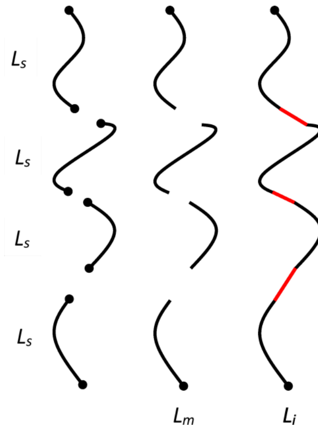
Figure 4: Method for calculation of ridge segment length ( L_s ), mapped length ( L_m ) and system length ( L_i ). Dots indicate the start and termination points of length calculations. Gaps in solid lines between points are not included in length calculations. Straight red lines indicate linear interpolation of length calculation across gaps.
