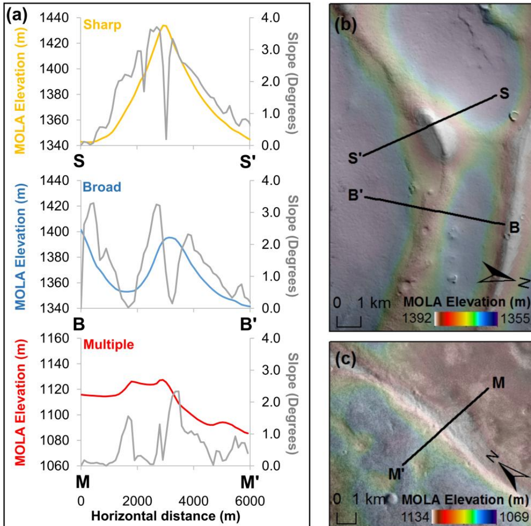
Figure 7: Examples of classification of ridge crest morphological types. (a) Elevation (coloured lines) and slope (grey lines) profiles are displayed for sharp, broad, and multiple-crested crest morphologies. Letters refer to the start and end points of the profiles displayed in (b) and (c) . Scales are equivalent on all three plots and have vertical exaggeration of \sim 46 . Point spacing along profiles is \sim 115 m. (b) A section of Ridge D showing the locations of the sharp-crested and broad-crested cross-sectional profiles in (a) . MOLA \sim 115 m/pixel DEM overlain on CTX image B08_012610_1036_XN_76S018W, image credit: NASA/JPL-Caltech/MSSS. Extent displayed in Fig. 5. (c) A section of Ridge B showing the location of the multiple-crested cross-sectional profile in (a) . MOLA \sim 115 m/pixel DEM overlain on CTX
