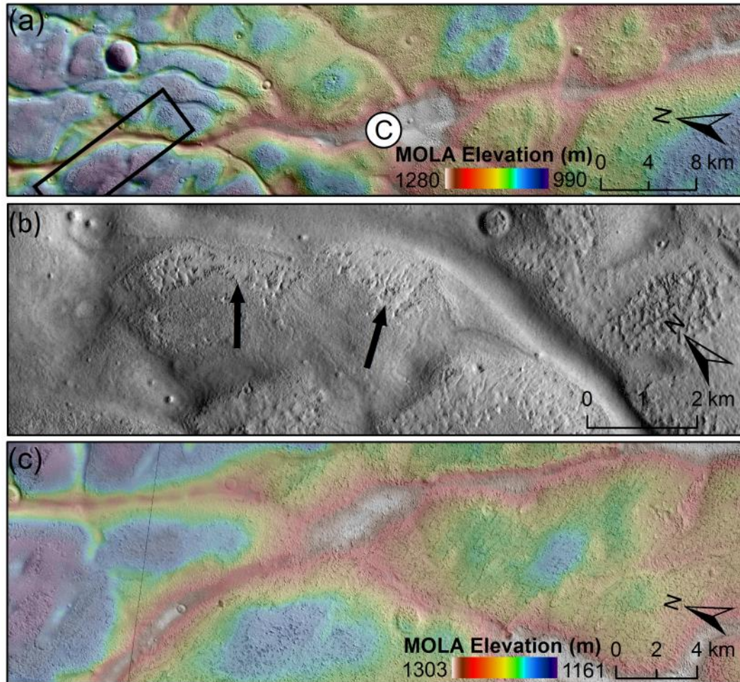
Figure 6: Illustrations of the influence of the textured mantling deposit upon ridges within the study area. The reader is referred to the web-version of this article for interpretation of the colours in this figure. (a) CTX image P13_006282_1046_XN_75S043W overlain with colourised MOLA ~115m/pixel DEM showing emergence of Ridge C from textured mantling deposit in the South East. Black box shows location of (b). Extent shown in Fig. 5 (b) CTX image P13_006282_1046_XN_75S043W of a section of Ridge C close to the contact with the mantling deposit showing remnant accumulations (indicated by black arrows) of the textured deposit adjacent to Ridge C; (c) CTX image P12_005807_1024_XI_77S035W overlain with colourised MOLA ~115 m/pixel DEM showing mantling by the textured deposit
