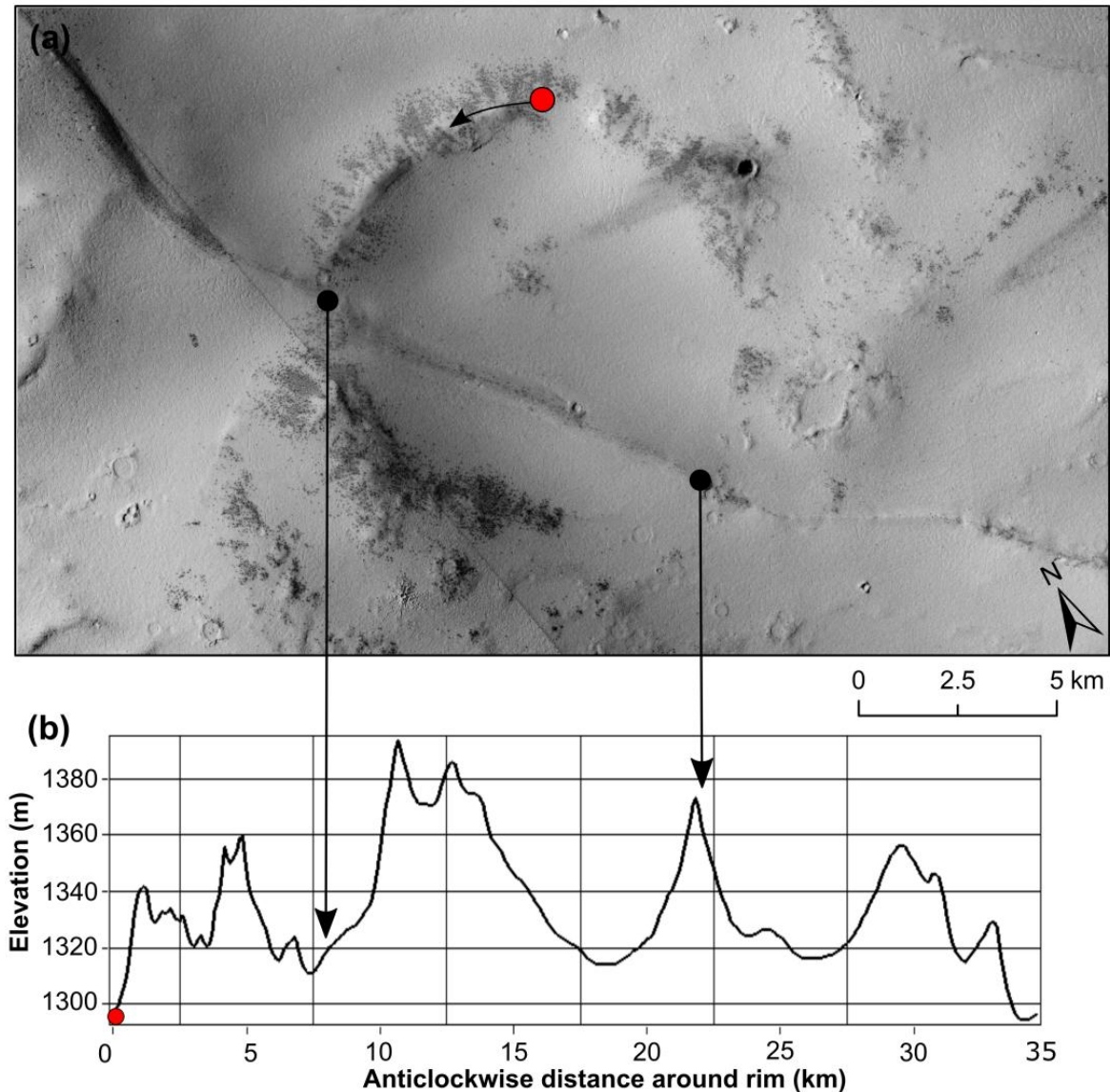
Figure 13 (a) Passage of Ridge A through an infilled crater (CTX images B12_014_285_1025_XN_77S026W and B12_014351_1024_XN_77S028W, image credit: NASA/JPL-Caltech/MSSS). Image extent is displayed in Fig. 5. (b) Topographic profile of the crater rim derived from the \sim 115\text{m/pixel} MOLA DEM, passing anticlockwise from the point marked in (a). Points on the profile that intersect Ridge A are indicated with vertical arrows.
