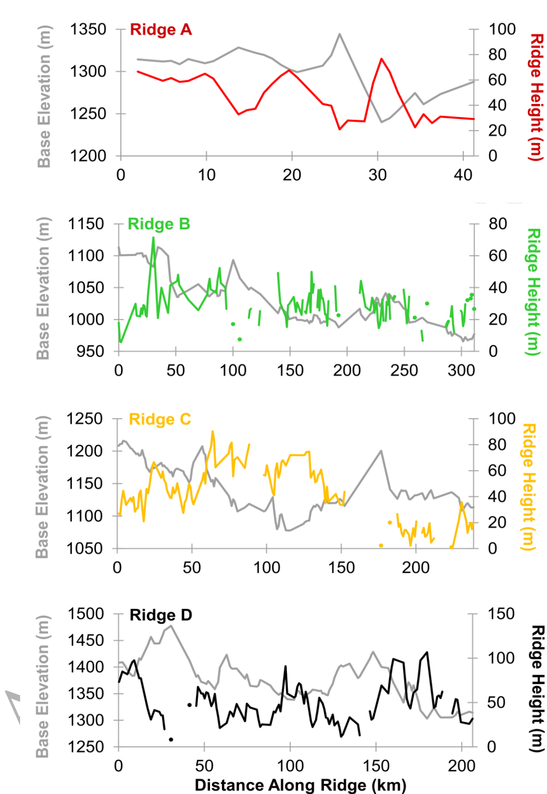
Figure 11: Longitudinal plots of ridge height, H (coloured lines and points) and base elevation, Z_{base} (grey lines) derived from systematically sampled cross-sectional profiles on
