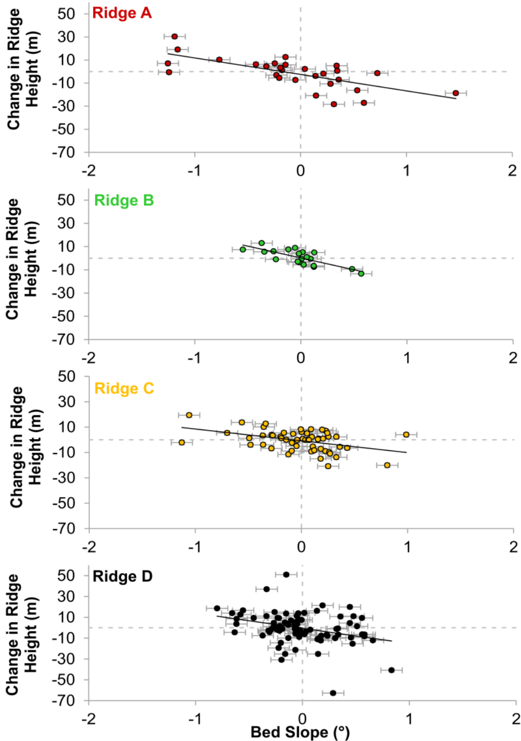
Figure 12: Scatterplots of longitudinal change in ridge height ( dH ) against bed slope ( \theta_L ) for cross-sectional profiles on Ridges A ( n = 28 ), B ( n = 20 ), C ( n = 55 ) and D ( n = 80 ), with linear trend lines. Upper left quadrants represent descending slopes and increasing ridge heights, and lower right quadrants represent ascending slopes and decreasing ridge height. Error bars display uncertainties from Table 2.
