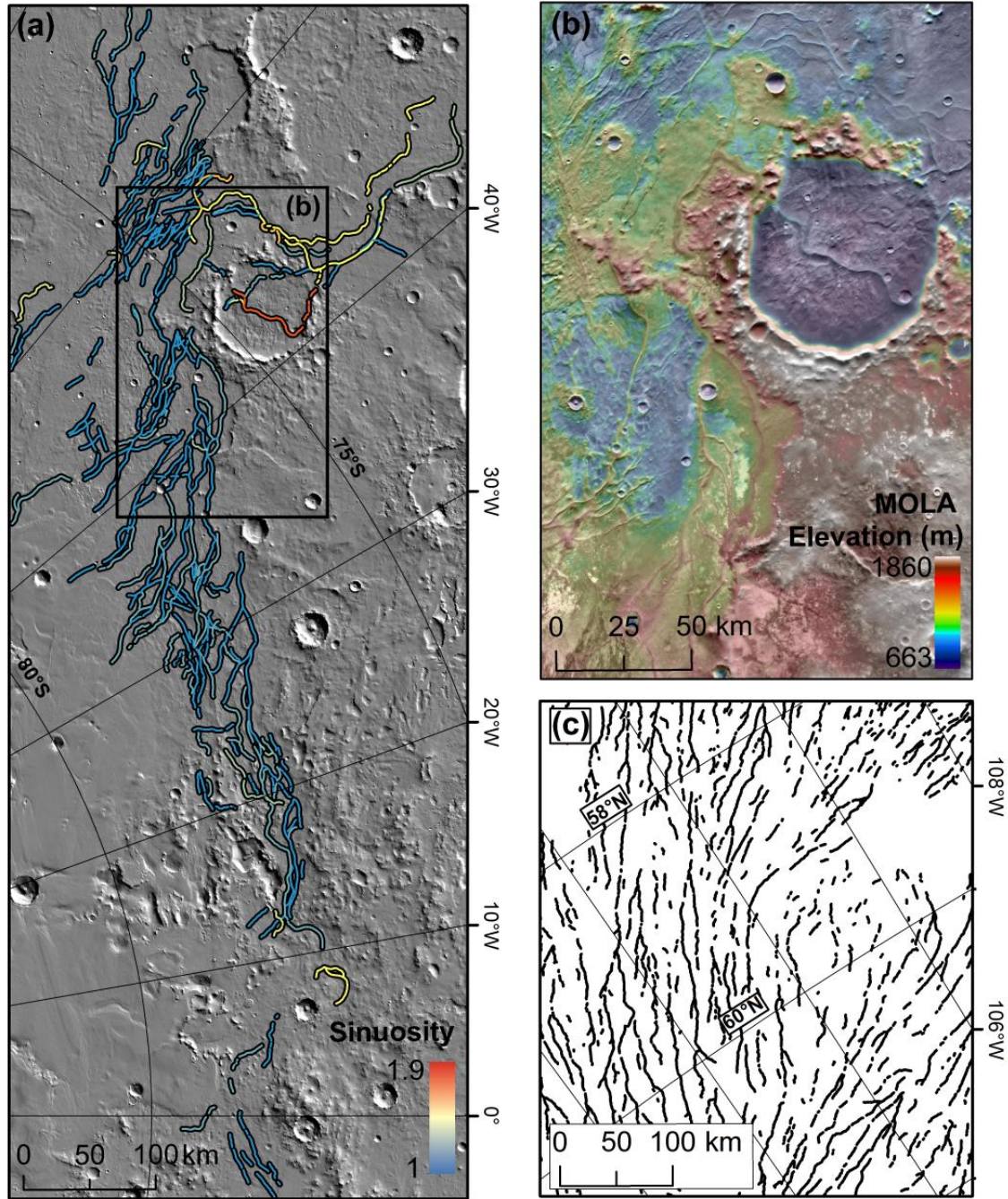
Figure 9: (a) Map of the Dorsa Argentea classified by system sinuosity, S_i , overlain on a hillshade map derived from \sim 115 and \sim 230 m/pixel MOLA DEMs. Map extent is displayed in Fig. 1. (b) \sim 115 and 230 m/pixel MOLA DEM overlain on image from the \sim 100 m/pixel THEMIS Day IR v11 512ppd global mosaic from USGS (image credit: NASA/JPL-Caltech/Arizona State University) showing a region of the Dorsa Argentea. Extent displayed in (a). (c) Map of a region of the terrestrial eskers in Canada mapped by Storrar et al. (2013),
