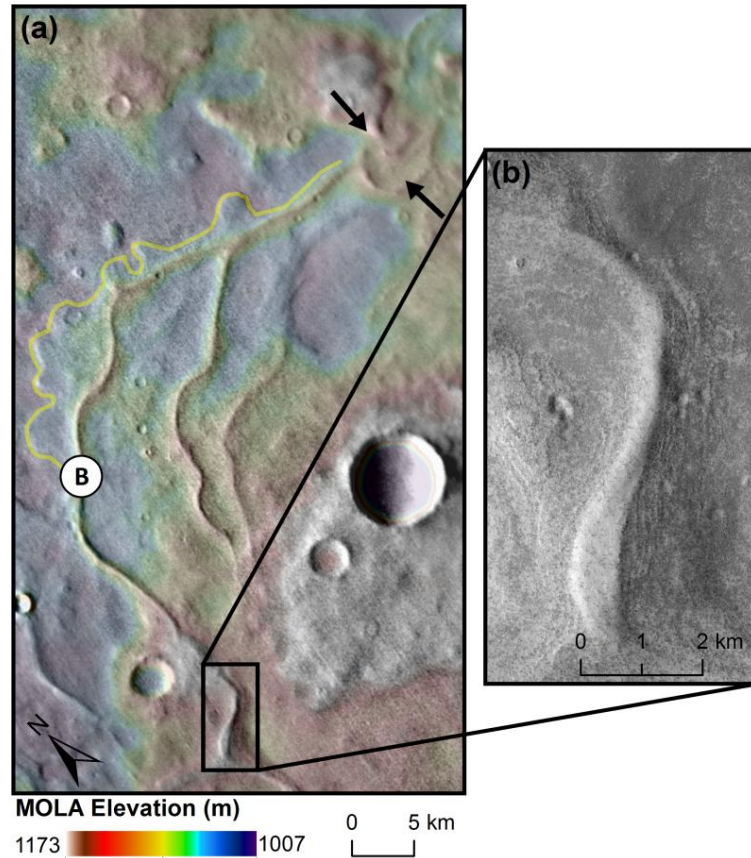
Figure 14: (a) Image from ~100 m/pixel THEMIS Day IR v11 512ppd global mosaic from USGS (image credit: NASA/JPL-Caltech/Arizona State University) of a section of Ridge B (extent displayed in Fig. 5.) showing the lateral pedestal feature (outlined). Black arrows indicate entry of Ridge B into East Argentea Planum. The black box shows the extent of (b). The reader is referred to the web-version of this article for interpretation of the colours in this figure. (b) Evidence of layering structures in the side slopes of Ridge B (CTX image G13_023371_1065_XN_73S048W, image credit: NASA/JPL-Caltech/MSSS).
