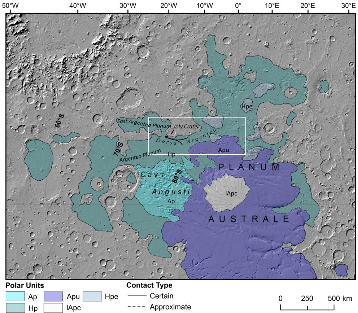
Figure 1: Map of the south polar region of Mars showing the major surface units (Tanaka et al., 2014a) with relevant features labelled, overlain on a hillshade map derived from 460 m/pixel MOLA DEM. The black arrow shows the general trend of the Dorsa Argentea ridges. Ap is the Amazonian polar unit; Apu is the Amazonian polar undivided unit; Hpe is the Hesperian polar edifice unit; Hp is the Hesperian polar unit, equivalent to the Dorsa Argentea Formation (DAF); and IApc is the Late Amazonian polar cap unit. The white box delineates our study area. Projection is south polar stereographic. Surface units, labels and contacts between them are modified from Tanaka et al. (2014a).
