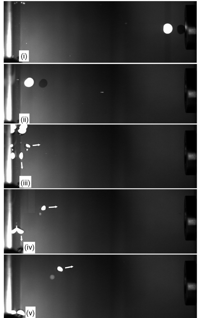
Fig. 10. Series of video stills for projection of a Hekla pellet, with an initial temperature of 1200 °C, corresponding to times of (i) 1.39 ms, (ii) 2.46 ms, (iii) 3.21 ms, (iv) 4.07 ms and (v) 5.03 ms.
