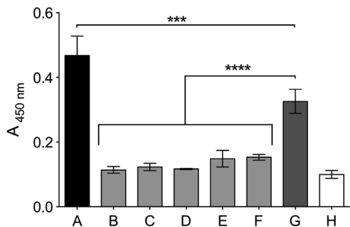
Fig. 3. THP affinity for the \alpha_2 I-domain. The recombinant \alpha_2 I-domain-GST-fusion protein was incubated at 0.5 \mu\text{g}/\text{ml} with THP at 100 \mu\text{g}/\text{ml} for 30 min in the presence of \text{Mg}^{2+} , with: no peptide (A); GPC(GPP) 5 GFOGER(GPP) 5 GPC (B); (GPP) 5 GFOGER(GPP) 5 (C); ES-GFOGER (D); Diazirine-ES-GFOGER (E); Diazirine-ES-GFOGER-Biotin (F); or GPP10 (G). The adhesion of the \alpha_2 I-domain to immobilized GPC(GPP) 5 GFOGER(GPP) 5 GPC after 1 h was assessed using anti-GST antibody. Control wells were coated with BSA incubated with the \alpha_2 I-domain (H).
