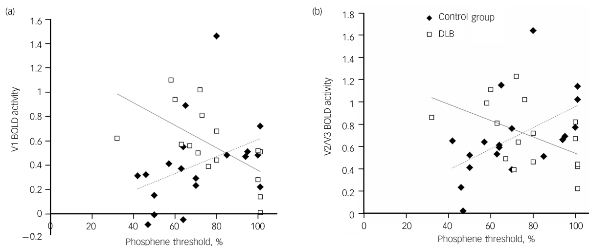
Fig. DS1 Scatter plots showing phosphene threshold plotted against V1 blood oxygen level-dependent (BOLD) activity (a) and V2/V3 BOLD activity (b) in response to checkerboard stimulation in dementia with Lewy body (DLB, n = 16) and control ( n = 19) groups.
