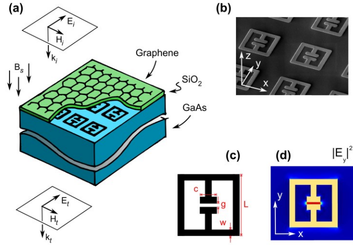
FIG. 1. (a) Schematic of the sample and of the experimental arrangement. An array of split-ring resonators (SRR) is patterned on the surface of a gallium arsenide substrate. A graphene monolayer is transferred on the surface, and isolated by a silicon oxide layer from the SRR. (b) Scanning electron micrography of the gold SRR. (c) Geometrical parameters of the SRR. (d) Resonant field excited in the gap of the SRR.
