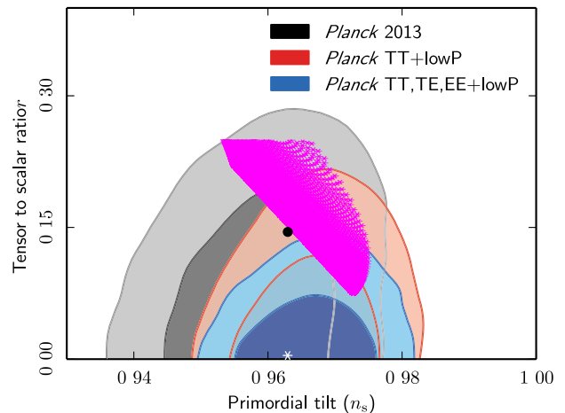
FIG. 1: The n_s - r diagram for the hyperbolic potential of [19] using N = 55 . The contours borrowed from Planck 2015 [4]. The area which is plotted over the contours corresponds to the hyperbolic Rubano & Barrow [20] potential (see Eq.(11)). The points correspond to chaotic (solid point) and Starobinsky (star) inflation respectively.
