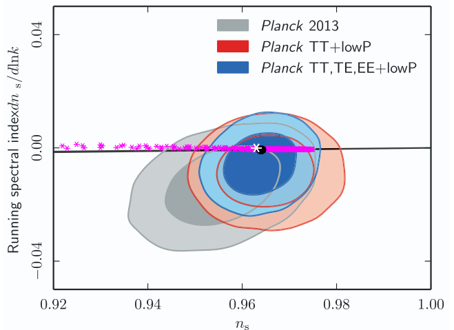
FIG. 2: The n_s - n'_s diagram. The area corresponds to the hyperbolic Rubano & Barrow [20] potential (for more details see the caption of figure 1).
