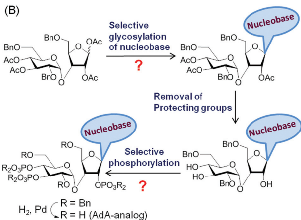
Fig. 1 (A) Molecular structures of IP 3 (1) and AdA (2); (B) conventional synthesis of AdA-analogs. The question marks represent the complexity of conventional syntheses.
