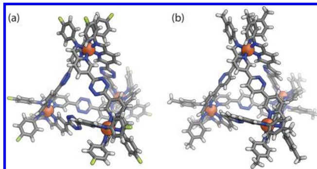
Figure 2. Depictions of the X-ray crystal structures of (a) tetrazine-edged cage 1a , and (b) pyridazine-edged cage 2e . Key: light green = fluorine; orange = iron; blue = nitrogen. Disorder and anions have been omitted for clarity.
