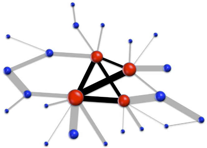
Figure 1 | Weighted rich clubs are measured in terms of the weighted connectedness between rich nodes. The rich club is the set of red (color online) nodes with a richness value above a certain threshold \bar{r} . In this example, the richness parameter is degree and \bar{r} = 3 . Size of nodes is proportional to their richness. The rich club is thus the subgraph formed by nodes with degree larger than 3. The weighted connectedness, C , of the rich club is the sum of the weights of the links between the nodes in the subgraph (black lines). The rich-club coefficient \phi is calculated by dividing the existing weighted connectedness C by the maximal possible weighted connectedness, F . See Eq. 3 and Figure 2.
