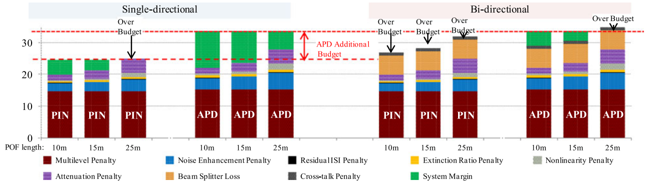
Fig. 5. Simulation results of power budget analysis.
