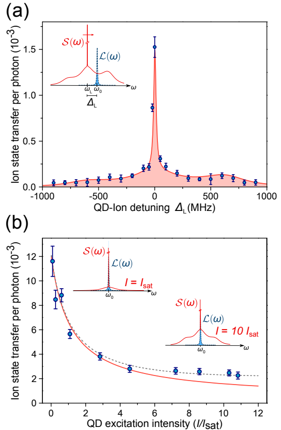
FIG. 3. (Color online) Efficiency of ion state transfer as a function of the QD-ion detuning and QD driving intensity. (a) Spectral dependency of the absorption probability per received photon. The solid line displays the numerical model. The slight asymmetry is due to the detuning of the QD transition from the excitation laser frequency \omega_L induced by finite nuclear spin polarization, and the presence of fast dephasing at high excitation powers, characteristic for this sample [29]. (b) Absorption probability of the ion per received photon as a function of the QD excitation intensity. Insets show the QD photon spectrum S(\omega) at two different excitation intensities and the ion absorption line \mathcal{L}(\omega) . The convolution of the two, normalized by the number of QD photons, gives rise to the solid line. Including the imperfect suppression of the excitation laser (ratio of QD to laser photons is 70 : 1 at I_{\text{sat}} ) in the numerical modeling predicts the dashed line. The error bars are statistical errors. We note that the ion-cavity coupling rate for the results in panel (b) is slightly higher than that for the measurements in panel (a).
