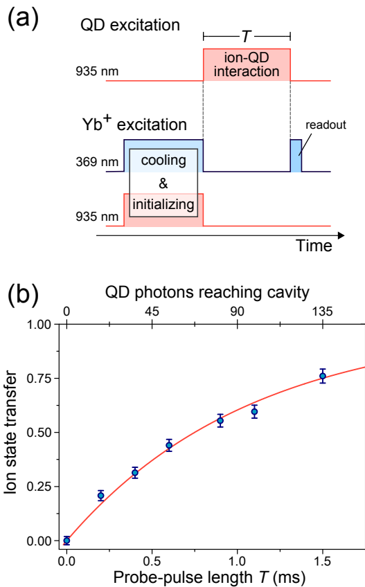
FIG. 2. (Color online) Optical pumping of the ion by QD photons. (a) The ion is prepared in the |-3/2\rangle state of the ^2D_{3/2} manifold by optical pumping at 369 nm and 935 nm simultaneously. Subsequently, the QD is excited for a time T and the generated photons are sent to the ion. The protocol cycle ends with the optical readout of the ion state. (b) Probability of the ion to absorb a QD photon during T in the weak excitation regime ( I=0.5I_{\text{sat}} ). The solid line is an exponential fit with a time constant \tau = 1.1 ms. The top axis indicates the mean photon number for a given T reaching the ion cavity and has 10% statistical error.
