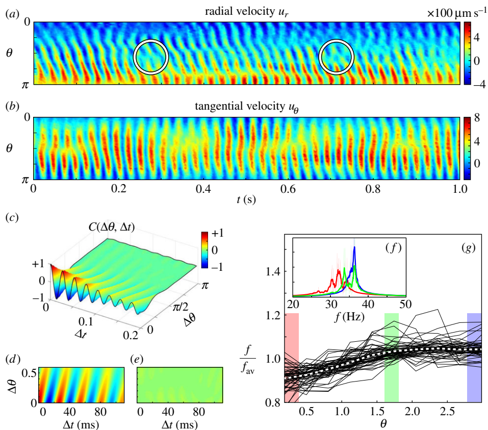
Figure 2. Properties of metachronal waves. (a) Radial u_r(r^*, \theta, t) and (b) tangential u_\theta(r^*, \theta, t) components of the flow field, measured at r^* = 1.3 R . Phase defects are evidenced by white circles. (c) Correlation function C(\Delta\theta, \Delta t) for a single representative Volvox colony, (d) its fitted correlation function C^{\text{fit}}(\Delta\theta, \Delta t) = e^{-\Delta t/\tau} e^{-\Delta\theta/L} \cos(k\Delta\theta - \omega\Delta t) and the (e) corresponding error. The scale bar for (c–e) is the same. (f) Power spectrum of the autocorrelation function C(0, \Delta t) (for one Volvox colony), calculated for three distinct values of \theta . (g) Average beat frequency as a function of polar angle \theta for n = 60 different colonies (black) as well as the ensemble average (white dotted).
