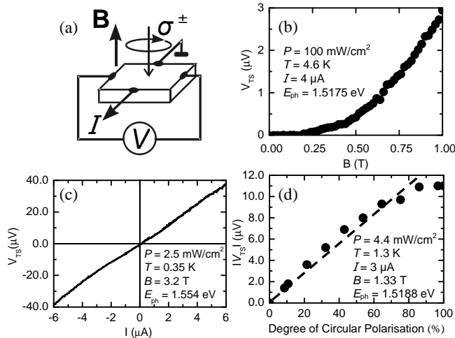
FIG. 1. (a) The experimental arrangement. (b) Magnetic field dependence of V_{\text{TS}} at low magnetic field for the symmetric QW. (c) The DC current dependence of V_{\text{TS}} for the asymmetric QW. (d) |V_{\text{TS}}| versus laser helicity for the symmetric QW. The dashed line is a guide for the eye.
