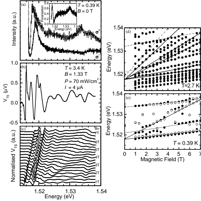
FIG. 2. (a) Zero-magnetic-field right ( \sigma^+ ) and left ( \sigma^- ) circularly polarised PLE spectra for the symmetric QW. Inset: Circular polarisation of that PLE. (b) Photon energy dependence of V_{TS} for the same symmetric QW. (c) Photon energy dependence of that V_{TS} at various magnetic fields. (d) Magnetic field dependence of those V_{TS} peak energies. (e) Magnetic field dependence of \sigma^+ (solid circles) and \sigma^- (open circles) PLE peak energies for the same symmetric QW. The lines are guides for the eye and are explained in the text.
