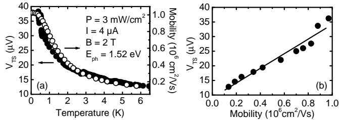
FIG. 3. (a) V_{\text{TS}} (filled circles) and 2D hole gas mobility [16] (open circles) for the same symmetric QW as a function of temperature. (b) V_{\text{TS}} versus mobility. The line is a guide for the eye.
