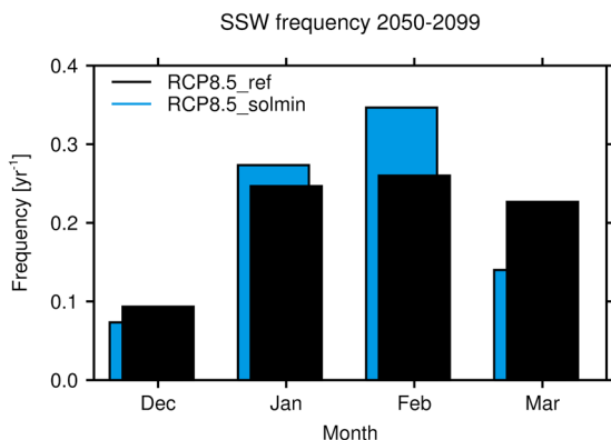
Figure 6. The wintertime distribution of Arctic stratospheric sudden warming events ( \text{year}^{-1} ) in the RCP8.5_ref (black) and RCP8.5_solmin (blue) experiments for the period 2050–2099.
