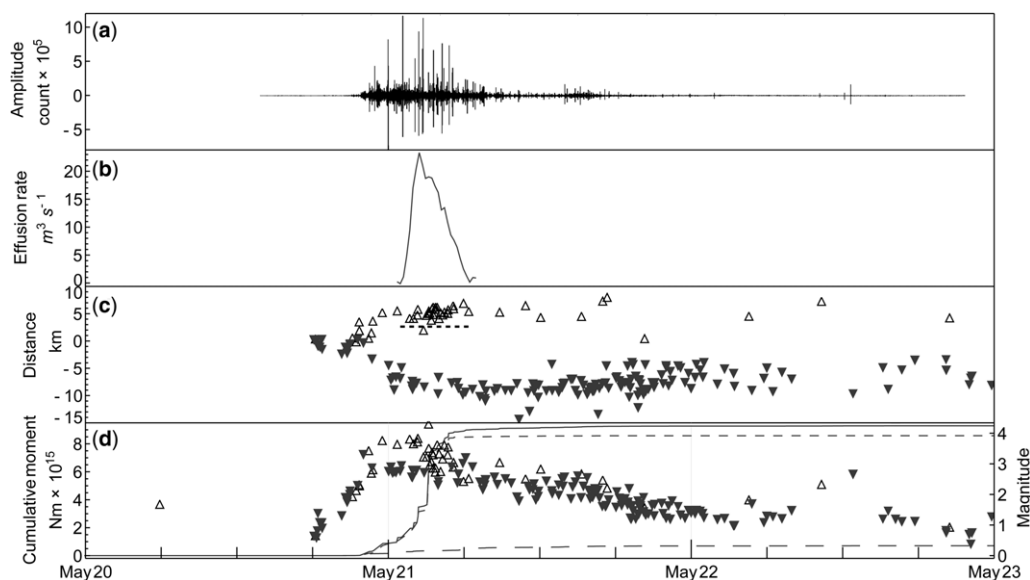
Fig. 5. The timing of seismic events and lava effusion. (a) Vertical component seismic trace for station IGRÉ (see Fig. 1a). (b) Effusion rate calculated from extracted SEVIRI band 3 ( 1.6 \mu\text{m} ) radiance. (c) Migration of seismicity along dyke by distance from centre. Open triangles are northern segment earthquakes, filled triangles southern segment earthquakes and dashed line shows location and duration of the eruption. All earthquakes within 3 km of the dyke are plotted. (d) Earthquake magnitudes and cumulative moment for all events within 3 km of the dyke model. Open triangles are earthquakes in the northern dyke segment, filled triangles are earthquakes in the southern dyke segment, short dashed line shows cumulative seismic moment for northern dyke, long dashed line is for southern dyke and the continuous line gives the total.
