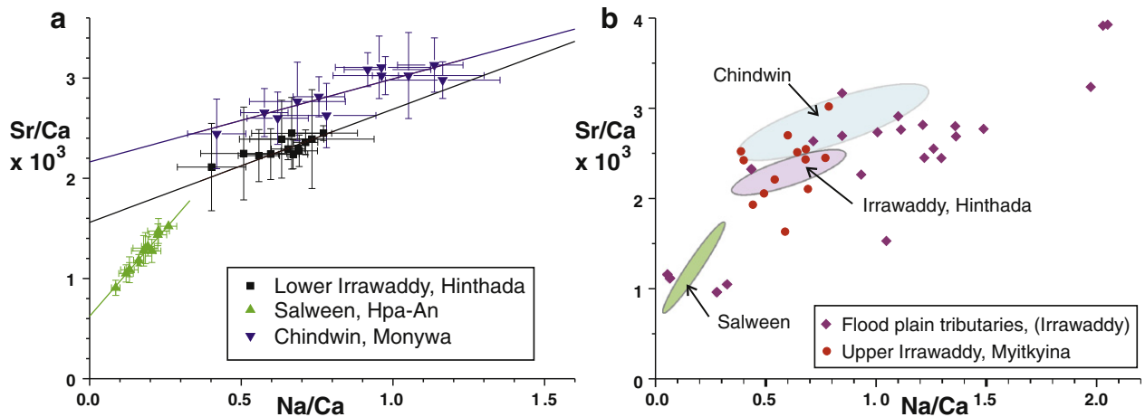
Fig. 8. a. Sr/Ca versus Na/Ca ratios for cyclic-corrected mean monthly samples from Lower Irrawaddy at Hinthada, Salween at Hpa-An and Chindwin at Monywa. Lines are least squares best fits to arrays. b. Sr/Ca versus Na/Ca ratios for Irrawaddy floodplain tributaries compared to fields for Lower Irrawaddy at Hinthada, Salween at Hpa-An and Chindwin at Monywa.
