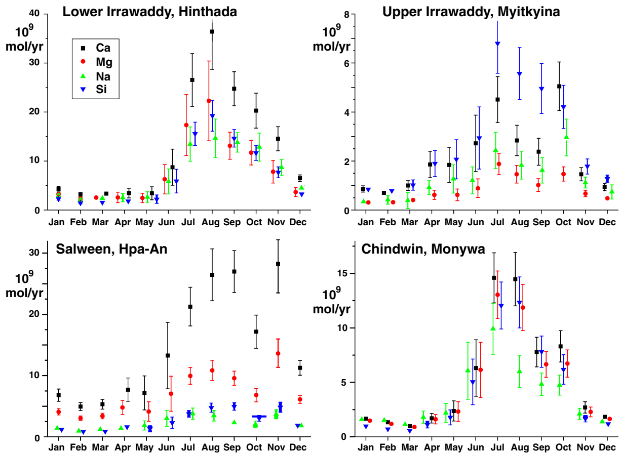
Fig. 10. Ca, Mg, Na and Si monthly fluxes in the Irrawaddy at Hinthada, Irrawaddy at Myitkyina, Salween at Hpa-An and the Chindwin at Monya. Error bars are the combined uncertainty from 1 standard error on the concentration mean of samples included in the monthly average or estimated from the mean error from months with more than two samples (see text and Eq. 1) and the uncertainty in the monthly discharge fluxes as discussed in the text.
