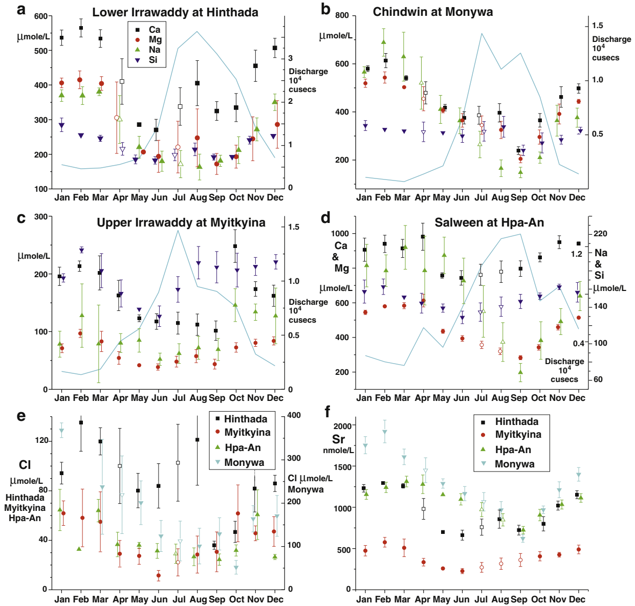
Fig. 4. a, b, c & d. Average monthly Ca, Mg, Na, Si concentrations, corrected for cyclic inputs, at Hinthaada (Lower Irrawaddy), Monywa (Chindwin), Myitkyina (Upper Irrawaddy) and Hpa-An (Salween). e & f. Monthly Cl and Sr concentrations at time series sample sites. Error bars 1 \times standard errors (see text) but not shown where smaller than symbols. Open symbols are months with no samples and the values shown are interpolated between adjacent sampled months and are used in calculating annual fluxes. Blue line in a is average monthly discharge at Pyaw from Robinson et al. (2007) in cusecs and blue line in b, c & d are monthly discharge from 2004 data. Note discharge values for winter months in Salween interpolated as discussed in text.
