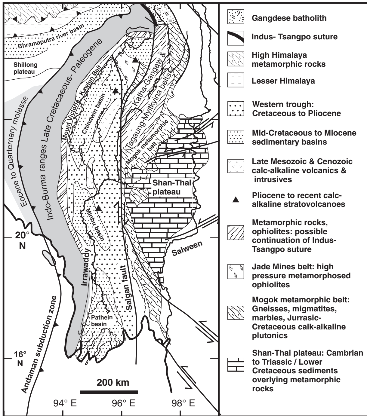
Fig. 3. Geology of Myanmar redrawn from Mitchell et al. (2007) and Searle et al. (2007).
