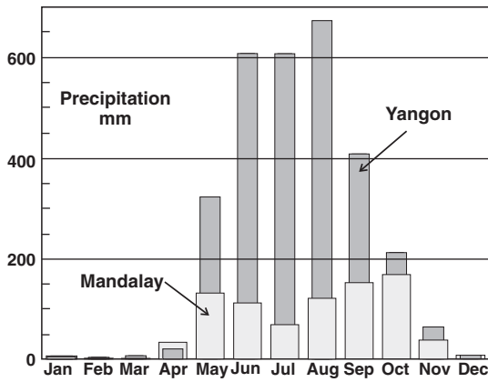
Fig. 5. Average monthly precipitation at Yangon & Mandalay after New et al. (2002).
