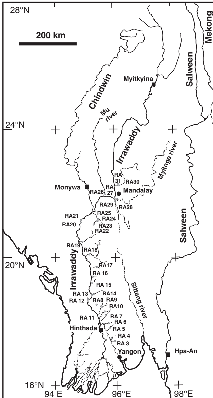
Fig. 2. Map of rivers in Myanmar and sample sites. Drawn from Army Map Service (GDVLB) (1955) 1:250,000 sheets. Solid squares denote the four time-series sample sites. Small grey circles denote tributaries sampled in summer 2007.
