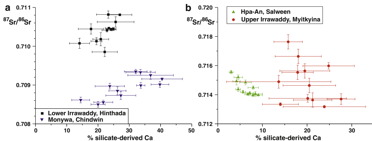
Fig. 11. (a) ^{87}\text{Sr}/^{86}\text{Sr} ratios versus percentage of silicate-derived Ca from the Irrawaddy at Hinthada, and Chindwin at Monywa and (b) the Salween at Hpa-An, and Irrawaddy at Myitkyina. Percentage of silicate-derived Ca is calculated by assuming a silicate Na/Ca ratio of 0.35 where Na is that corrected for rain and evaporate inputs as discussed in text. Poor positive correlations for Irrawaddy at Hinthada, and Chindwin at Monywa probably reflect an increased proportion of silicate dissolution in the dry season. Scatter exhibited by the Irrawaddy at Myitkyina and the good negative correlation exhibited by the Salween at Hpa-An probably reflect increased inputs of higher ^{87}\text{Sr}/^{86}\text{Sr} ratio carbonates from the metamorphic rocks to the east and north during the monsoon.
