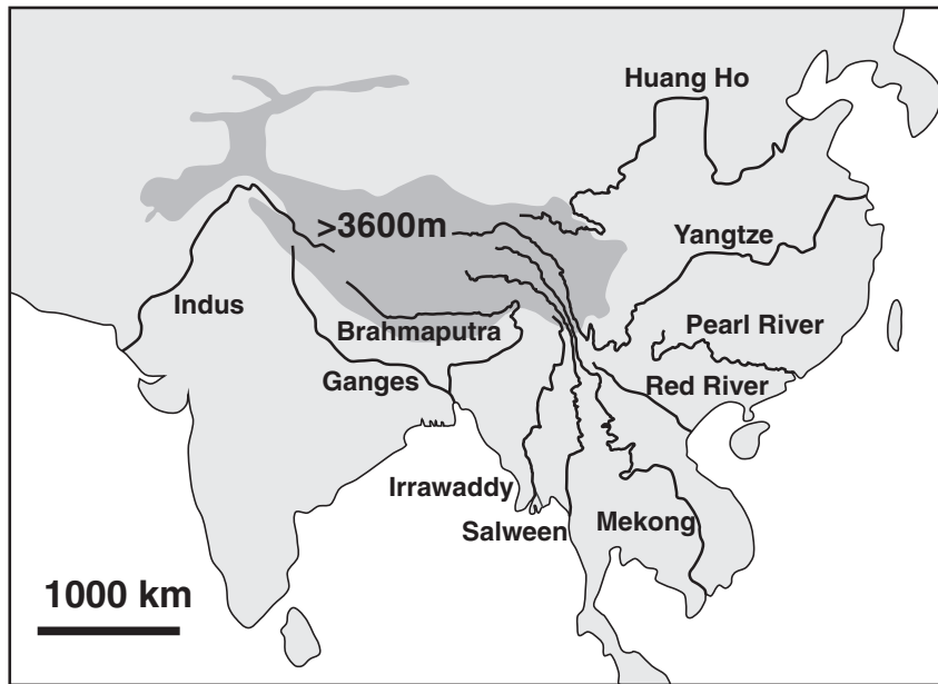
Fig. 1. Major rivers draining the Himalayan-Tibetan region in Asia. Redrawn after Bickle (1996) and Clark et al. (2004).
