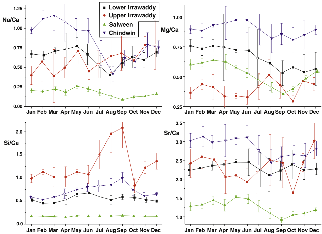
Fig. 7. Mean monthly Na/Ca, Mg/Ca, Si/Ca and Sr/Ca ratios (corrected for cyclic inputs) at four time-series sample sites. Error bars 1 \times standard errors on mean values. Open symbols are months with no samples and values are interpolated between adjacent sampled months.
