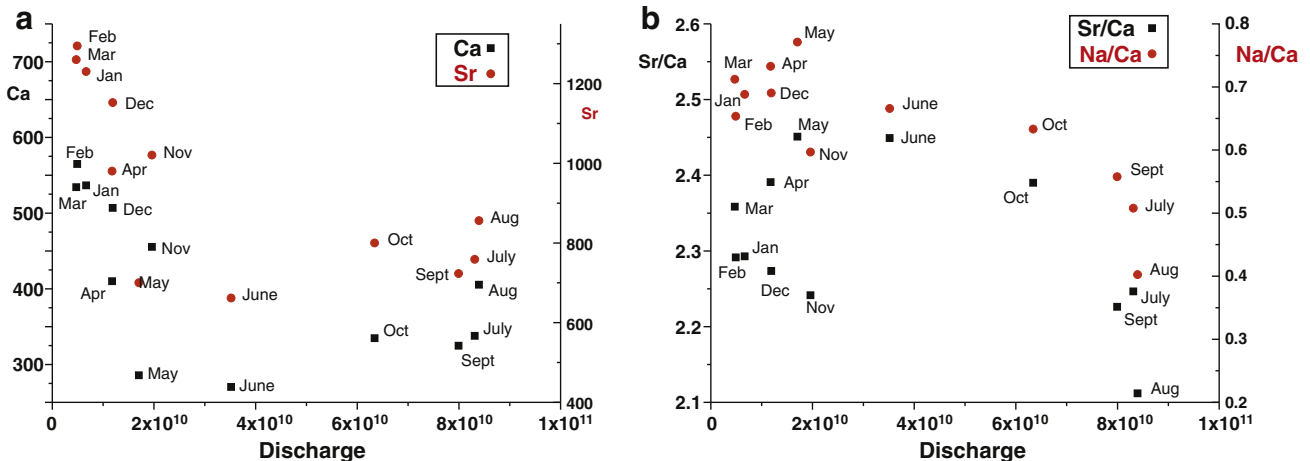
Fig. 6. Mean monthly Ca and Sr concentrations (a) and mean monthly 1000 \times \text{Sr/Ca} and Na/Ca ratios (b), corrected for cyclic inputs, at Hinthada (Lower Irrawaddy) plotted against the mean monthly discharge ( \text{m}^3/\text{month} ) at Pyay from Robinson et al. (2007).
