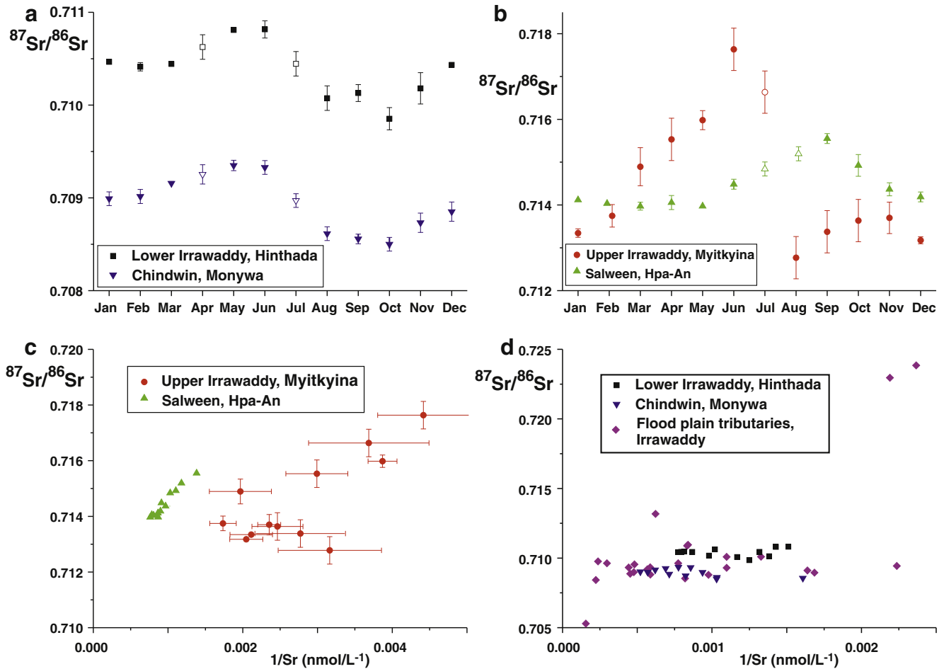
Fig. 9. (a) and (b) show variation of mean monthly ^{87}\text{Sr}/^{86}\text{Sr} ratios from Irrawaddy at Hinthada, Salween at Hpa-An, Chindwin at Monya and Irrawaddy at Myitkyina. Note that the Salween at Hpa-An and Irrawaddy at Myitkyina have higher ^{87}\text{Sr}/^{86}\text{Sr} ratios reflecting inputs from the older basement to the east and the Himalayan ranges. (c) and (d) show mean monthly ^{87}\text{Sr}/^{86}\text{Sr} ratios versus 1/\text{Sr} for Irrawaddy at Myitkyina and Salween at Hpa-An, Irrawaddy at Hinthada, Chindwin at Monya and floodplain tributaries. Error bars 1 \times standard errors (see text) but not shown where smaller than symbols. The positive correlations exhibited by the Salween at Hpa-An and Irrawaddy at Myitkyina probably reflect dilution of Sr concentrations in the monsoon coupled with a greater input from more northerly, more radiogenic, catchments. The two high ^{87}\text{Sr}/^{86}\text{Sr} ratio samples are from flooded fields and the adjacent Chaungmagyi River which drains the Mogok metamorphic rocks.
