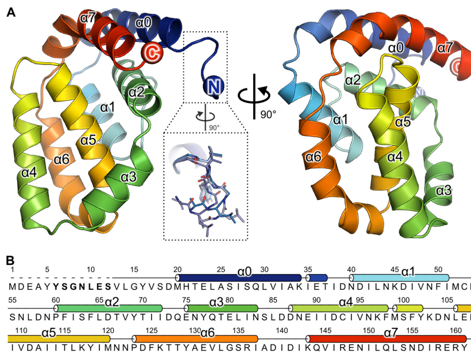
FIGURE 1. A49 adopts a Bcl-2-like fold. A , the structure of A49 \Delta 12 is shown in two orthogonal views as a ribbon colored from blue (N terminus) to red (C terminus). The inset shows the alternative conformations of residues 13–17 observed, highlighting the mobility of this region. In crystals of A49 grown from full-length protein, no density was observed for these residues. B , sequence of VACV WR A49. The secondary structure is shown above the sequence, and residues thought to interact with the \beta -propeller domain of \beta -TrCP are in boldface type.
